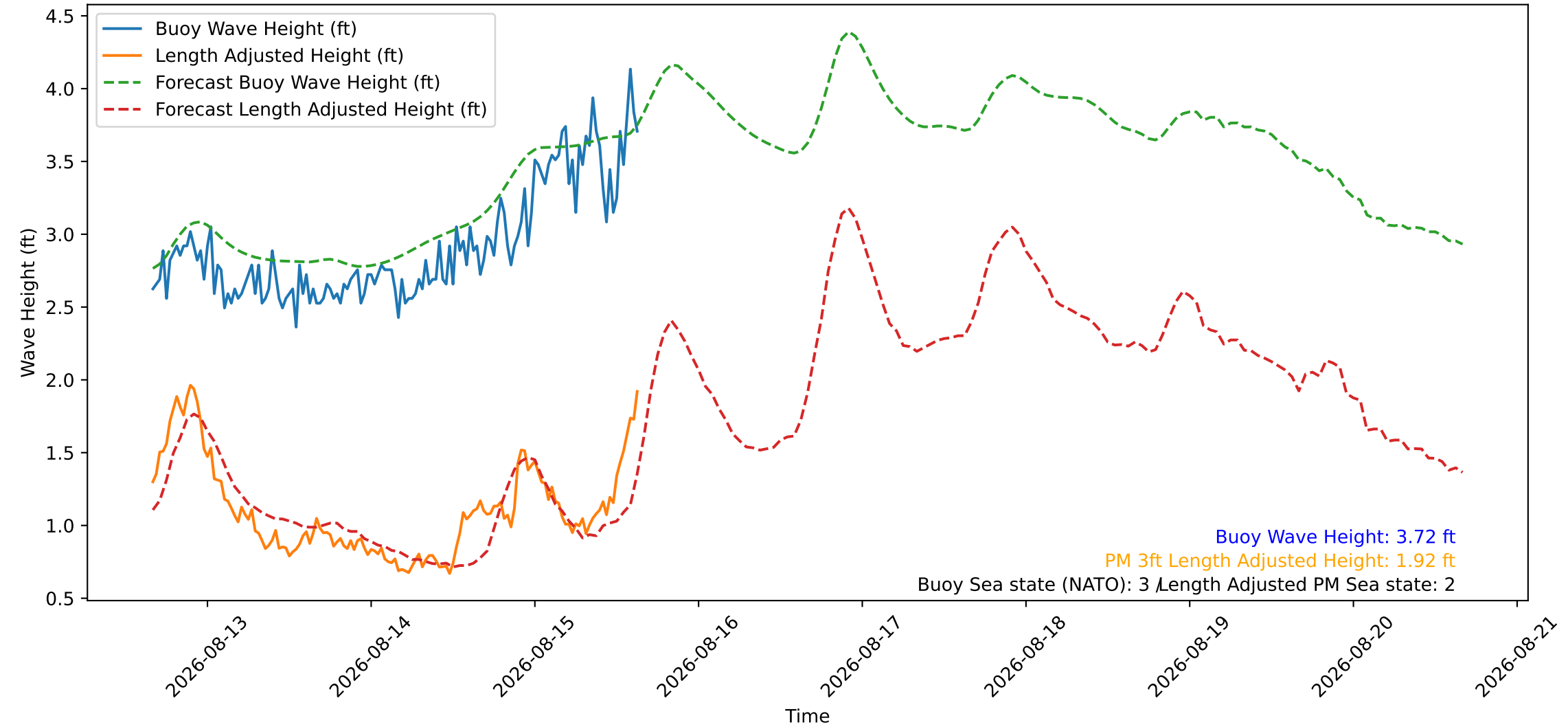
Wave Heights over Time for Green Beach at 2026-08-15 16:01:08
