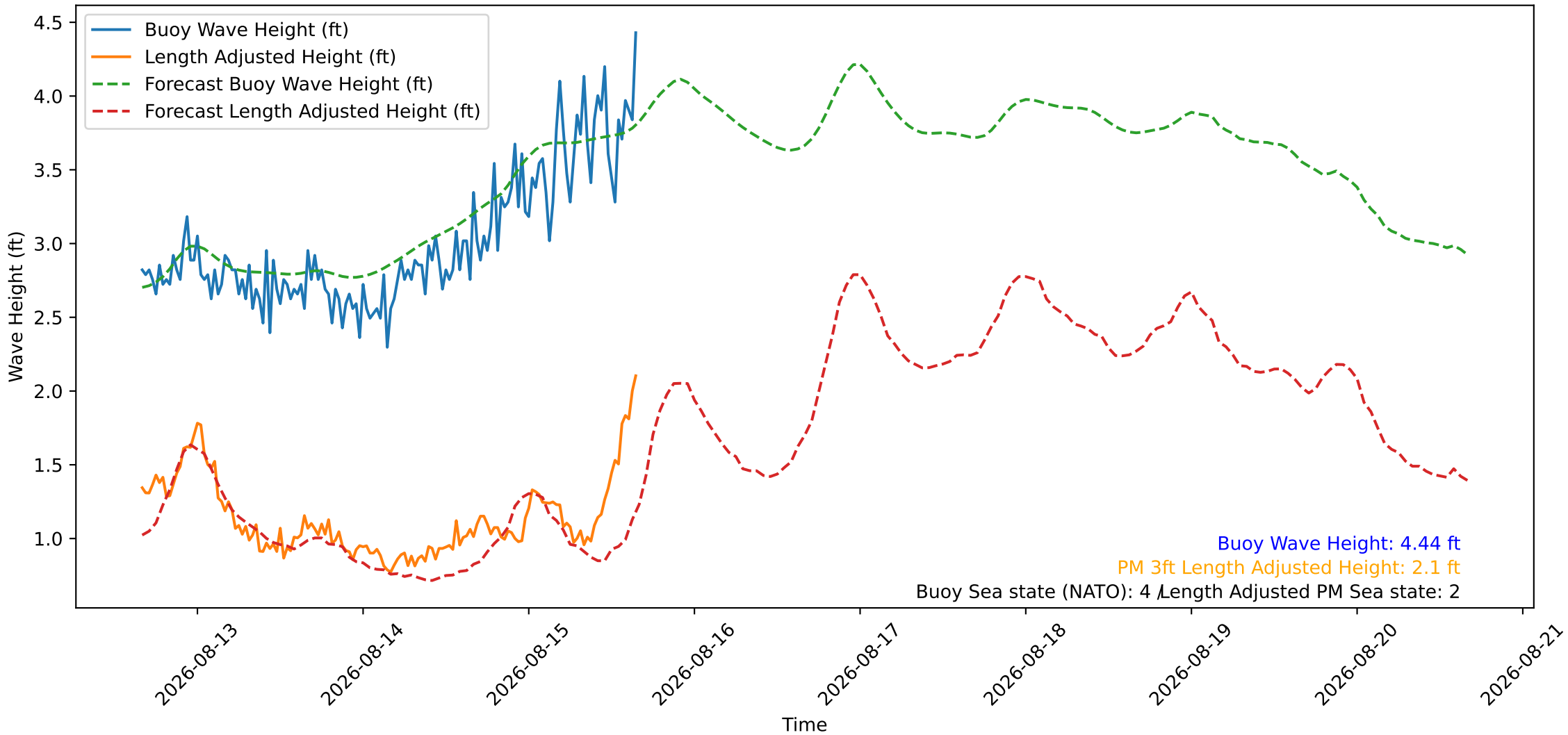
Wave Heights over Time for Oceanside Harbor at 2026-08-15 16:00:27
