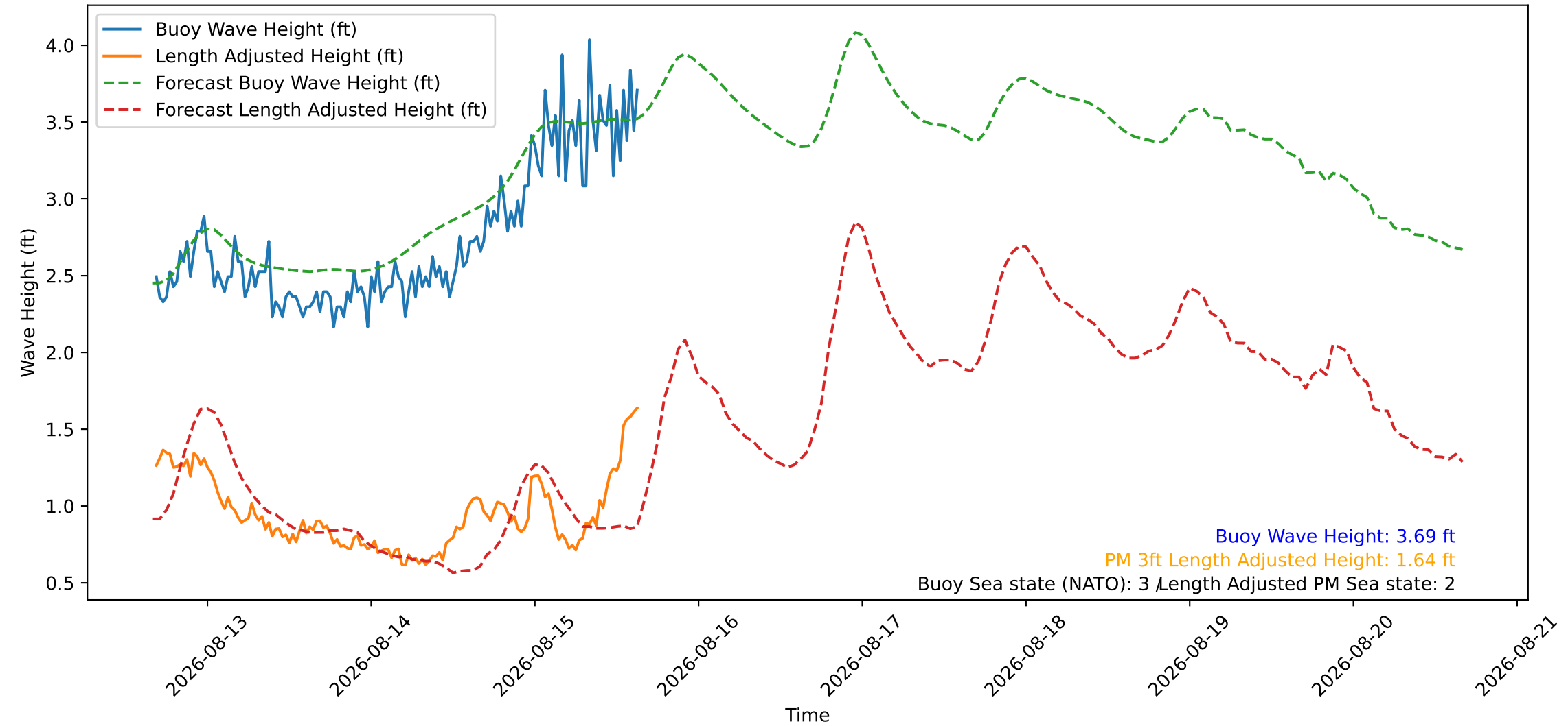
Wave Heights over Time for Red Beach at 2026-08-15 16:00:46
