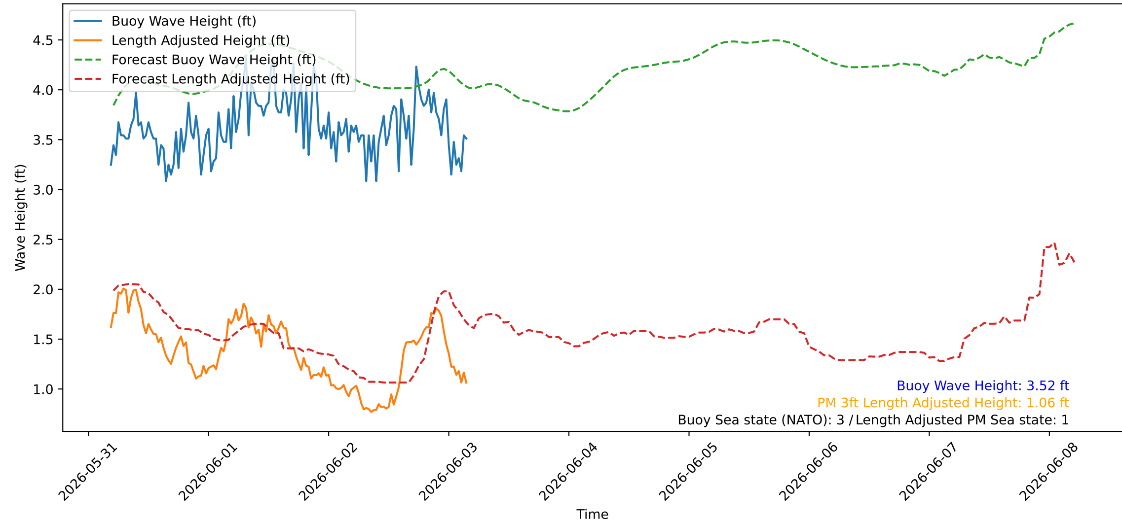
Wave Heights over Time for Green Beach at 2026-06-03 04:31:08
