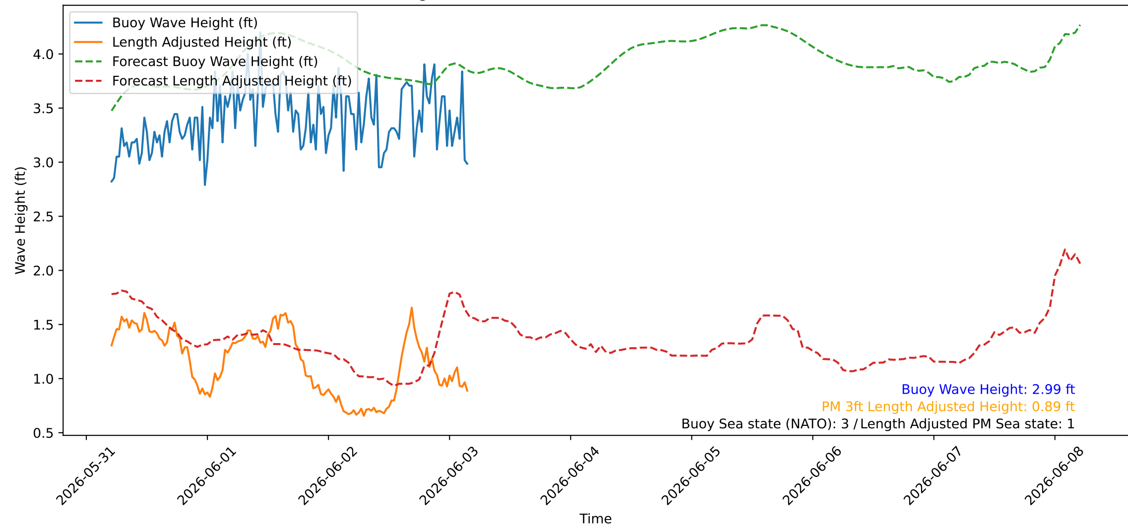
Wave Heights over Time for Red Beach at 2026-06-03 04:30:45
