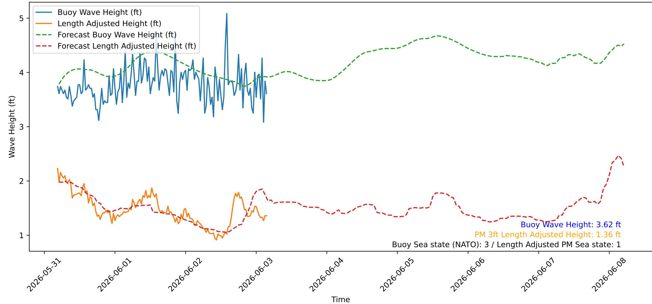
Wave Heights over Time for Oceanside Harbor at 2026-06-03 04:30:26
