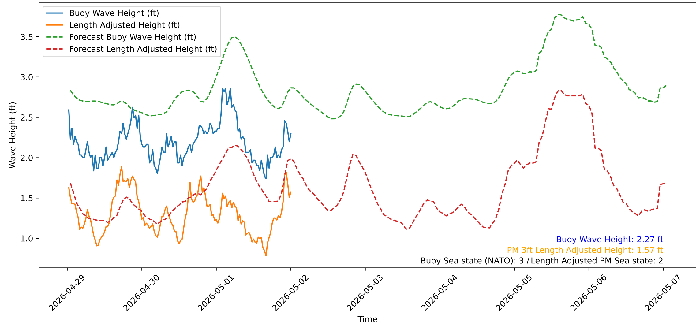
Wave Heights over Time for Green Beach at 2026-05-02 00:41:14
