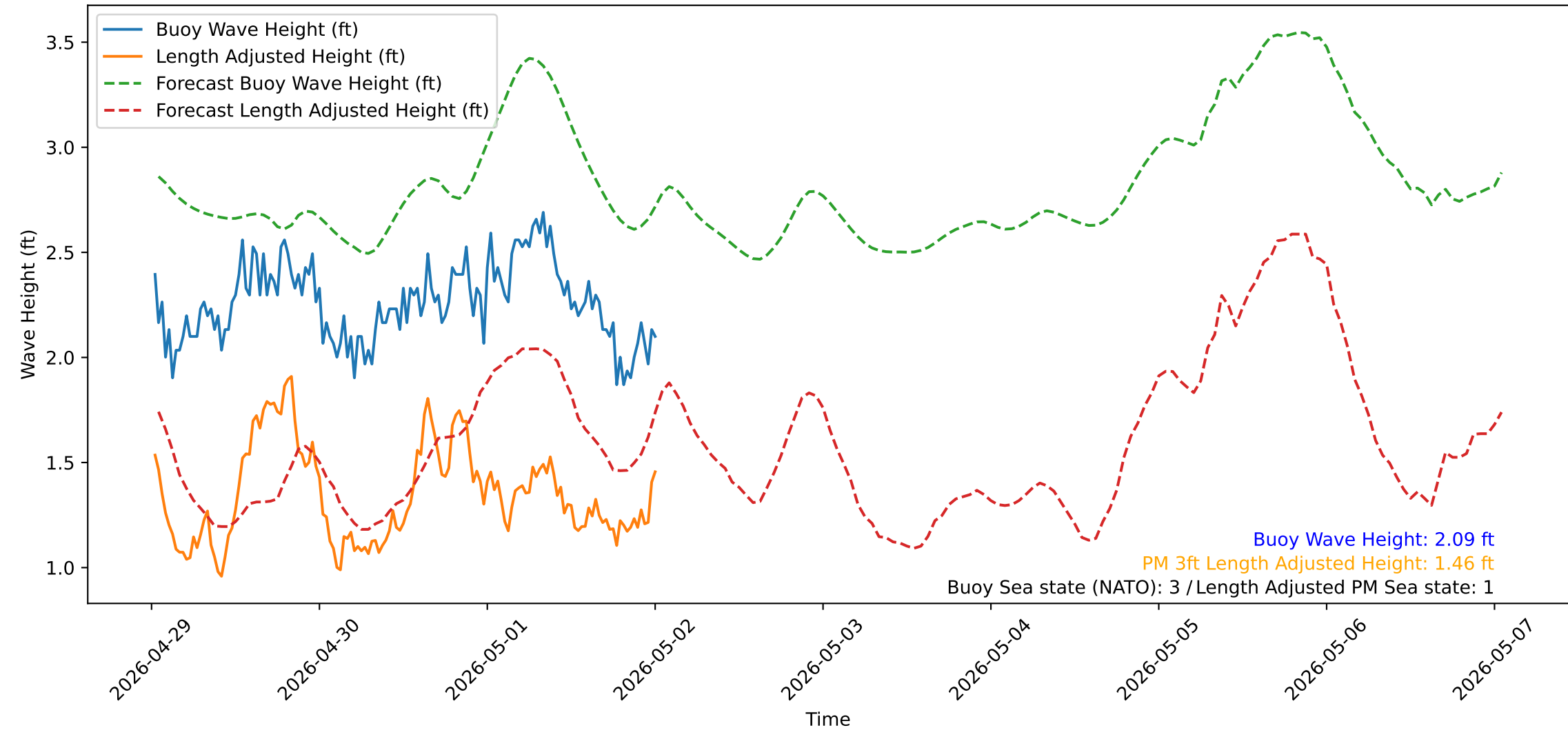
Wave Heights over Time for Oceanside Harbor at 2026-05-02 00:40:32
