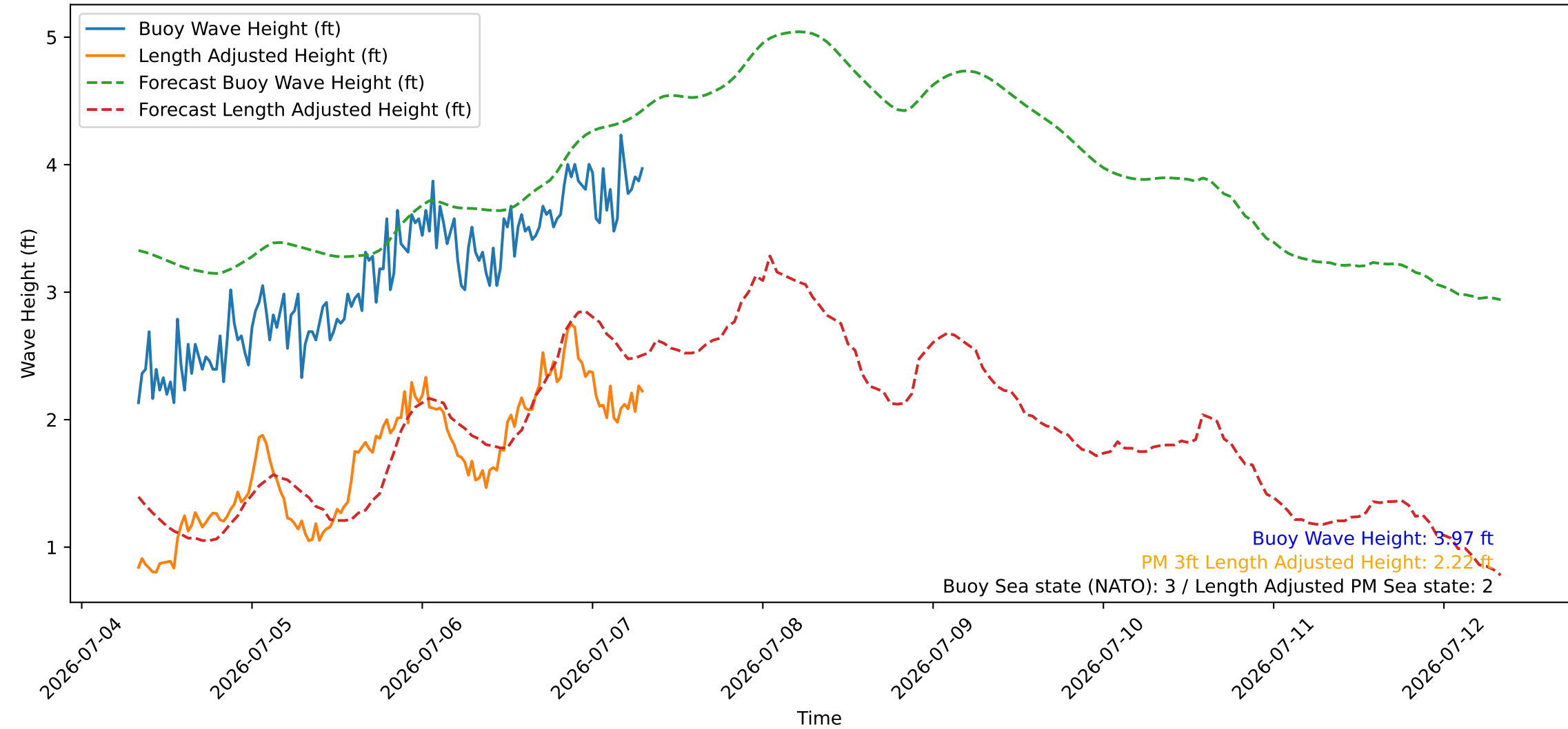
Wave Heights over Time for Oceanside Harbor at 2026-07-07 07:50:27
