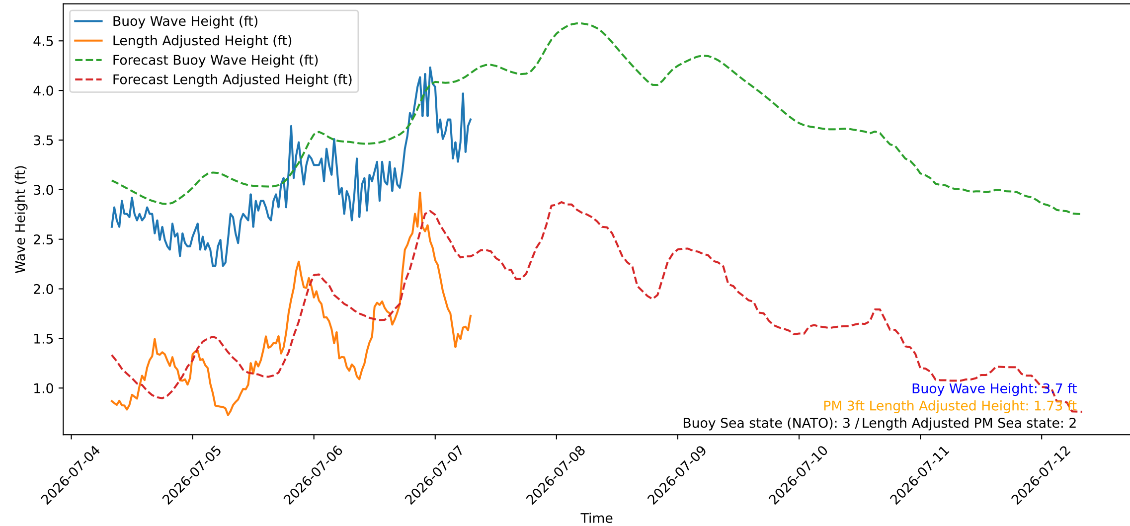
Wave Heights over Time for Red Beach at 2026-07-07 07:50:47
