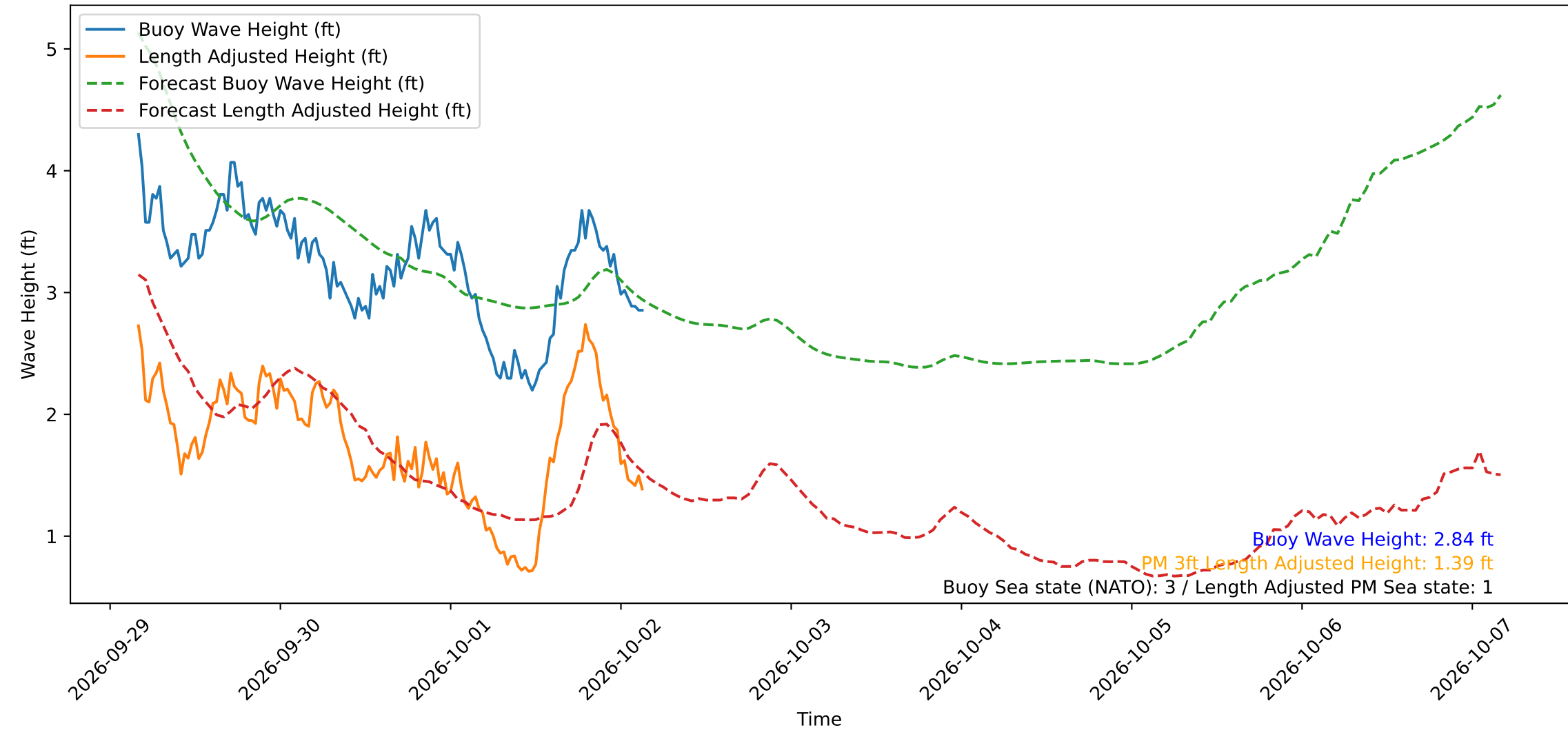
Wave Heights over Time for Green Beach at 2026-10-02 03:51:12
