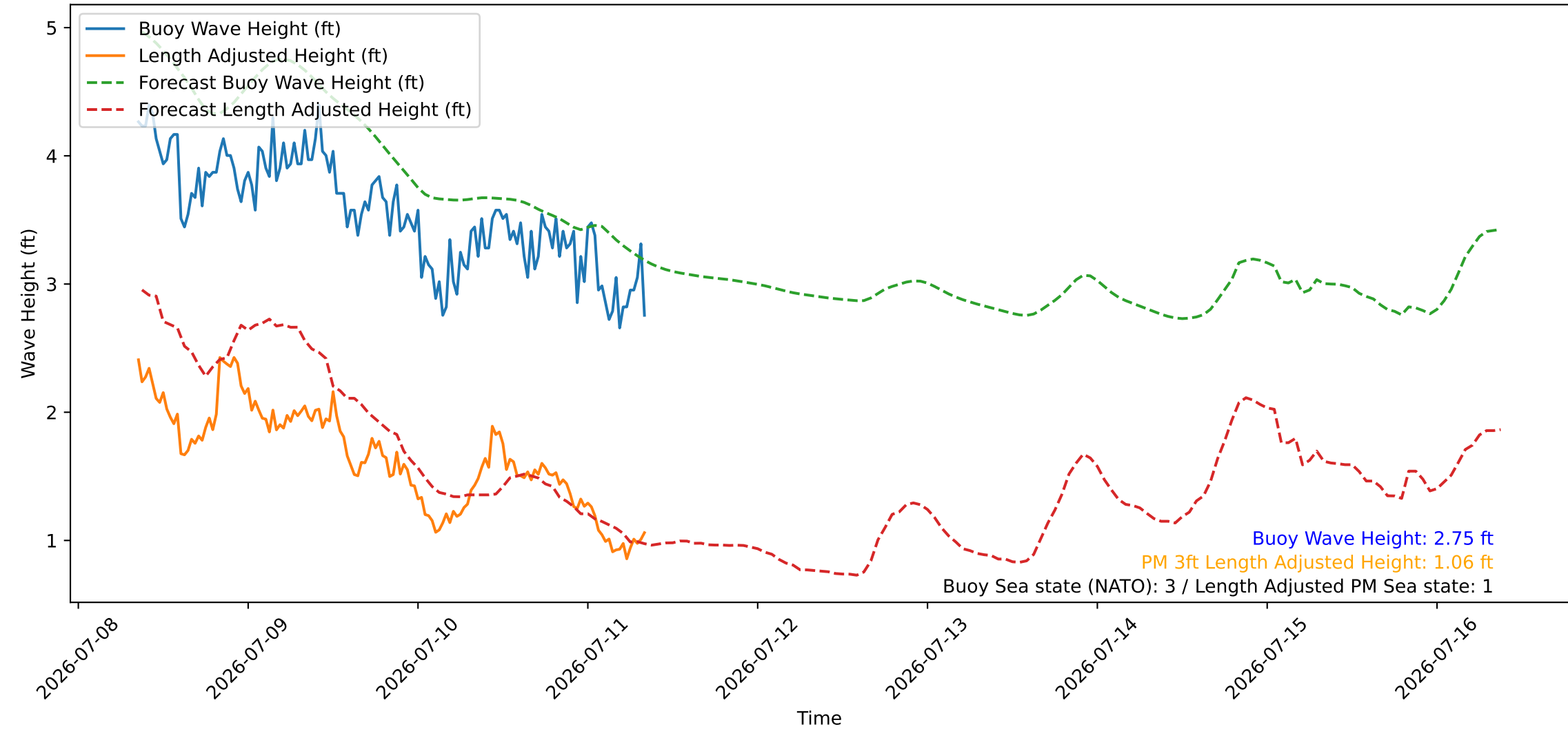
Wave Heights over Time for Green Beach at 2026-07-11 08:41:08
