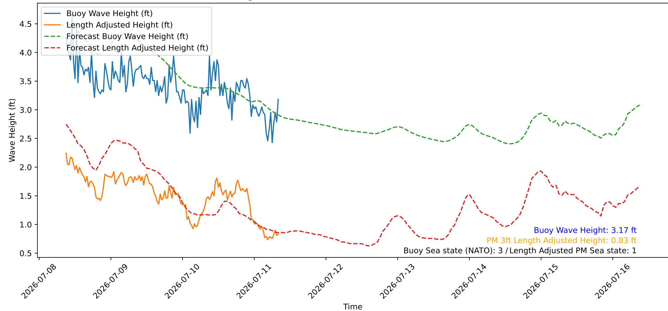
Wave Heights over Time for Red Beach at 2026-07-11 08:40:46
