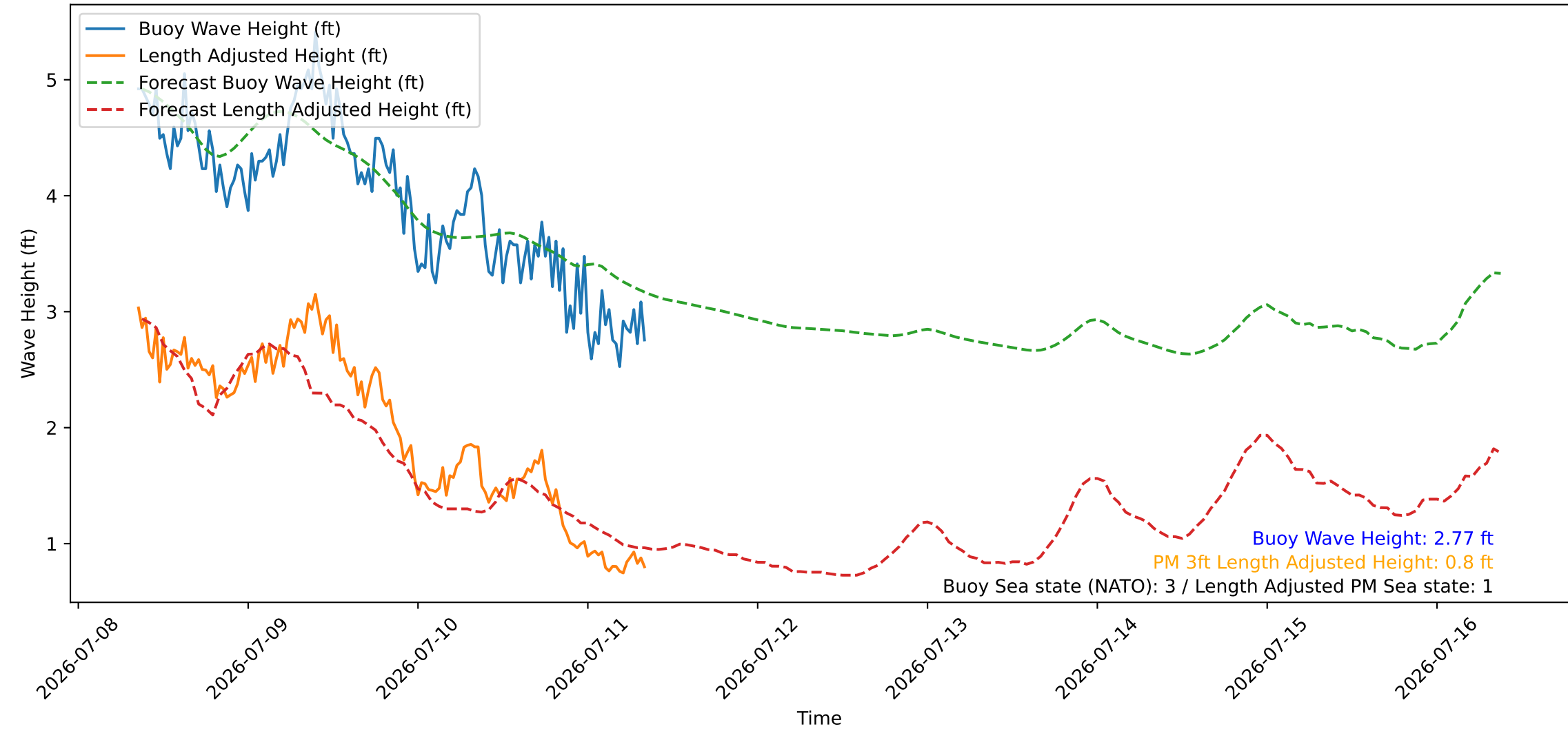
Wave Heights over Time for Oceanside Harbor at 2026-07-11 08:40:27
