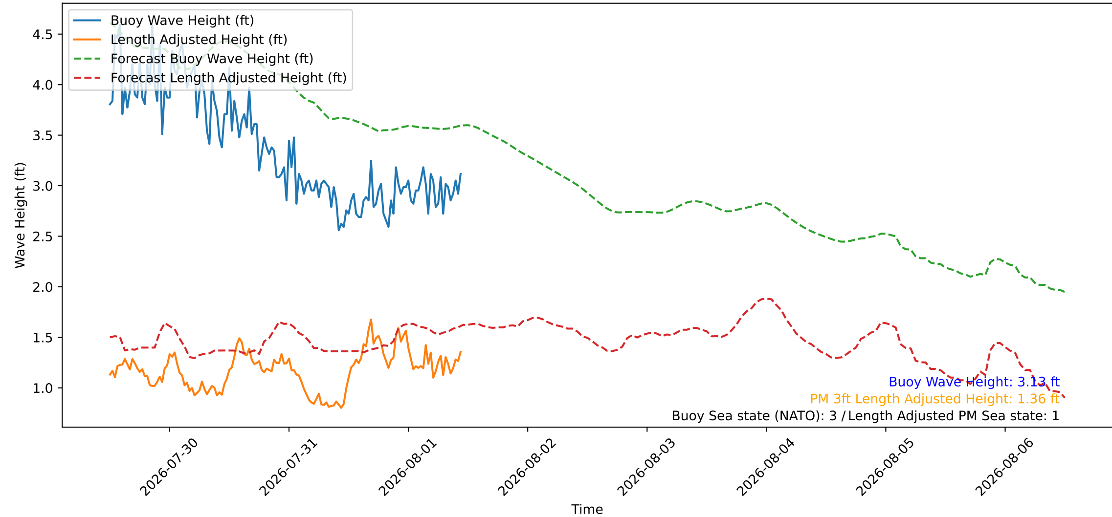
Wave Heights over Time for Red Beach at 2026-08-01 11:40:46
