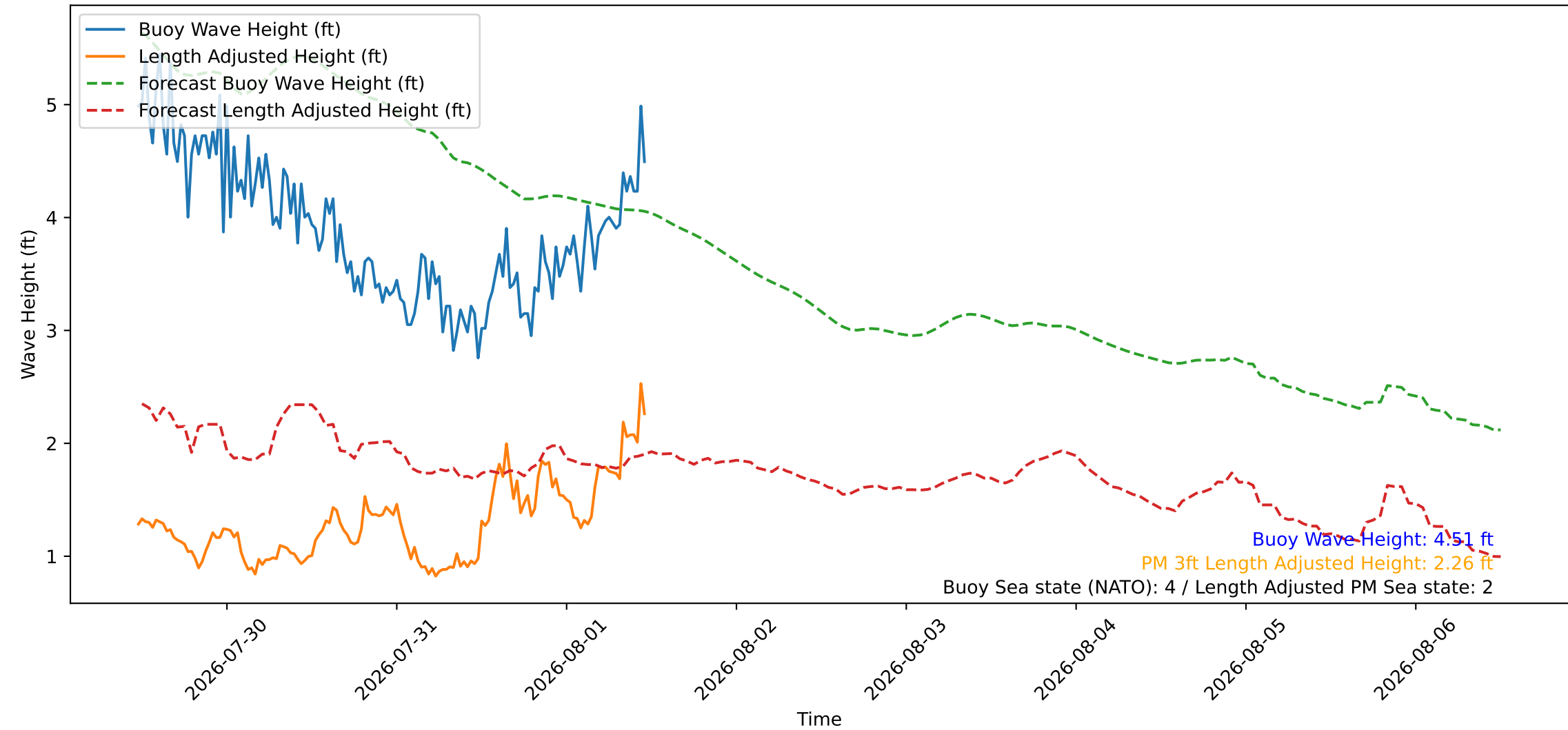
Wave Heights over Time for Green Beach at 2026-08-01 11:41:09
