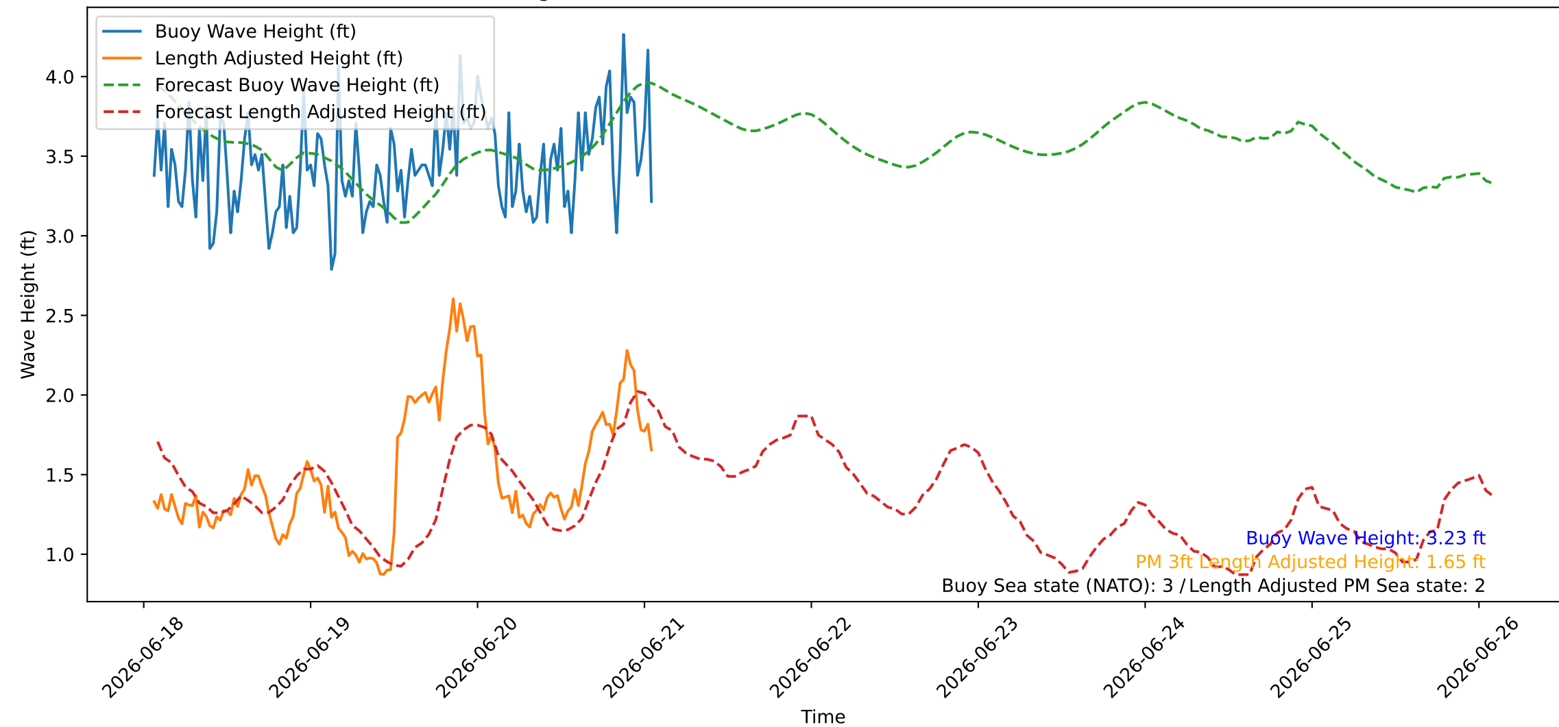
Wave Heights over Time for Oceanside Harbor at 2026-06-21 01:40:26
