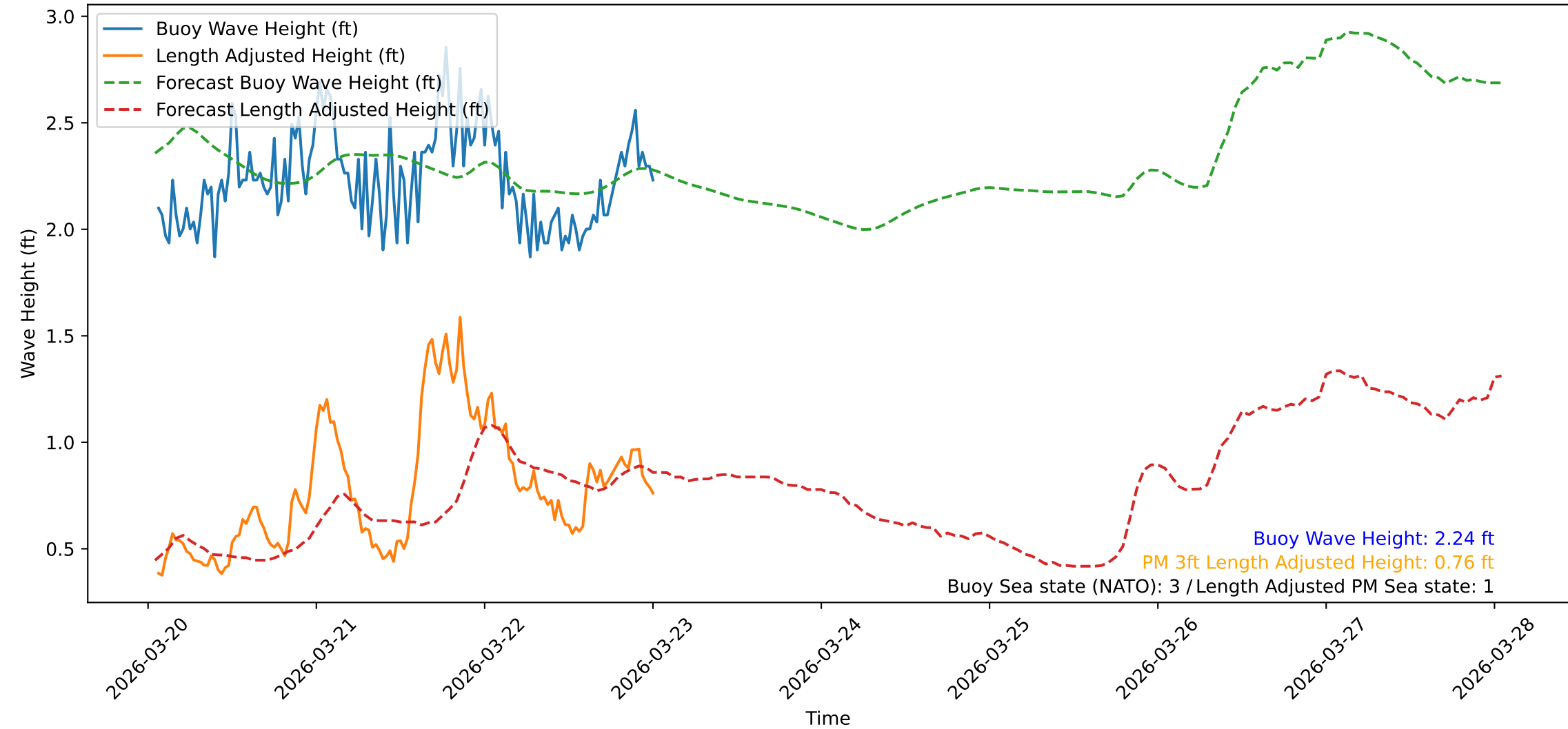
Wave Heights over Time for Red Beach at 2026-03-23 01:00:47
