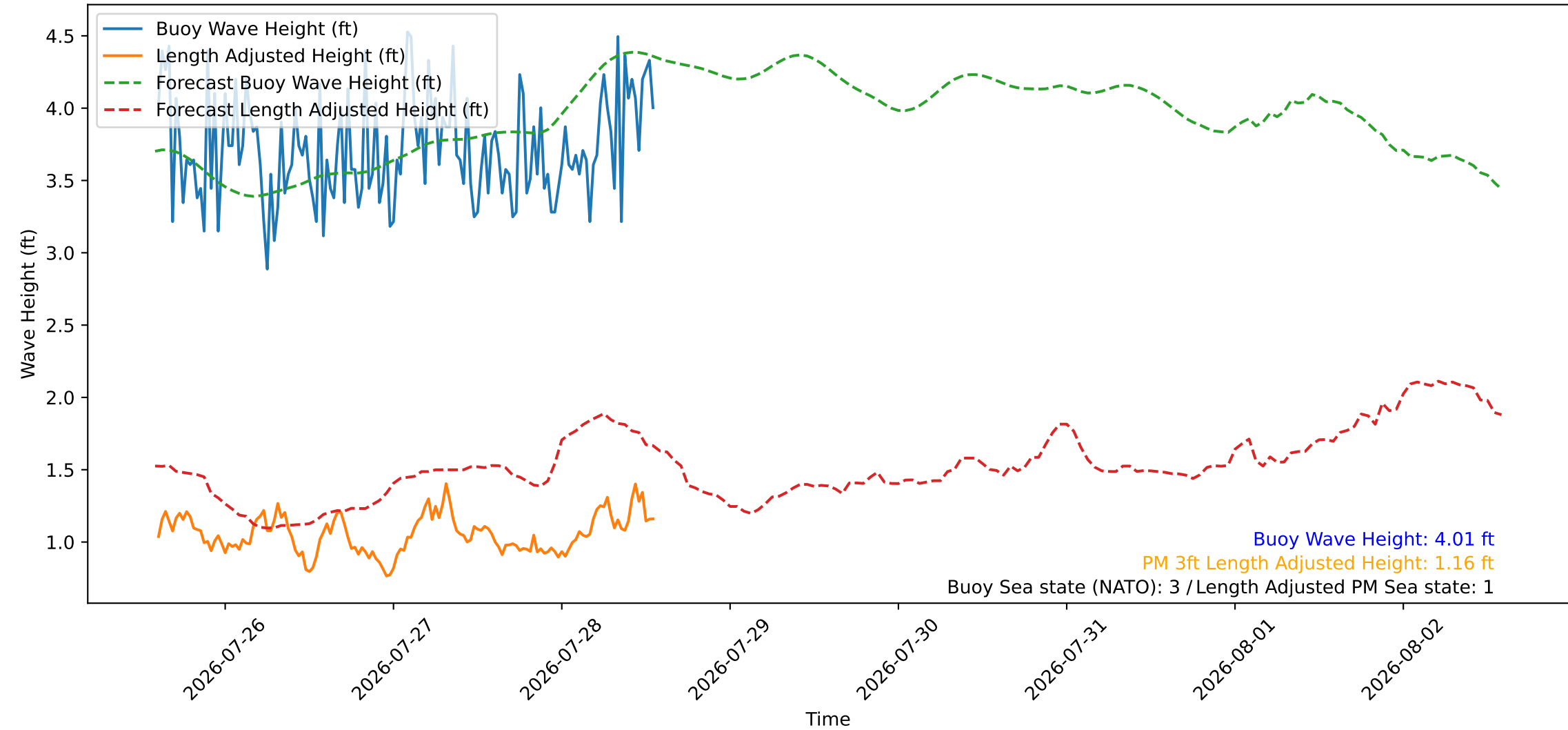
Wave Heights over Time for Red Beach at 2026-07-28 14:00:46
