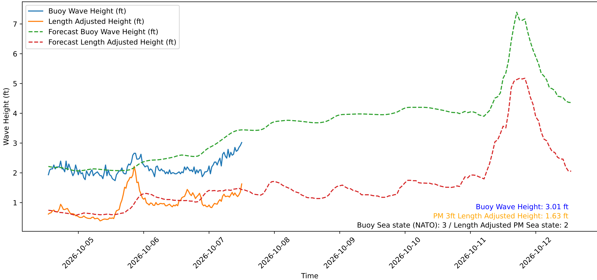
Wave Heights over Time for Red Beach at 2026-10-07 12:50:51
