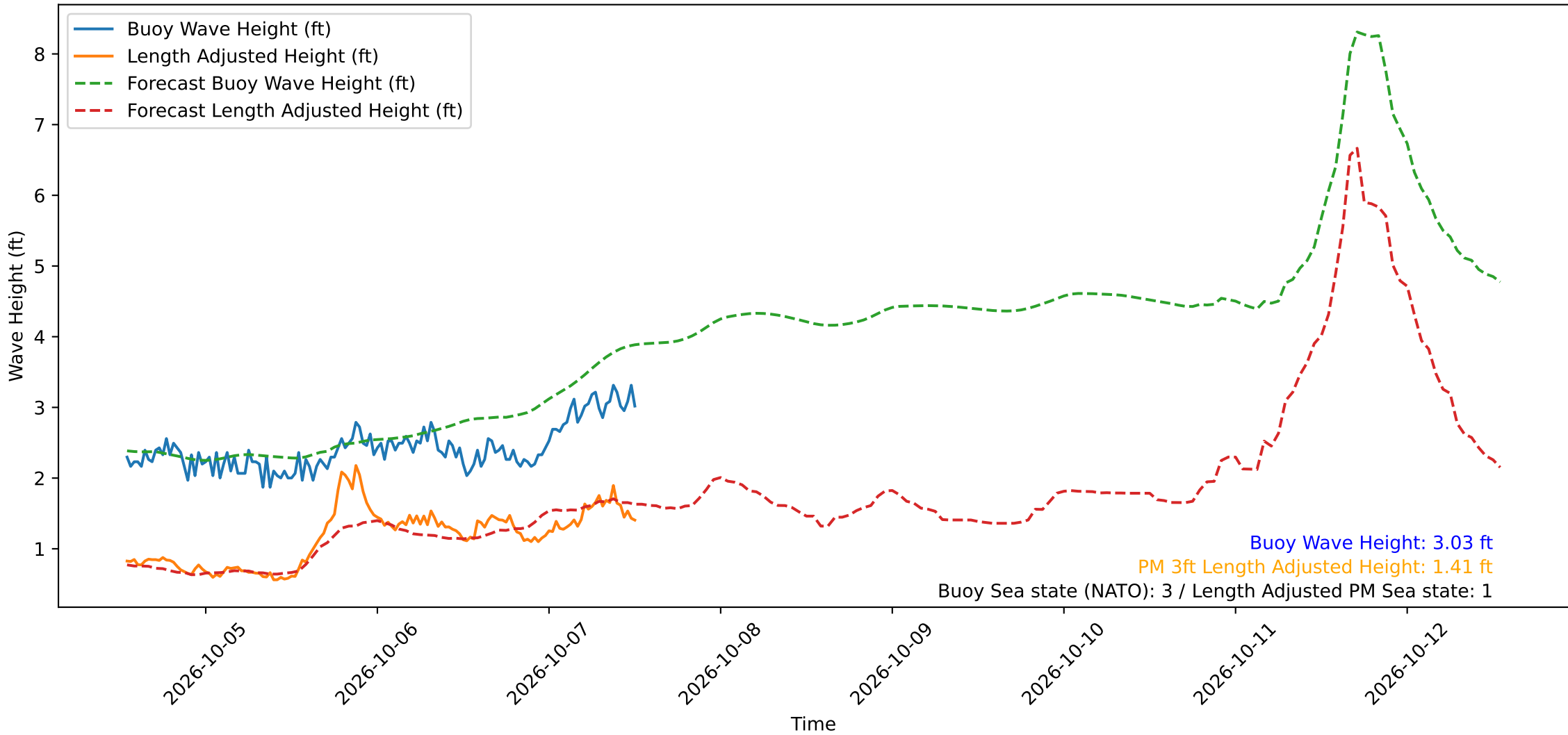
Wave Heights over Time for Oceanside Harbor at 2026-10-07 12:50:30
