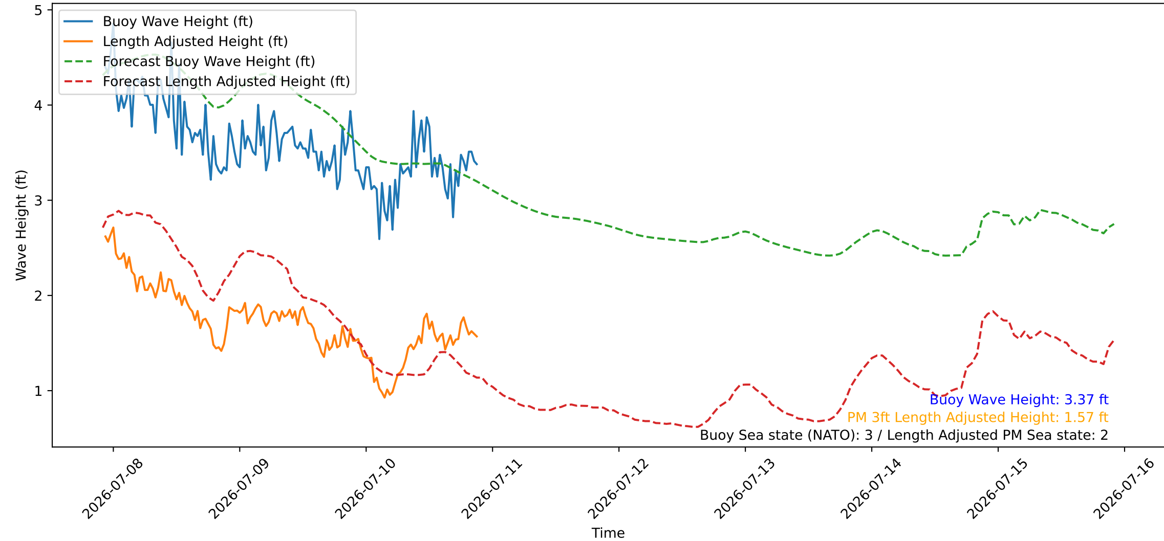
Wave Heights over Time for Red Beach at 2026-07-10 22:00:45
