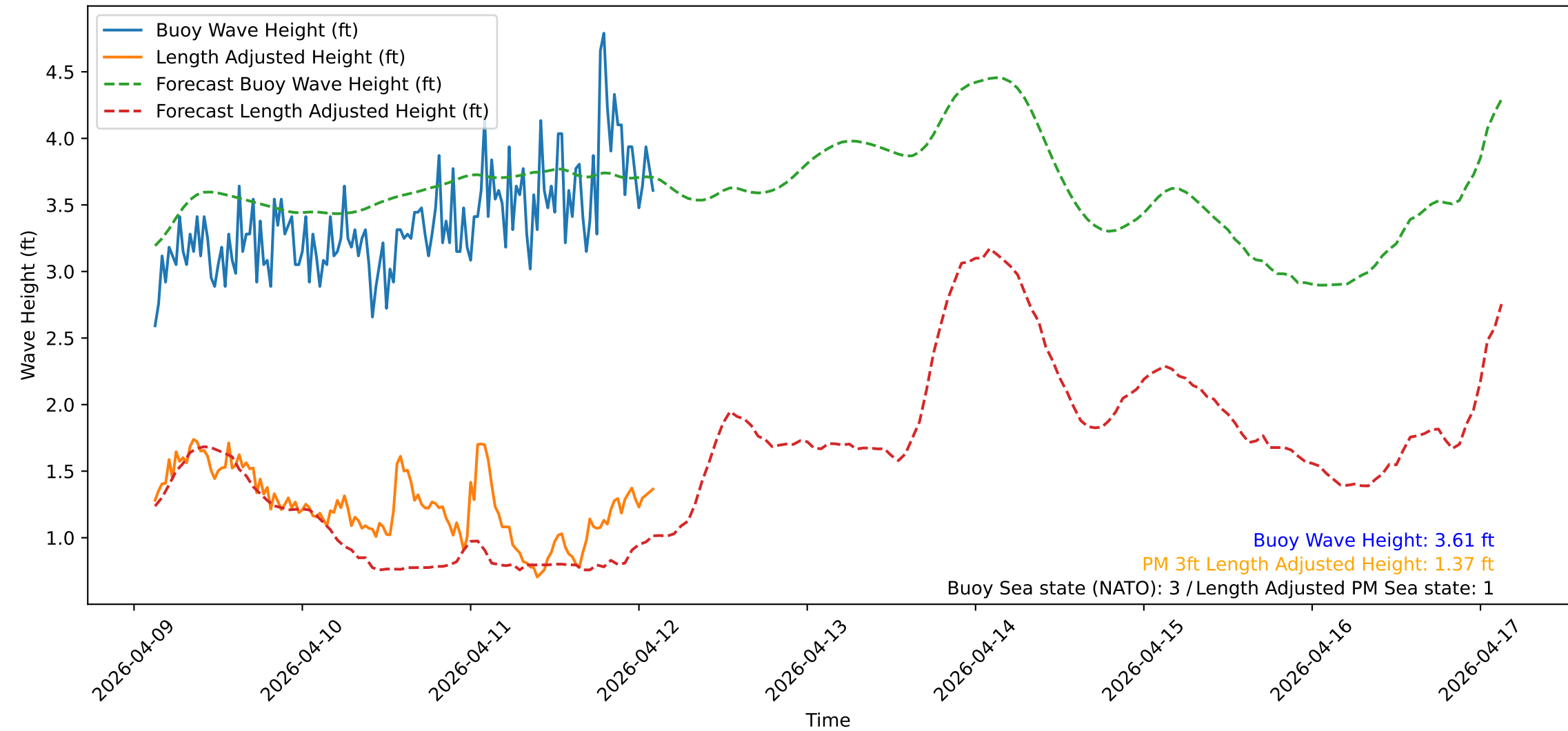
Wave Heights over Time for Oceanside Harbor at 2026-04-12 02:50:32
