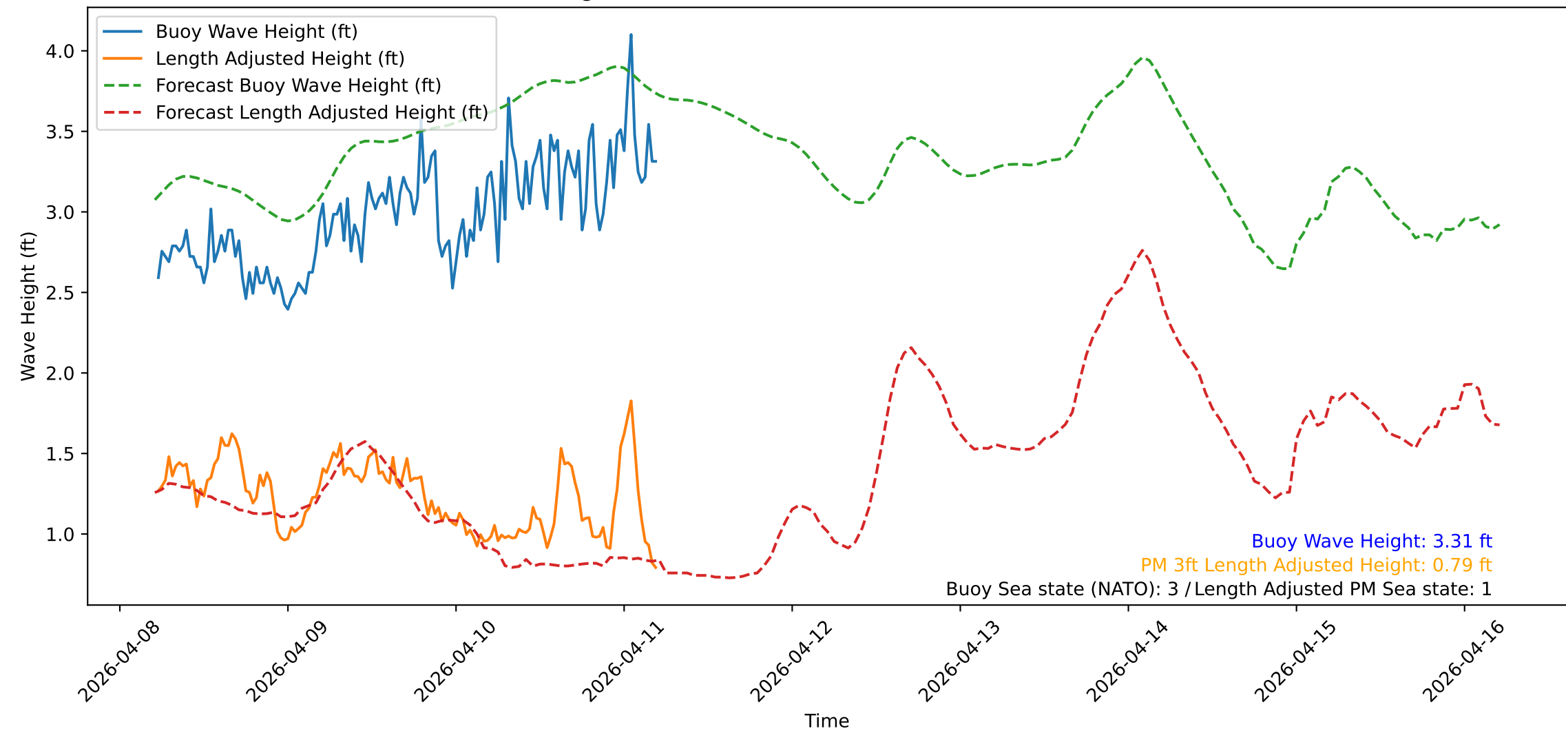
Wave Heights over Time for Red Beach at 2026-04-11 05:20:52
