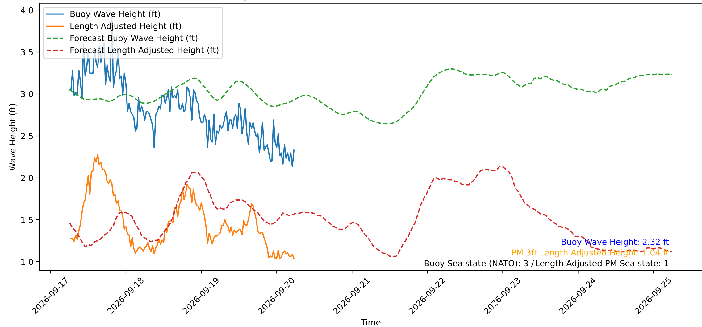
Wave Heights over Time for Oceanside Harbor at 2026-09-20 06:20:30
