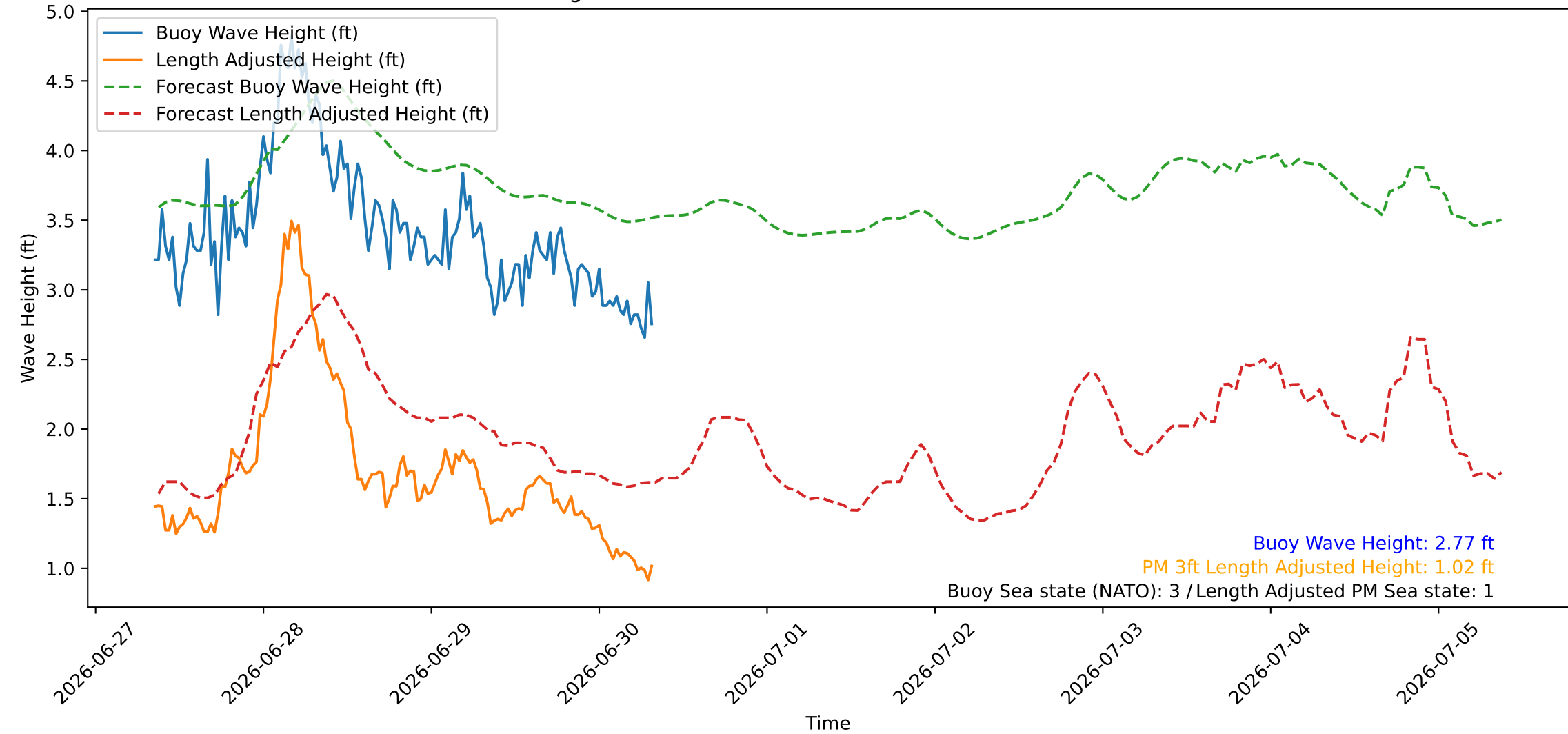
Wave Heights over Time for Green Beach at 2026-06-30 08:31:08
