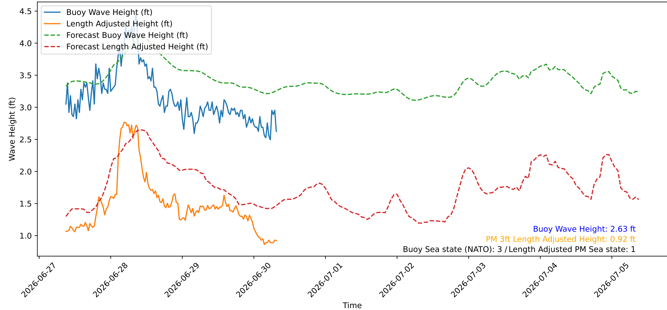
Wave Heights over Time for Red Beach at 2026-06-30 08:30:45
