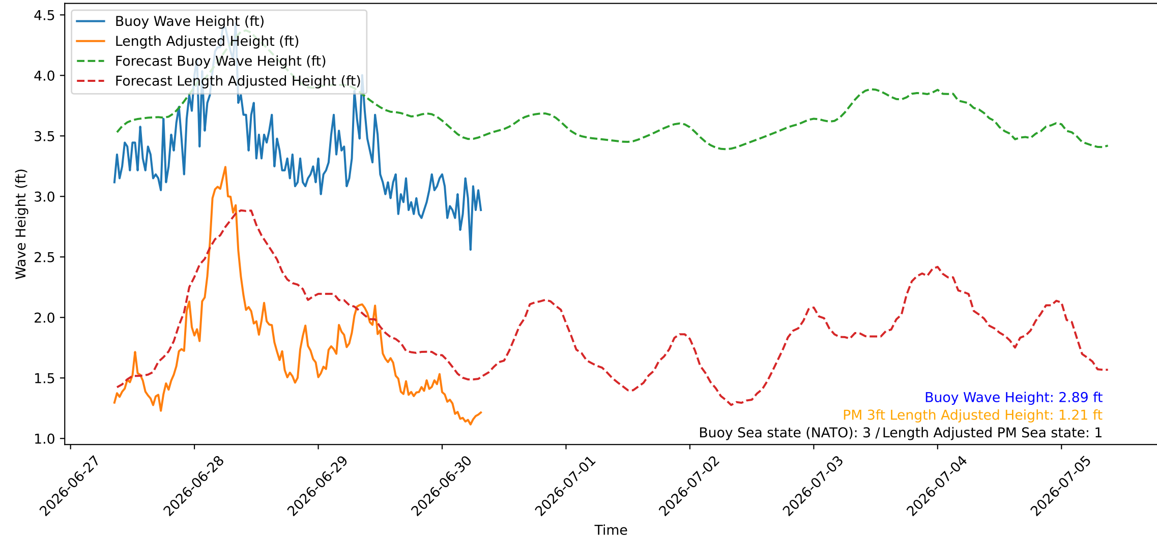
Wave Heights over Time for Oceanside Harbor at 2026-06-30 08:30:26
