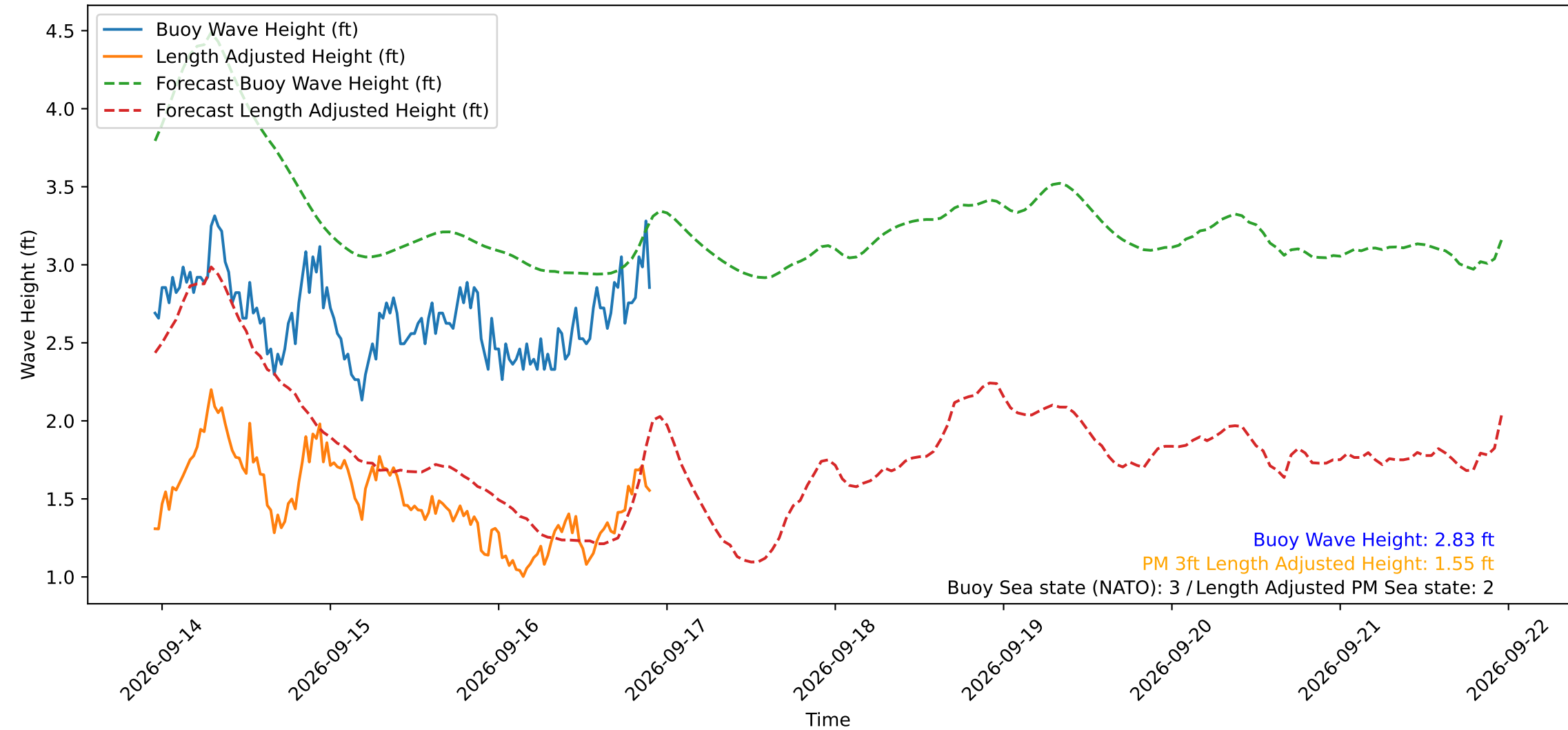
Wave Heights over Time for Green Beach at 2026-09-16 22:51:14
