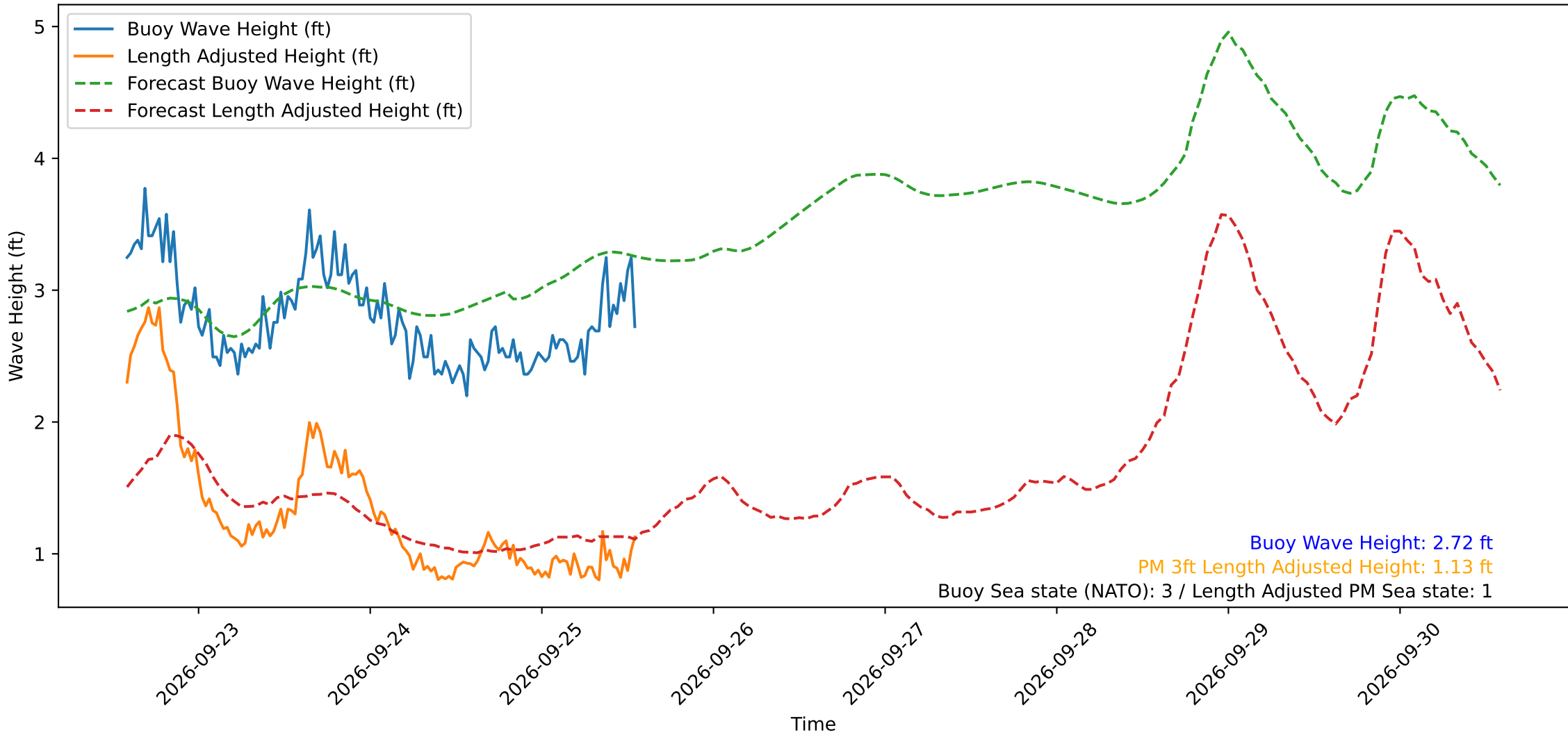
Wave Heights over Time for Oceanside Harbor at 2026-09-25 14:00:30
