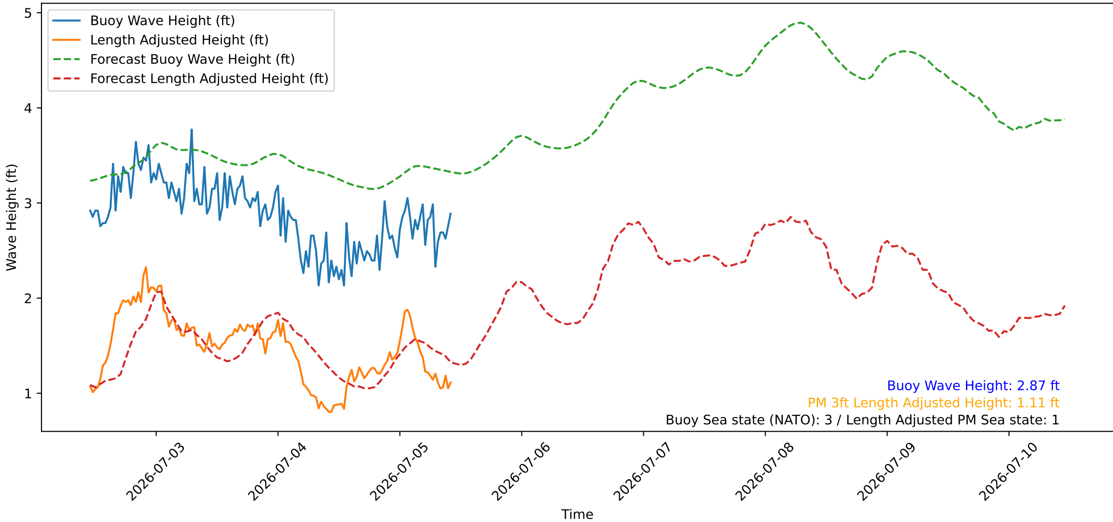
Wave Heights over Time for Oceanside Harbor at 2026-07-05 11:00:28
