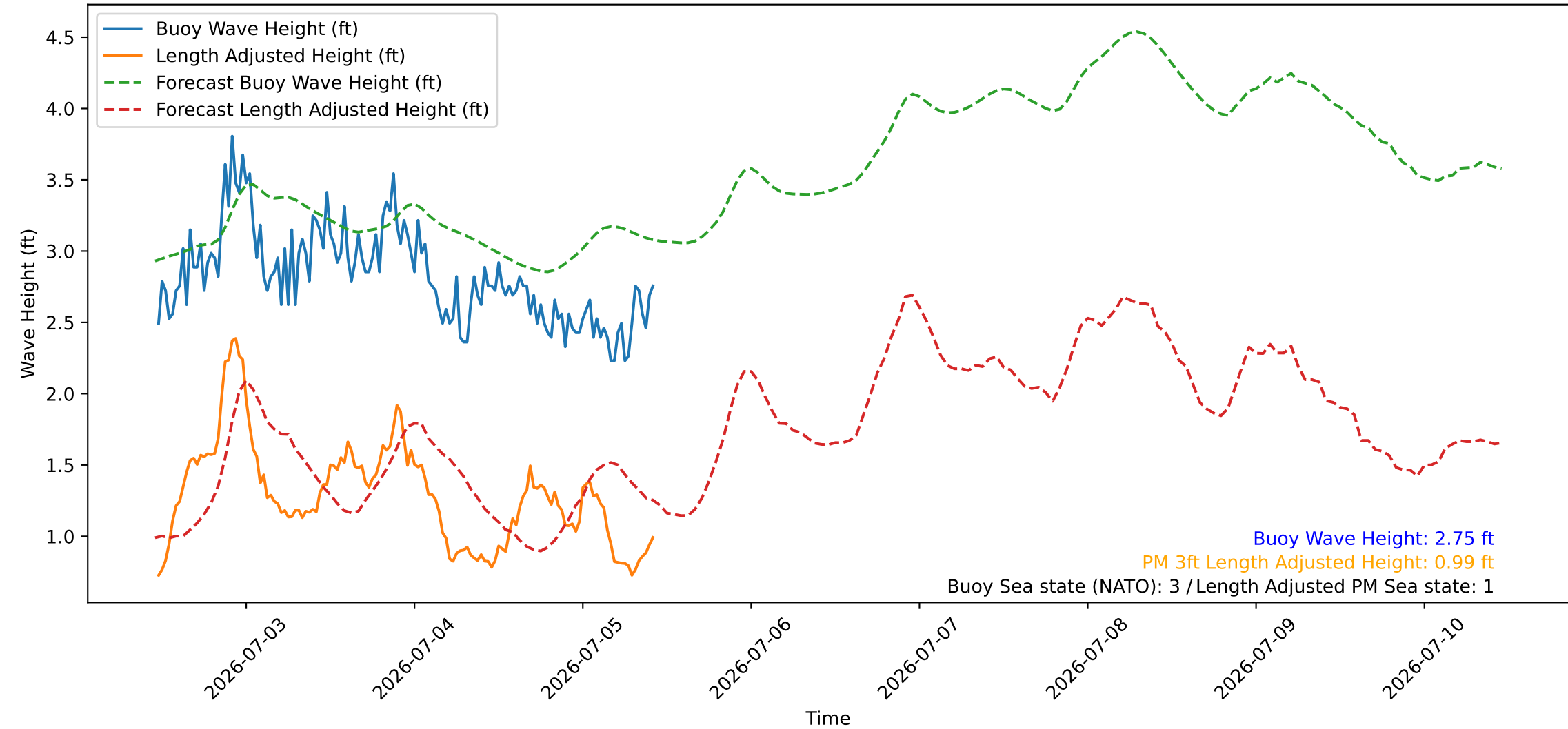
Wave Heights over Time for Red Beach at 2026-07-05 11:00:50
