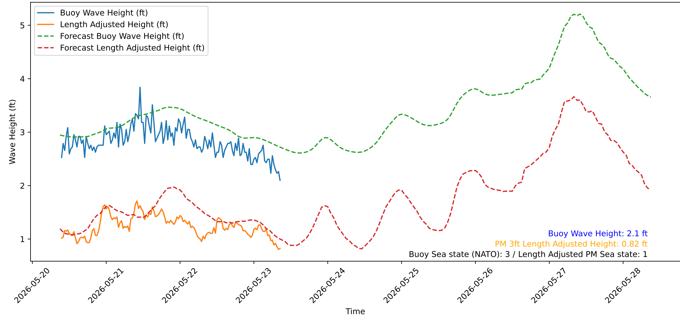
Wave Heights over Time for Oceanside Harbor at 2026-05-23 09:20:31
