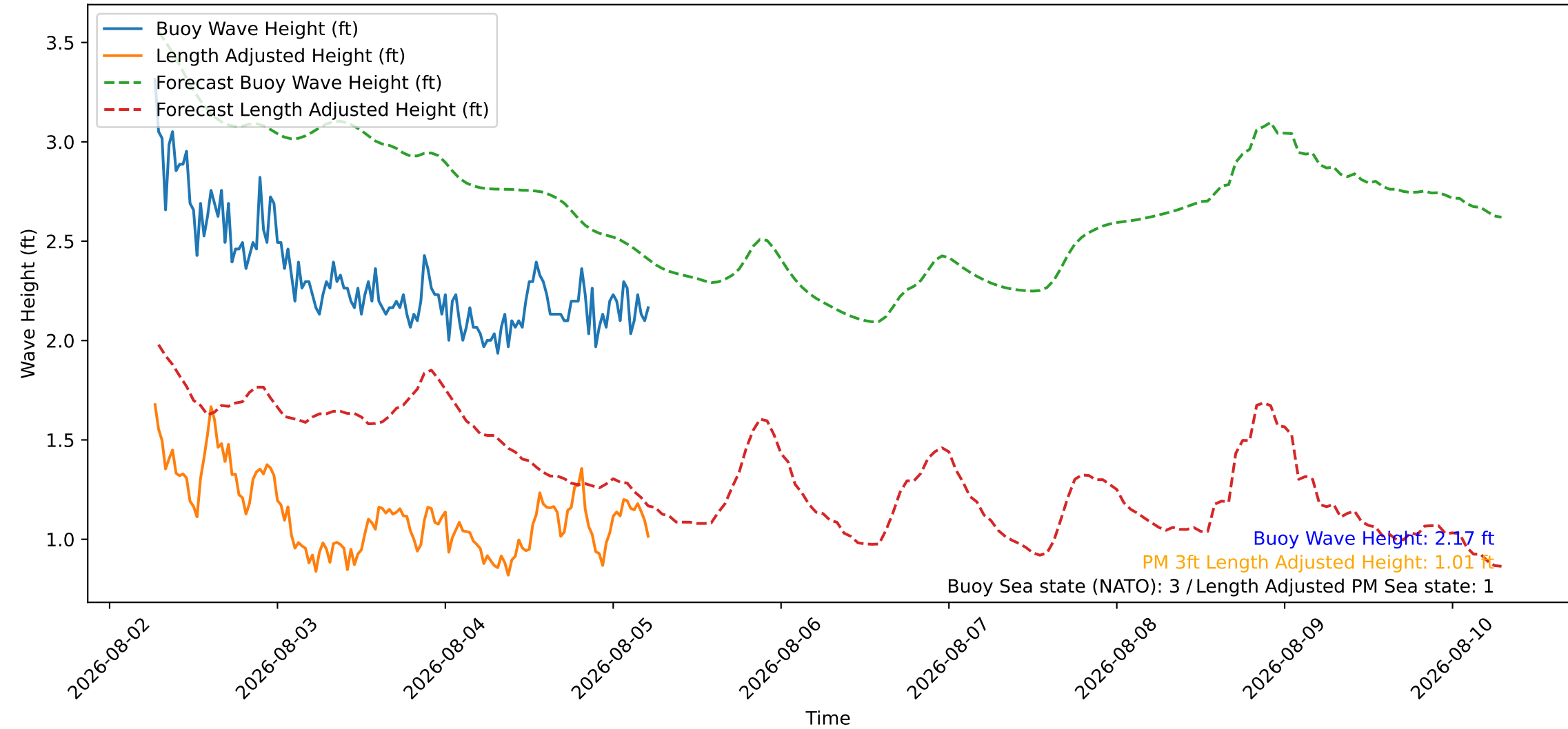
Wave Heights over Time for Green Beach at 2026-08-05 06:31:09
