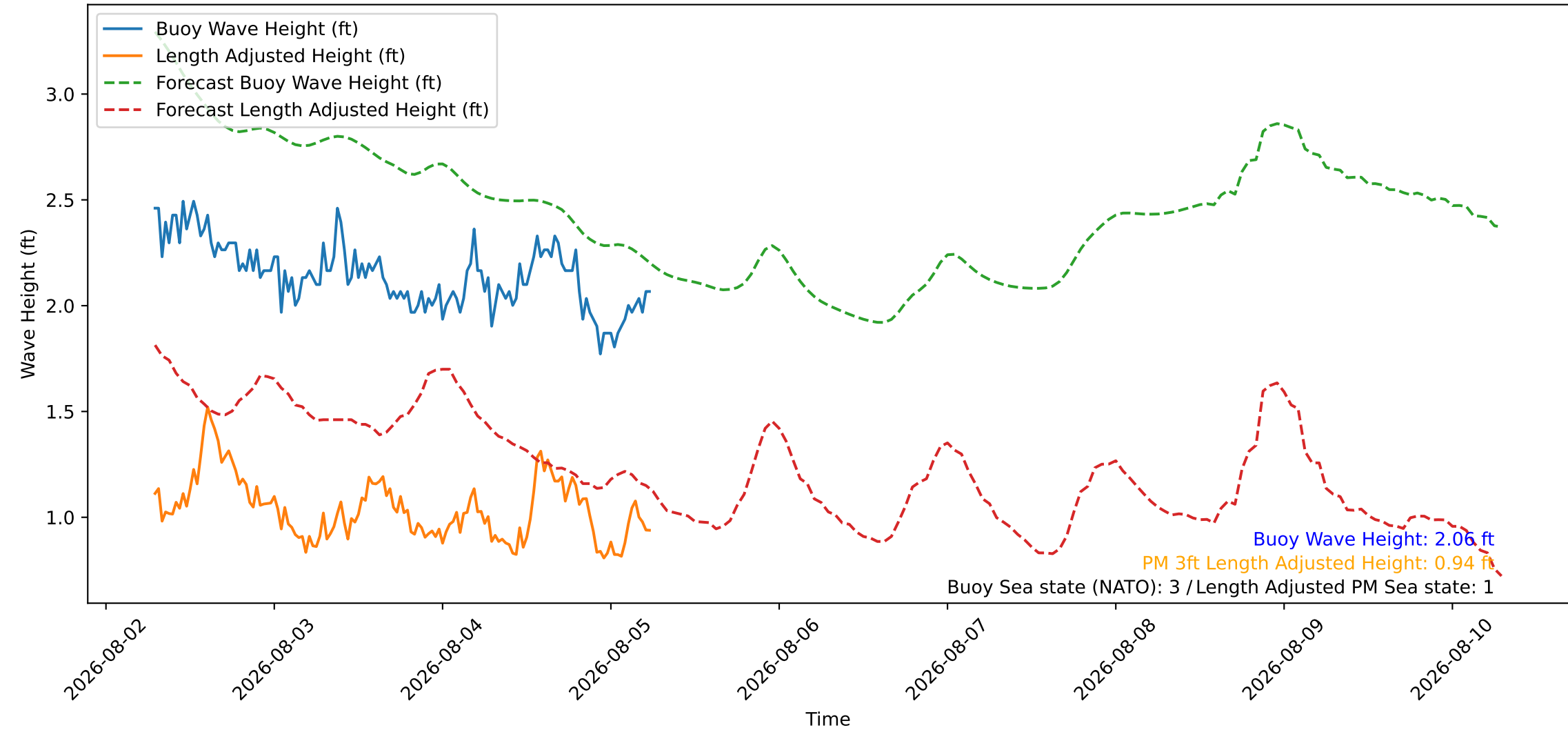
Wave Heights over Time for Red Beach at 2026-08-05 06:30:47
