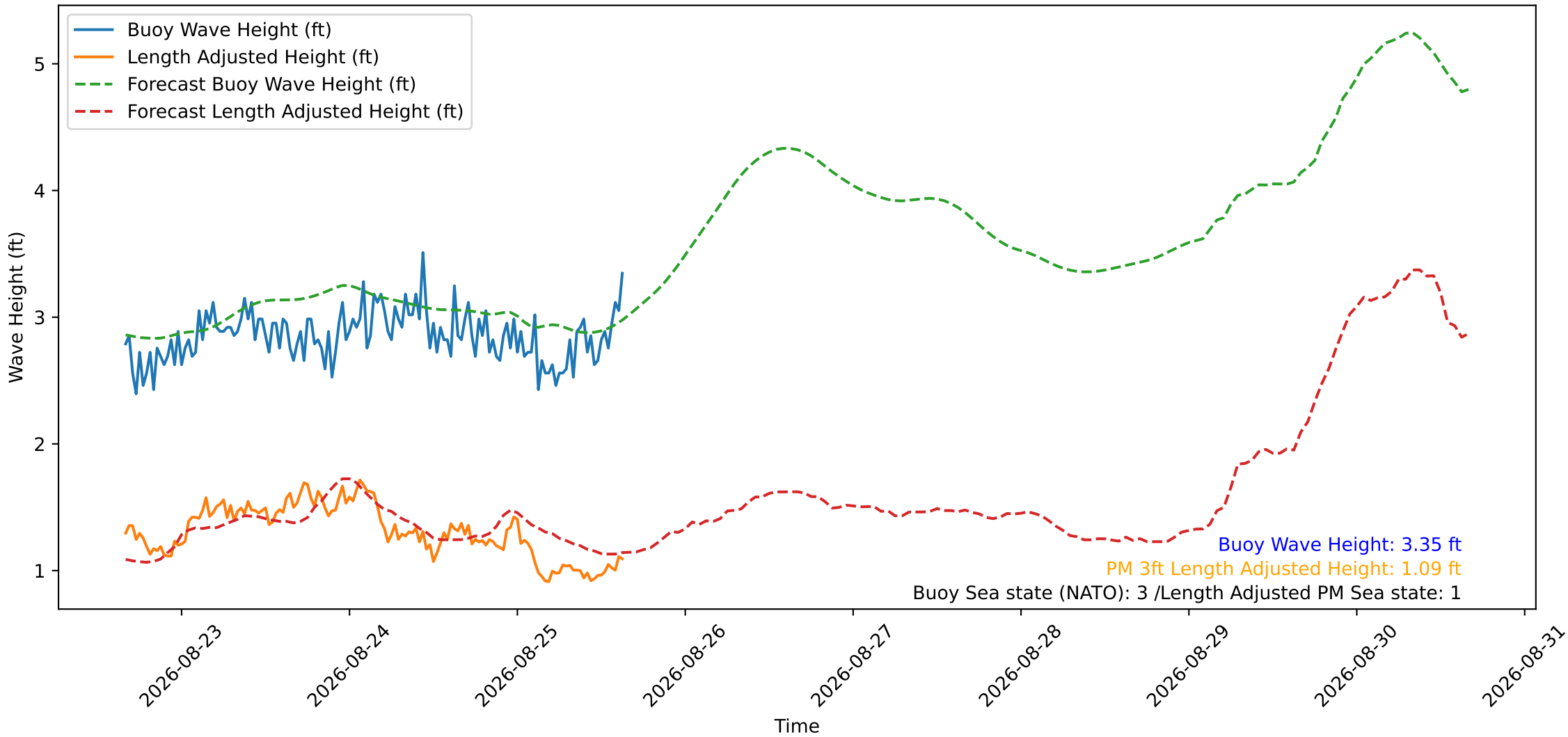
Wave Heights over Time for Oceanside Harbor at 2026-08-25 15:50:29
