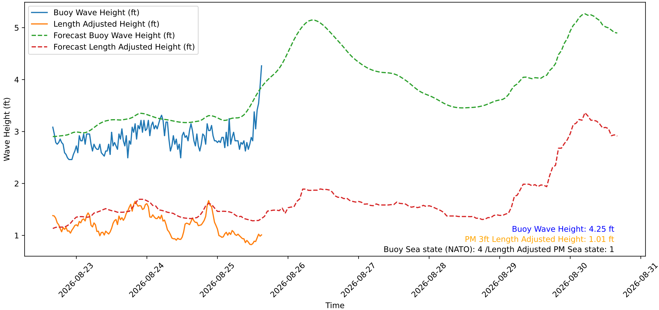
Wave Heights over Time for Green Beach at 2026-08-25 15:51:14
