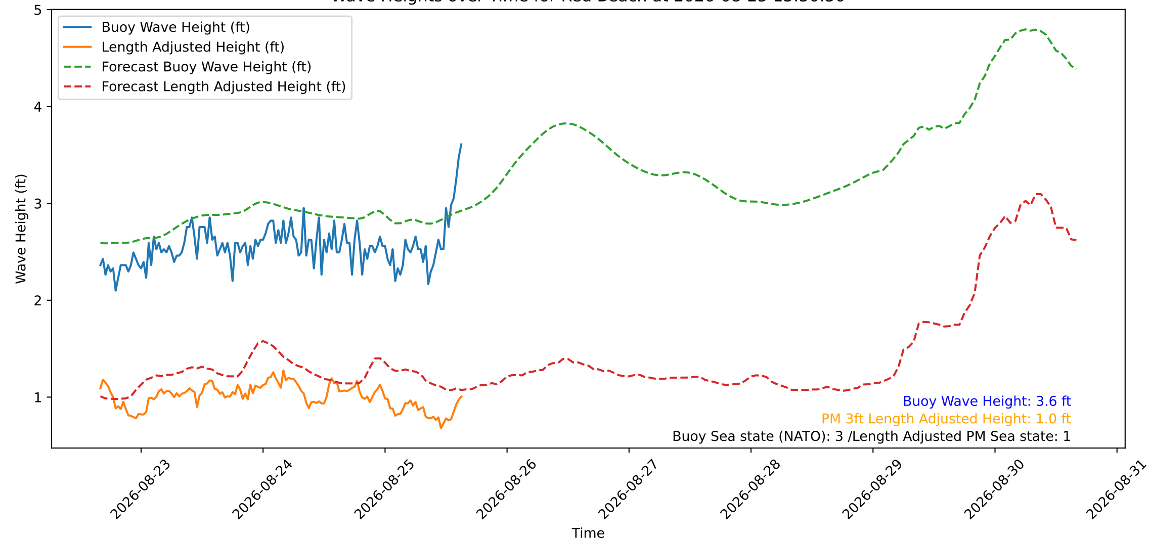
Wave Heights over Time for Red Beach at 2026-08-25 15:50:50
