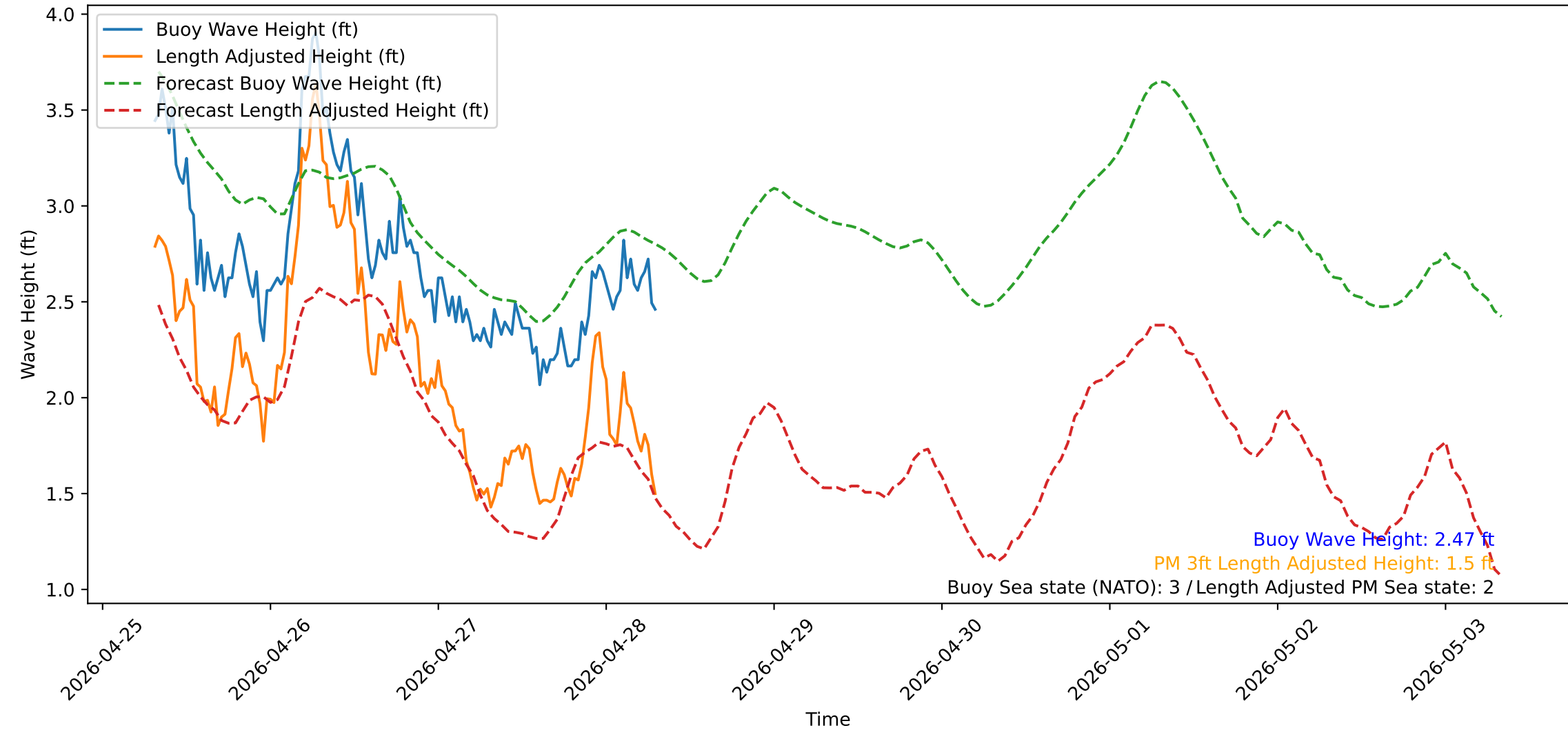
Wave Heights over Time for Oceanside Harbor at 2026-04-28 07:40:31
