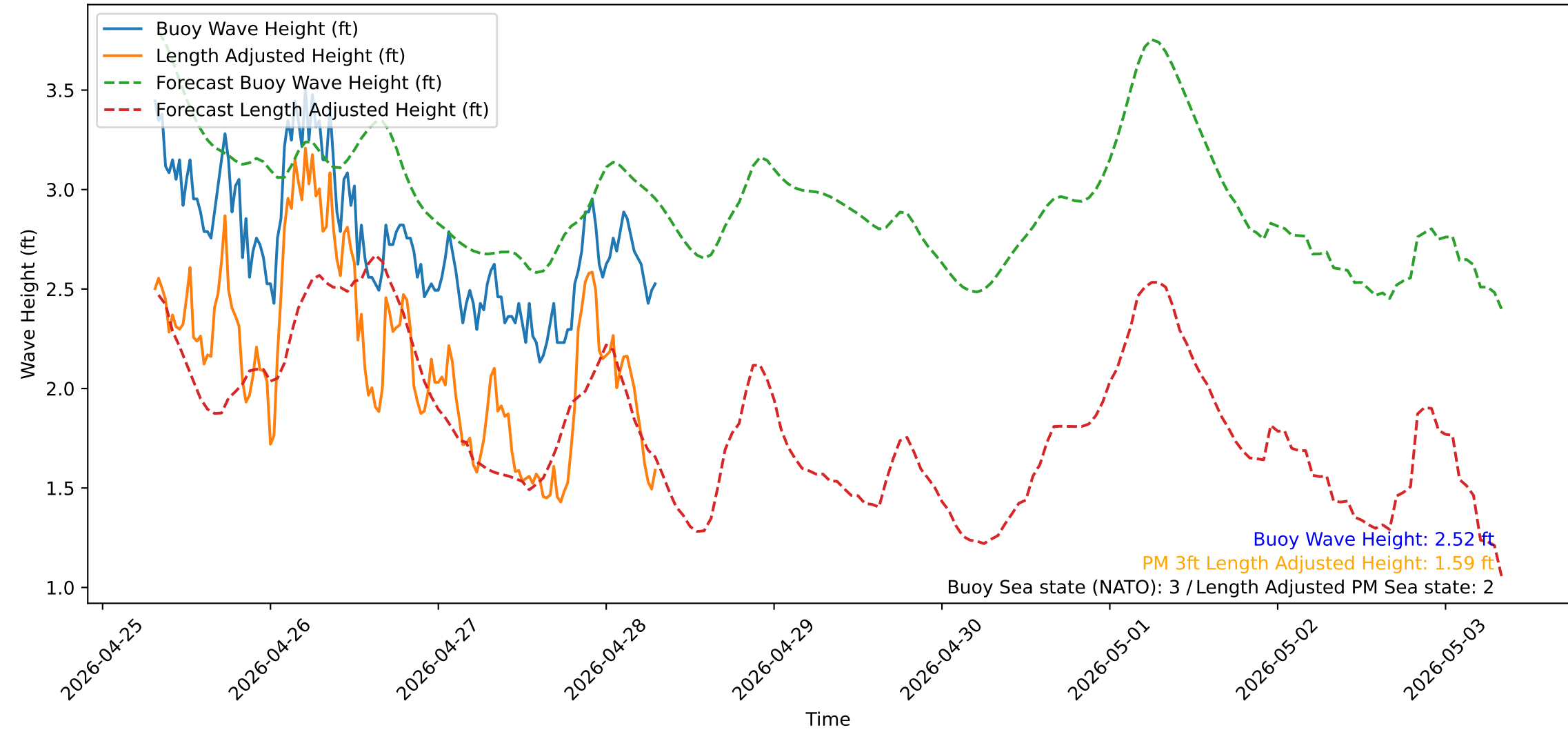
Wave Heights over Time for Green Beach at 2026-04-28 07:41:13
