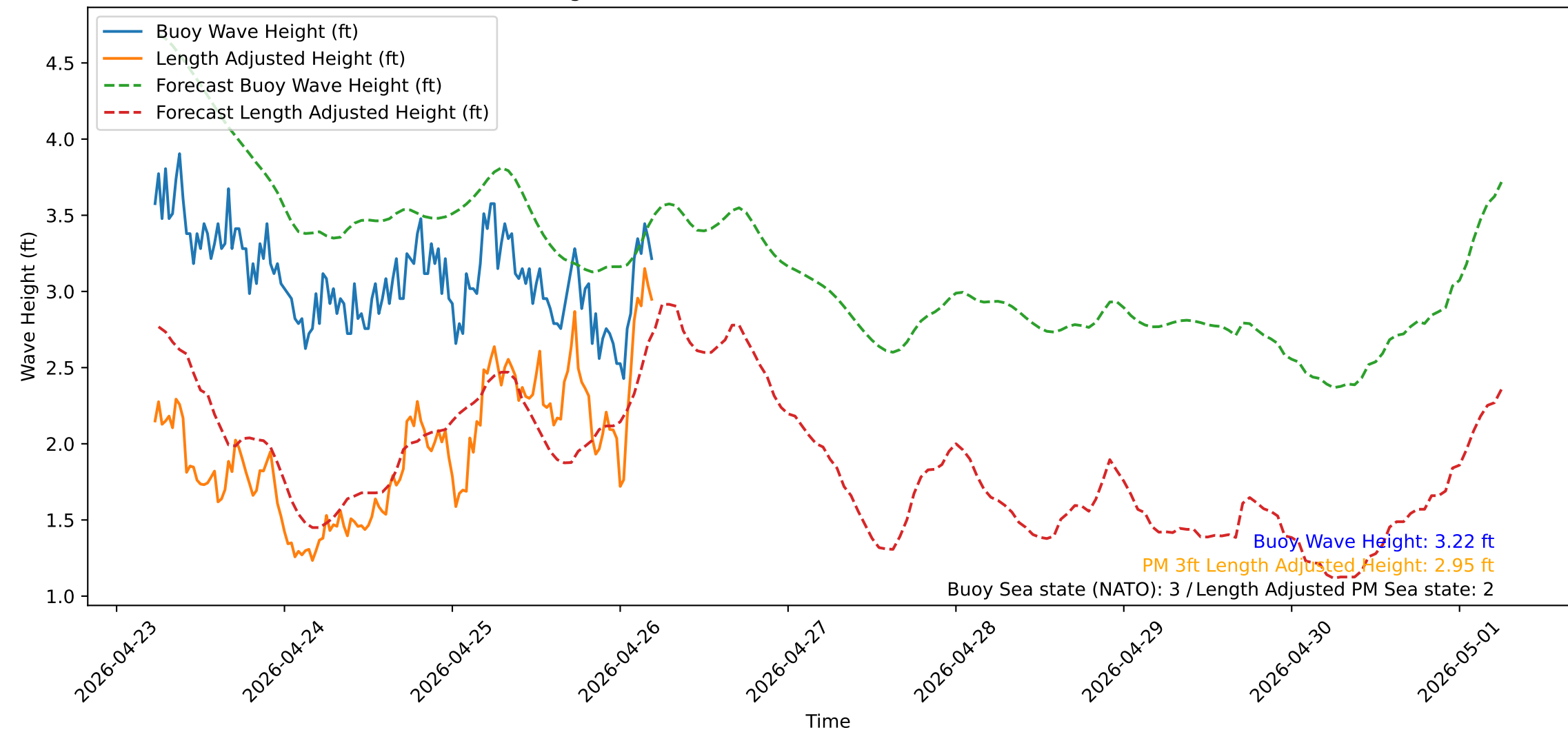
Wave Heights over Time for Green Beach at 2026-04-26 05:31:12
