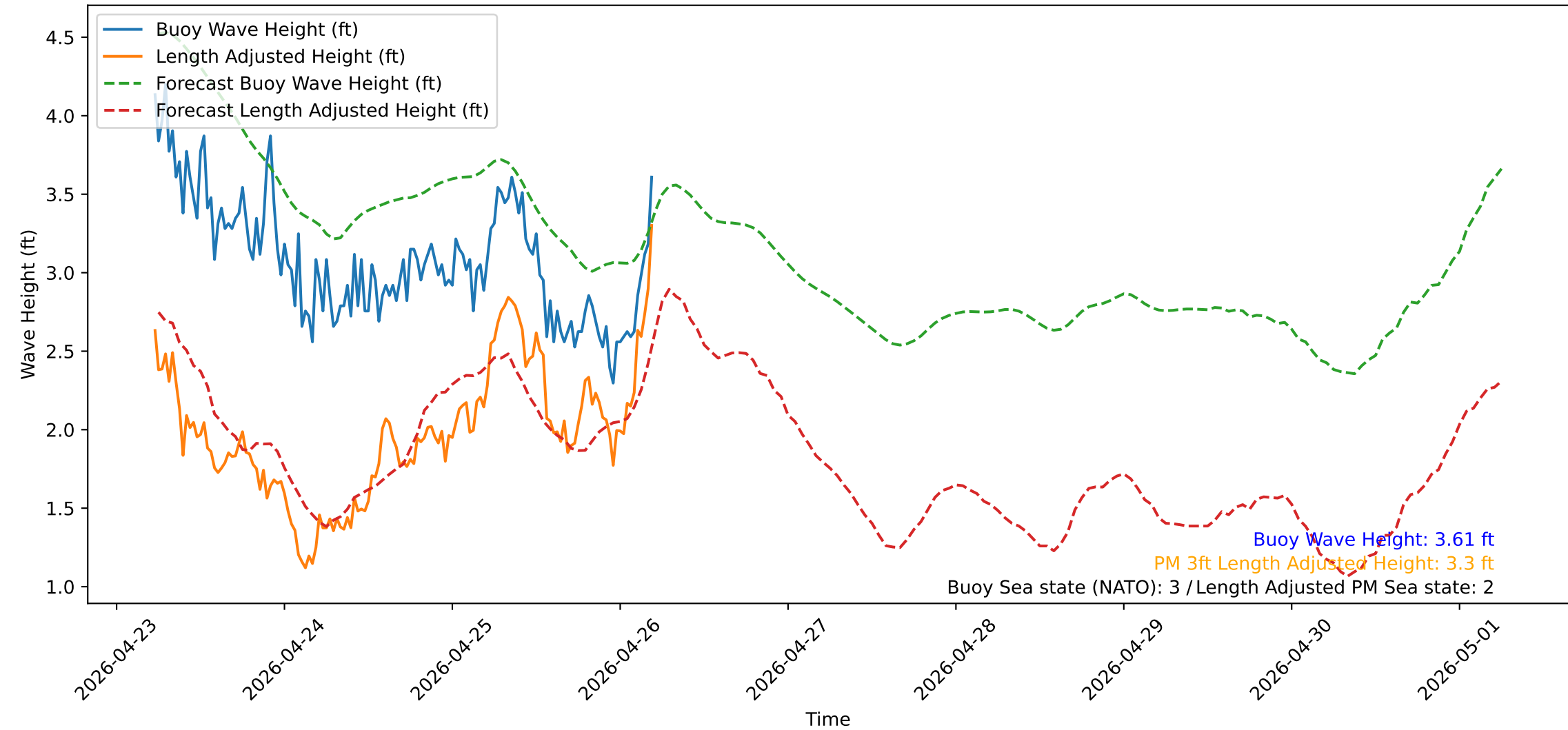
Wave Heights over Time for Oceanside Harbor at 2026-04-26 05:30:30
