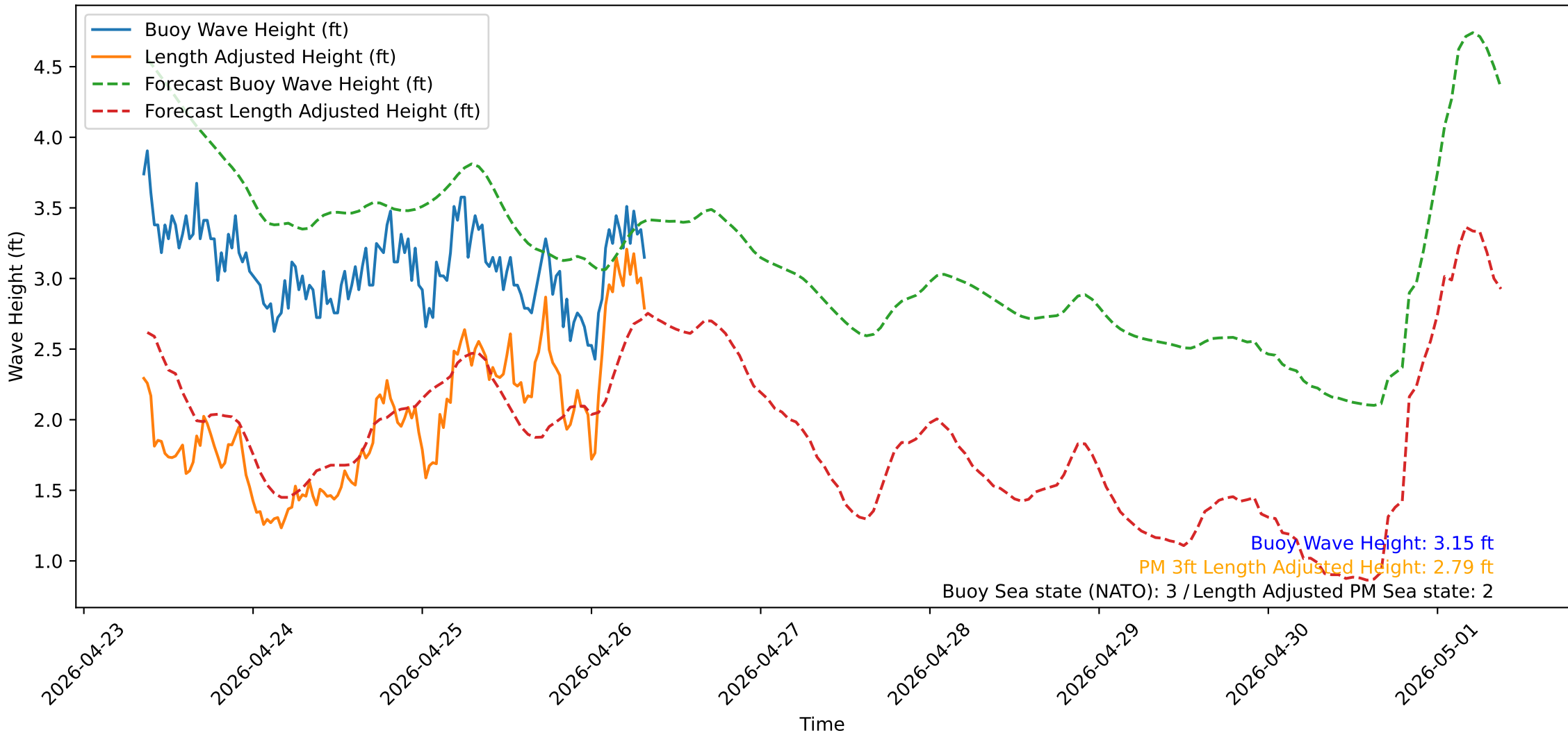
Wave Heights over Time for Green Beach at 2026-04-26 08:31:12
