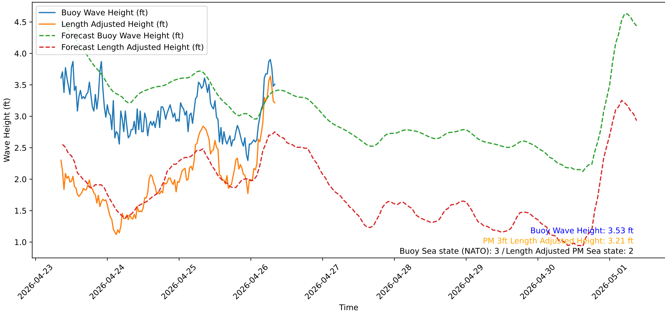
Wave Heights over Time for Oceanside Harbor at 2026-04-26 08:30:31
