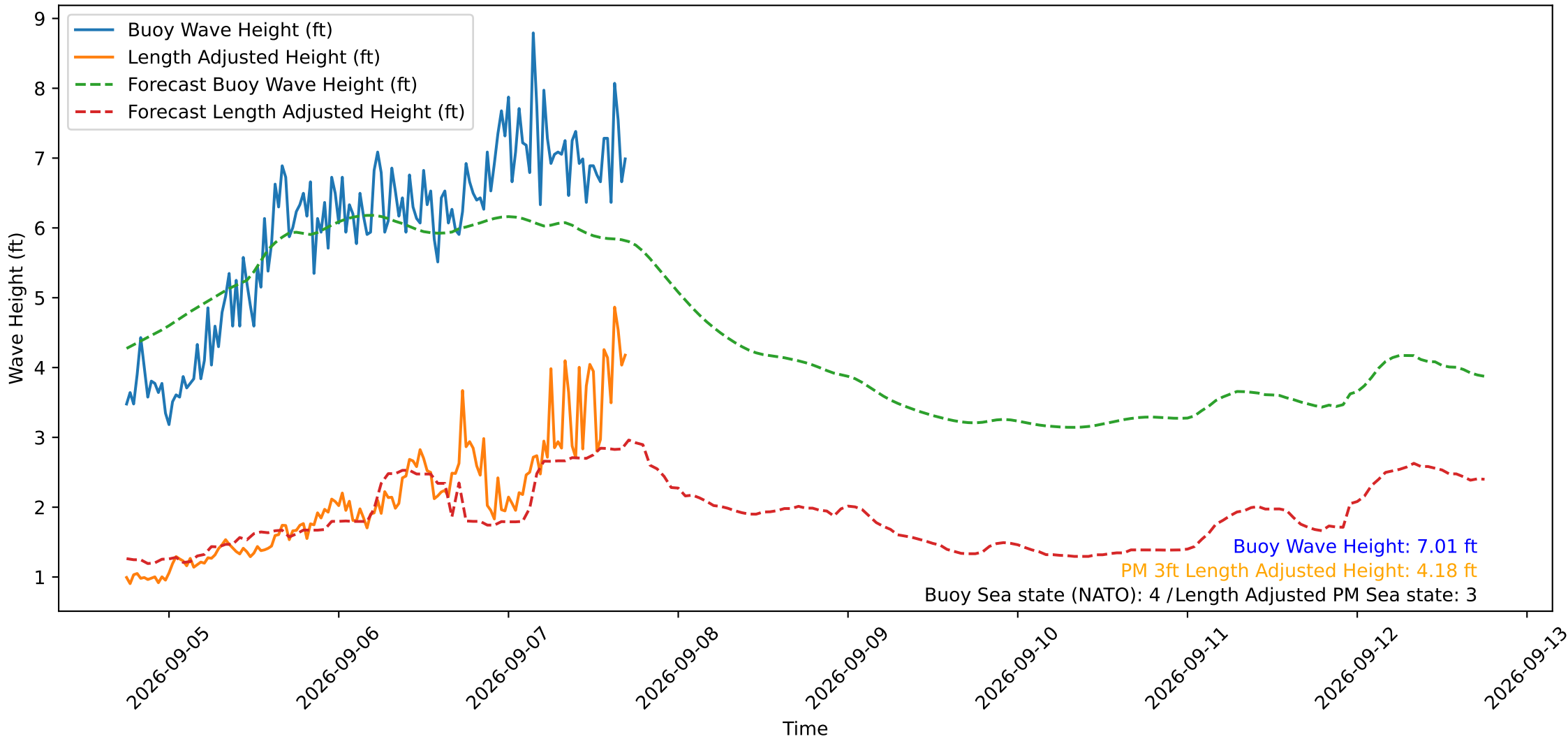
Wave Heights over Time for Green Beach at 2026-09-07 17:31:12
