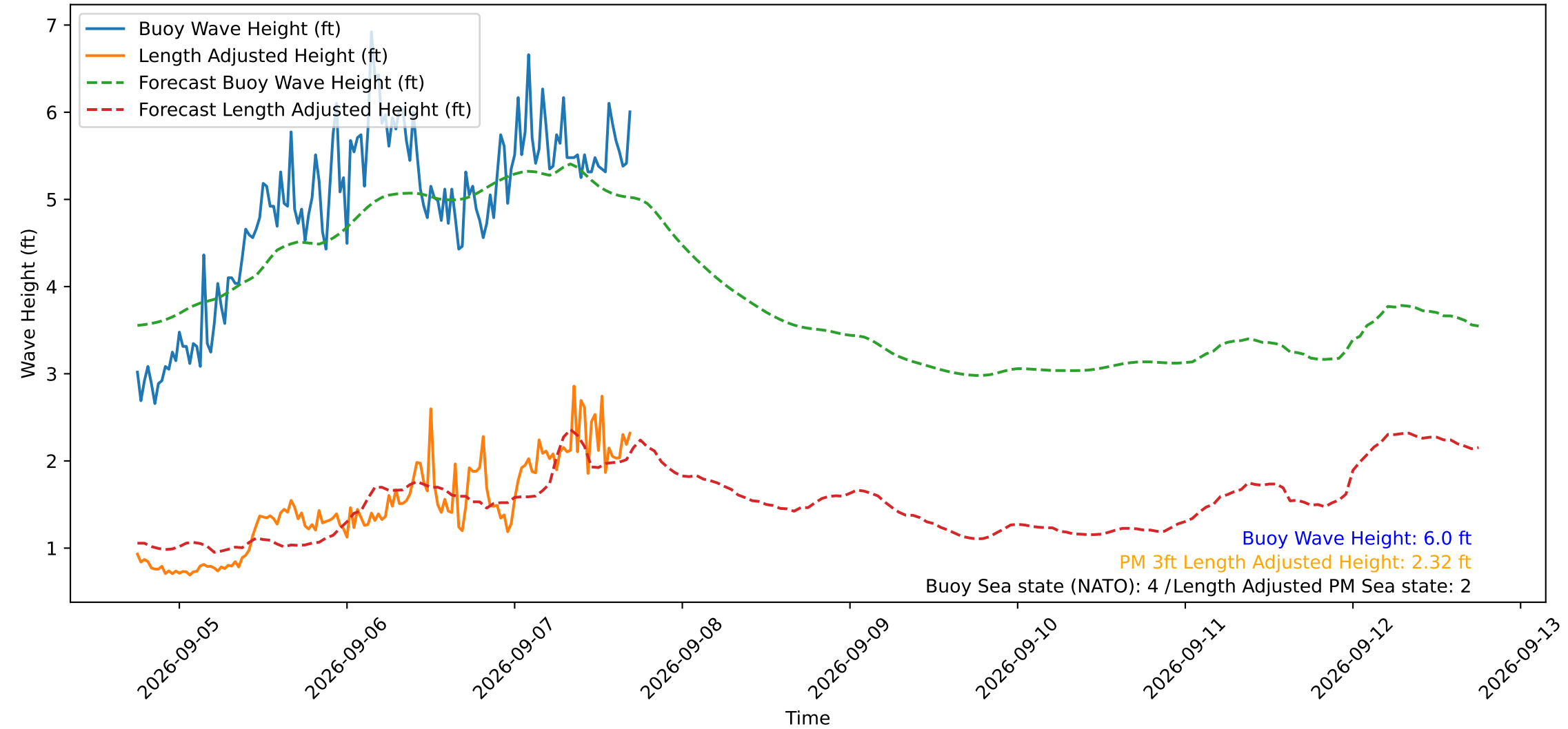
Wave Heights over Time for Red Beach at 2026-09-07 17:30:50
