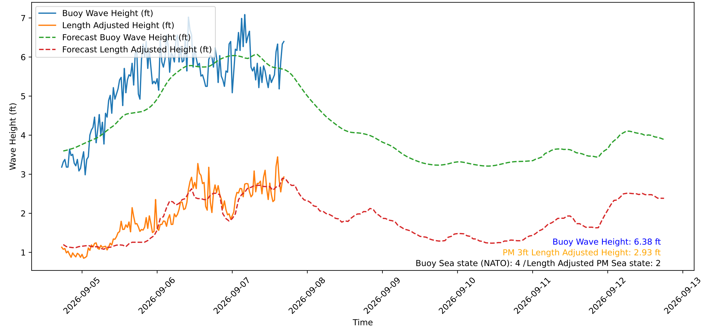
Wave Heights over Time for Oceanside Harbor at 2026-09-07 17:30:30
