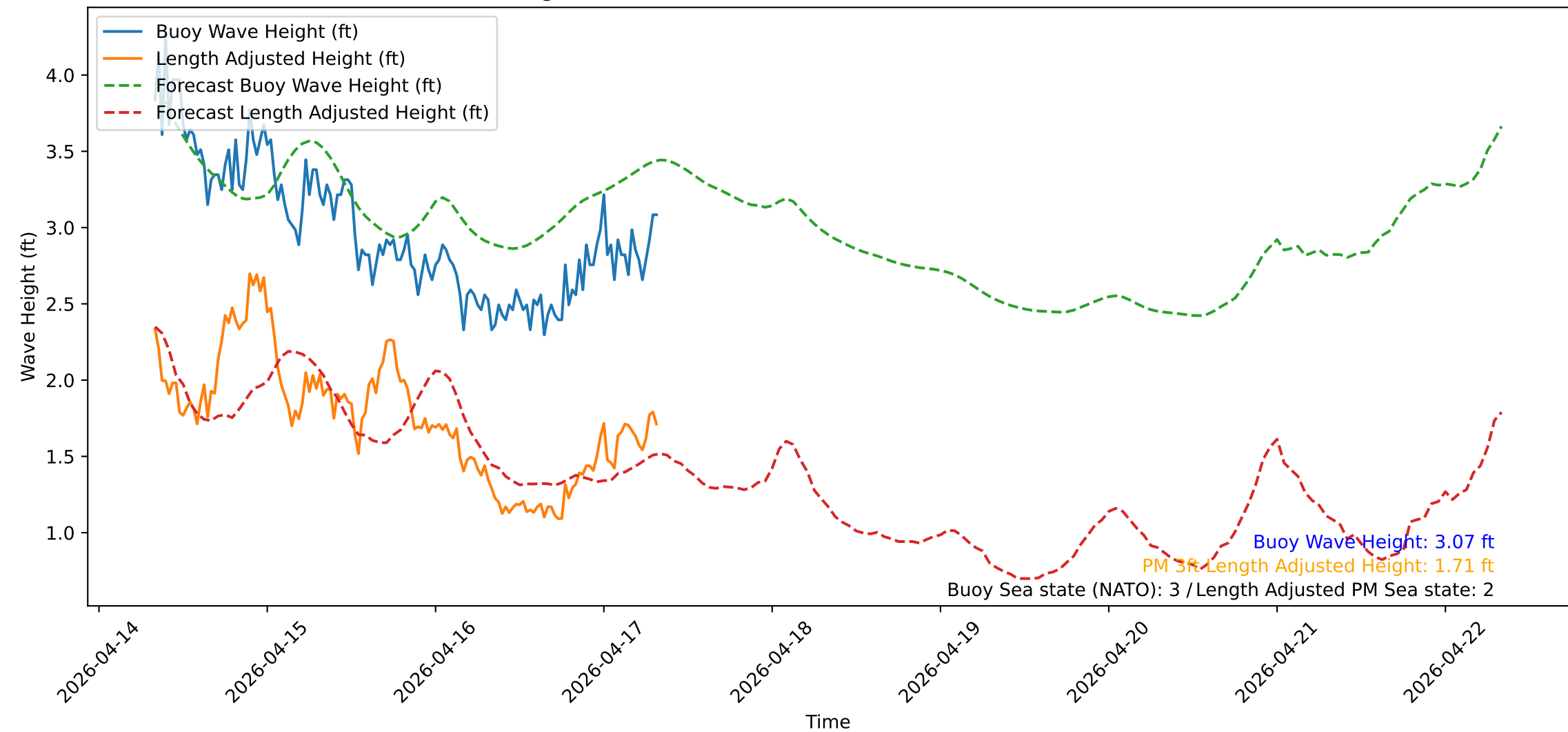
Wave Heights over Time for Oceanside Harbor at 2026-04-17 08:00:32
