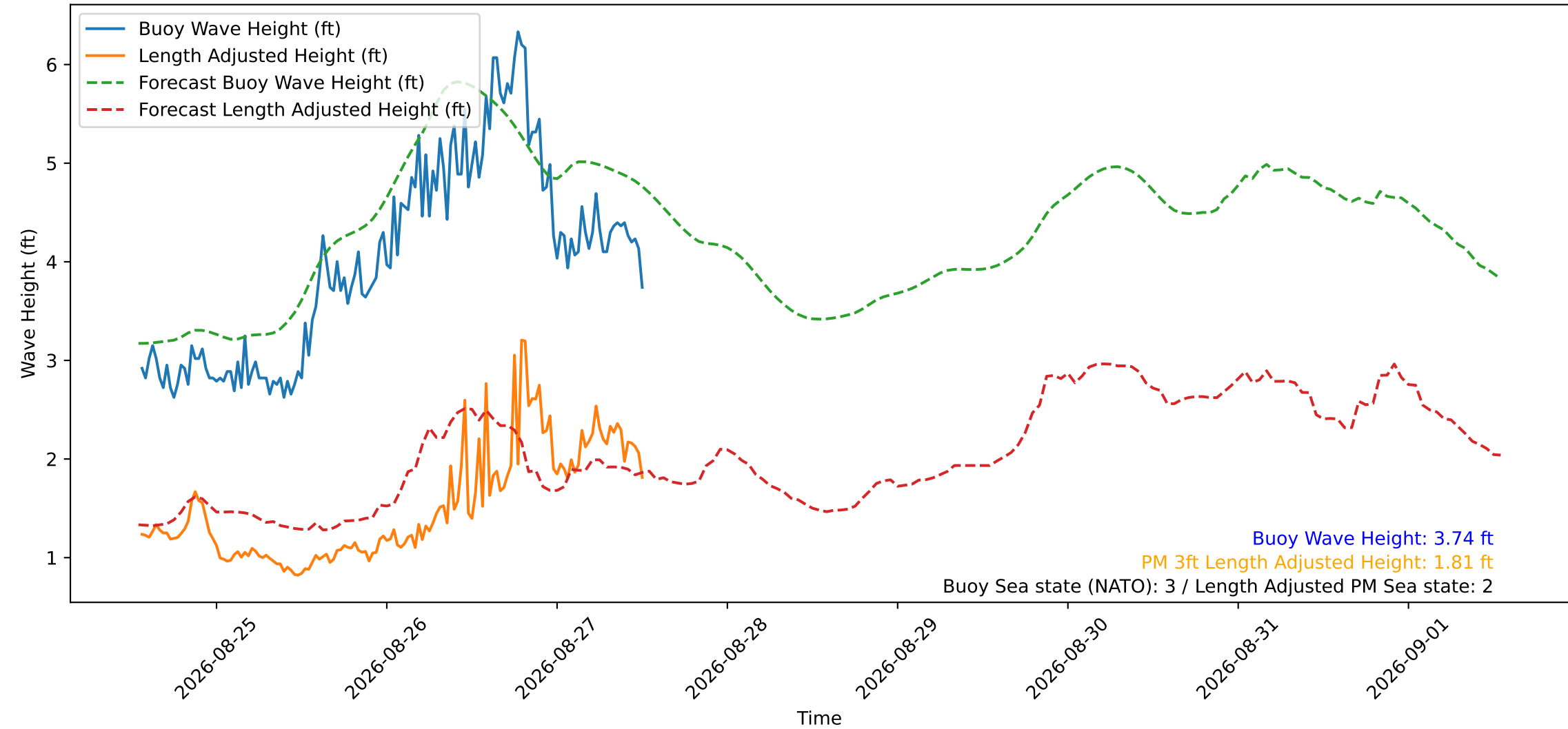
Wave Heights over Time for Green Beach at 2026-08-27 13:01:11
