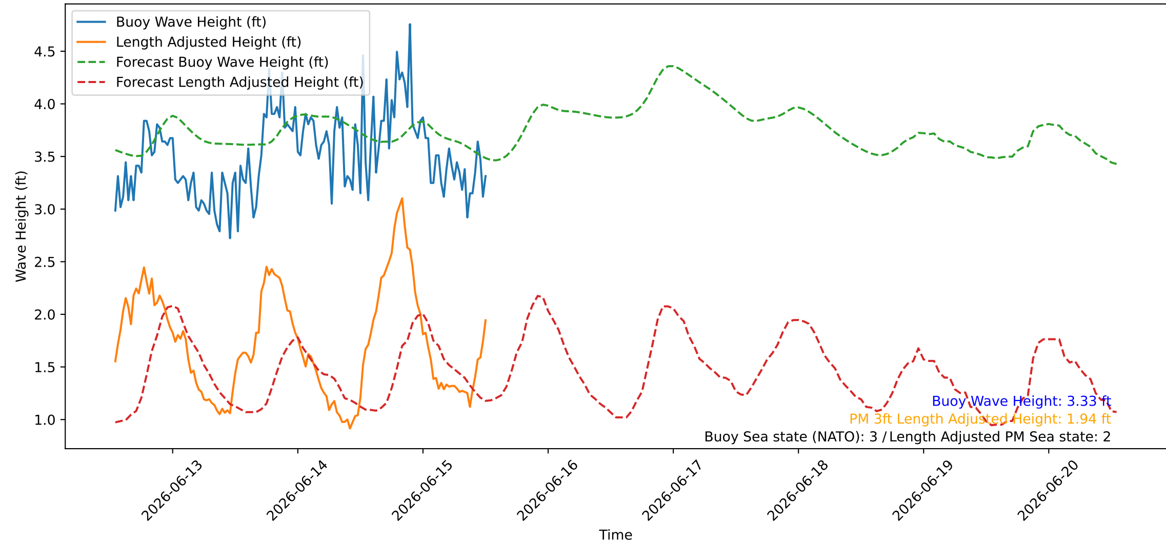
Wave Heights over Time for Red Beach at 2026-06-15 12:40:45
