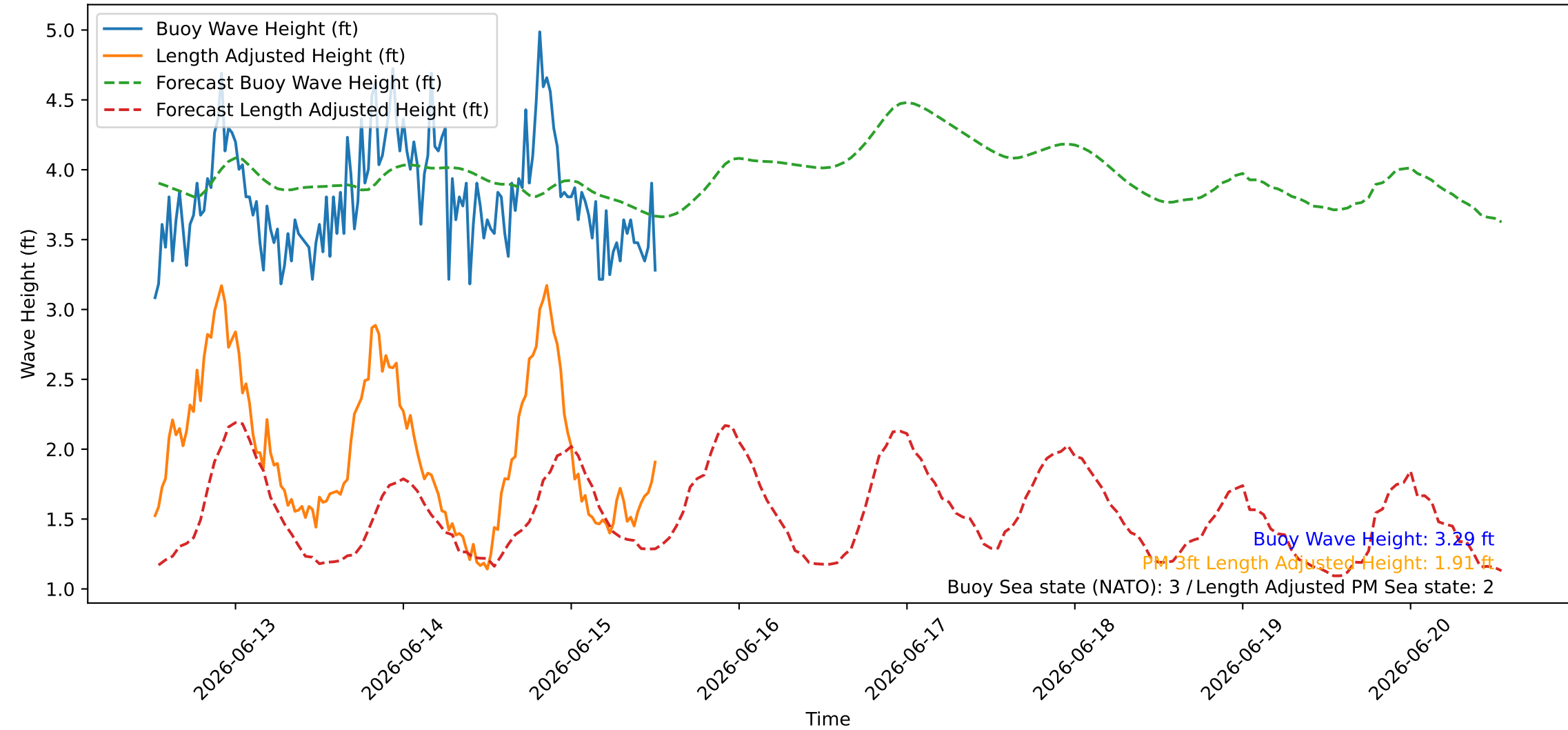
Wave Heights over Time for Oceanside Harbor at 2026-06-15 12:40:25
