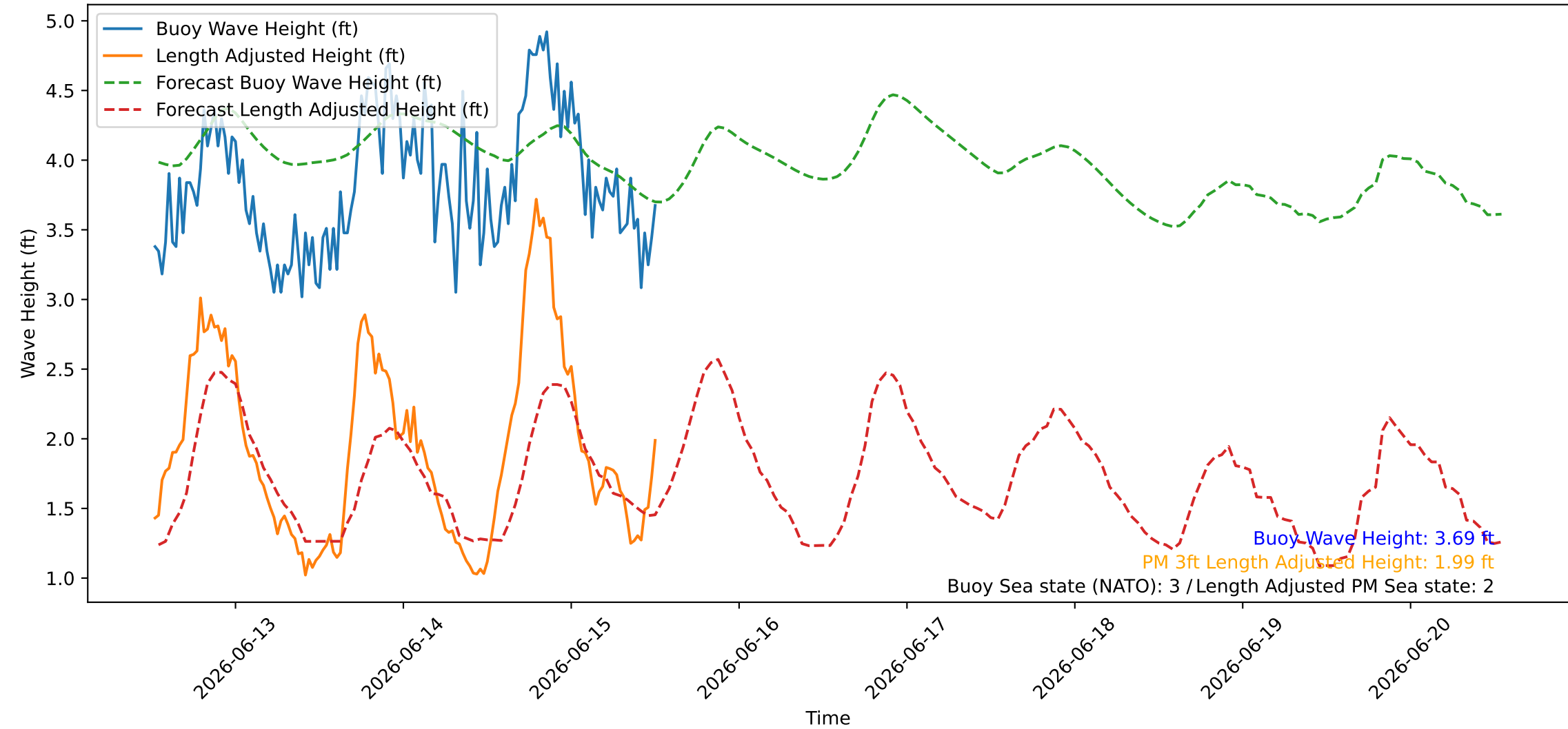
Wave Heights over Time for Green Beach at 2026-06-15 12:41:08
