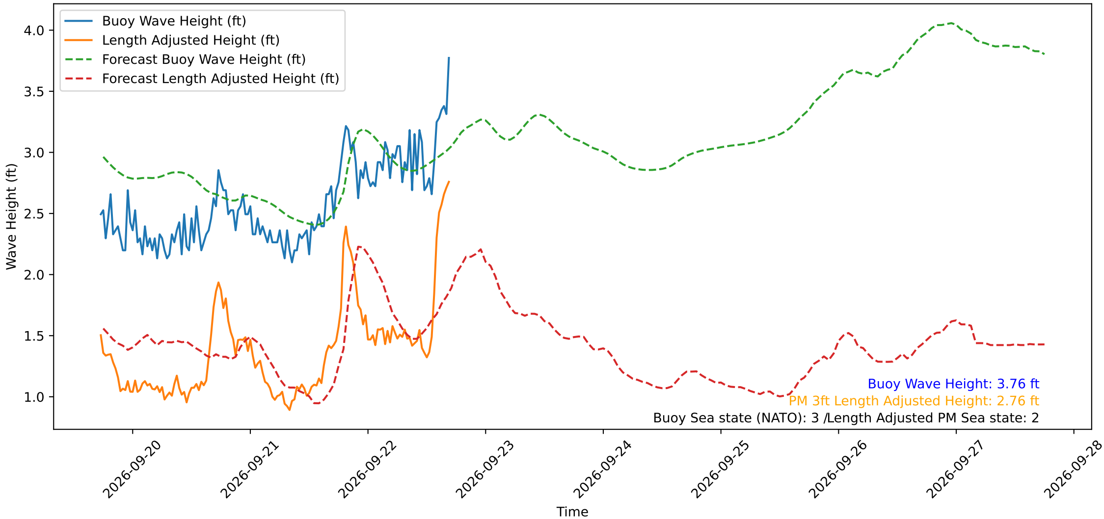
Wave Heights over Time for Oceanside Harbor at 2026-09-22 17:30:30
