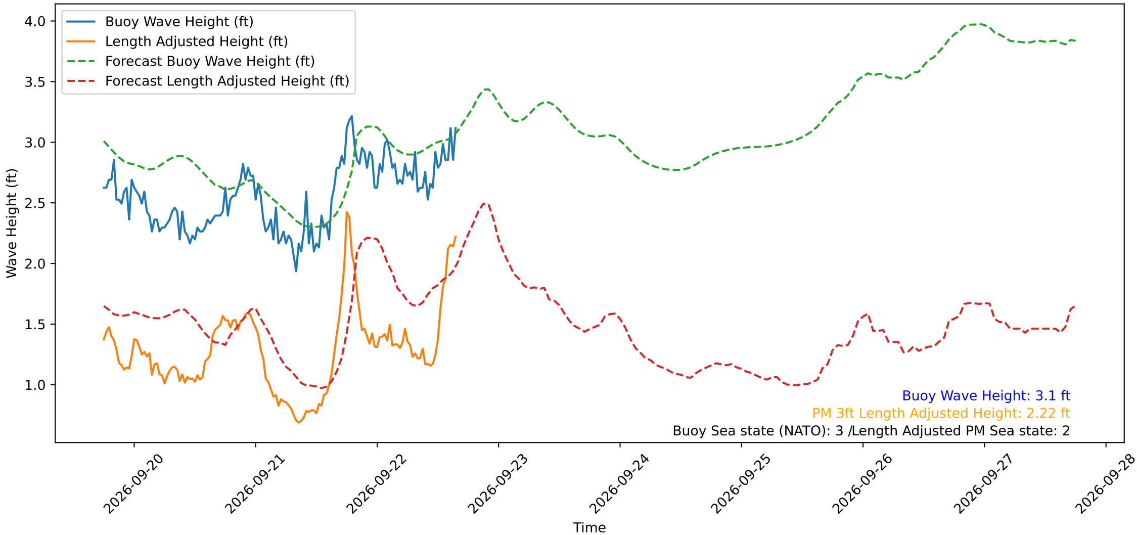
Wave Heights over Time for Green Beach at 2026-09-22 17:31:12
