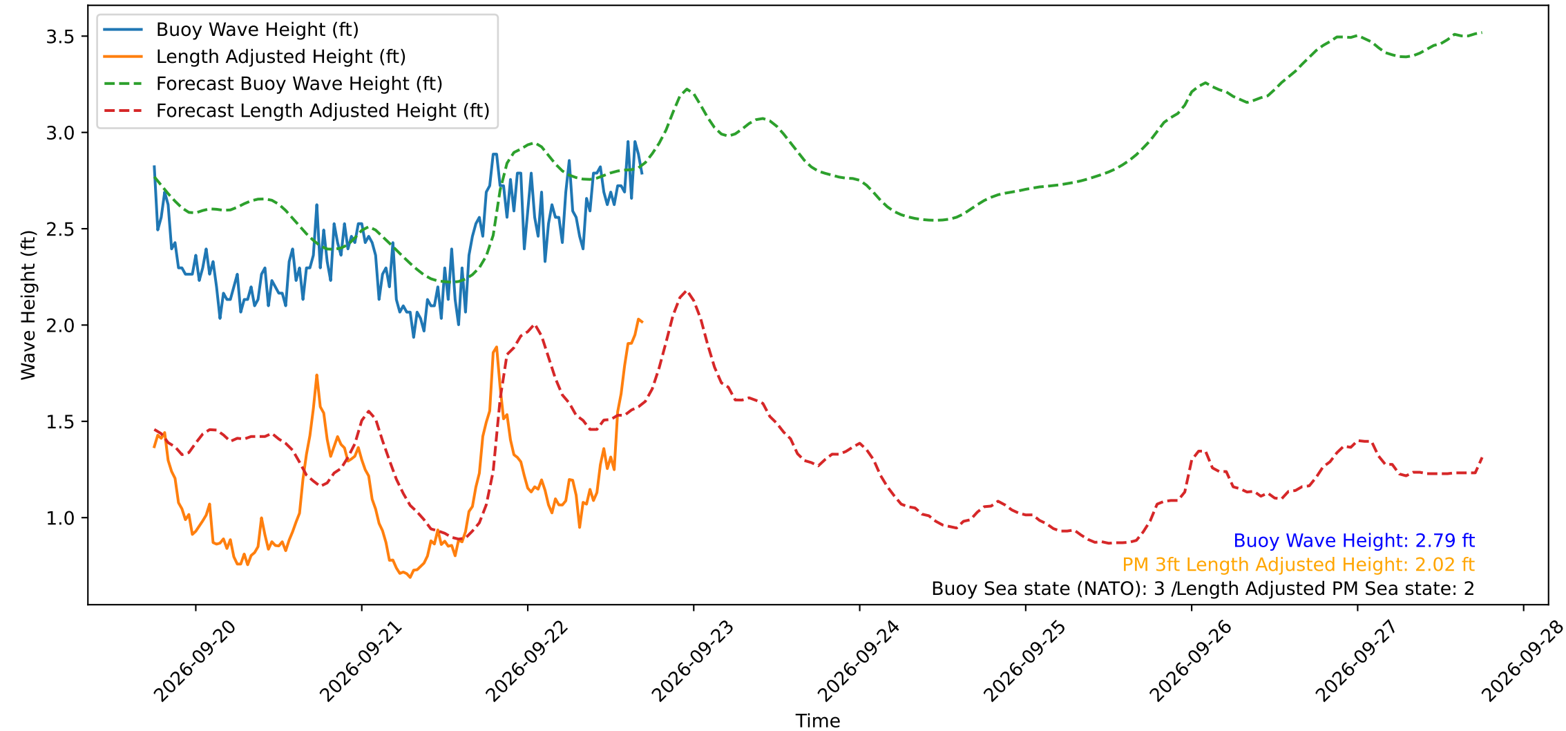
Wave Heights over Time for Red Beach at 2026-09-22 17:30:49
