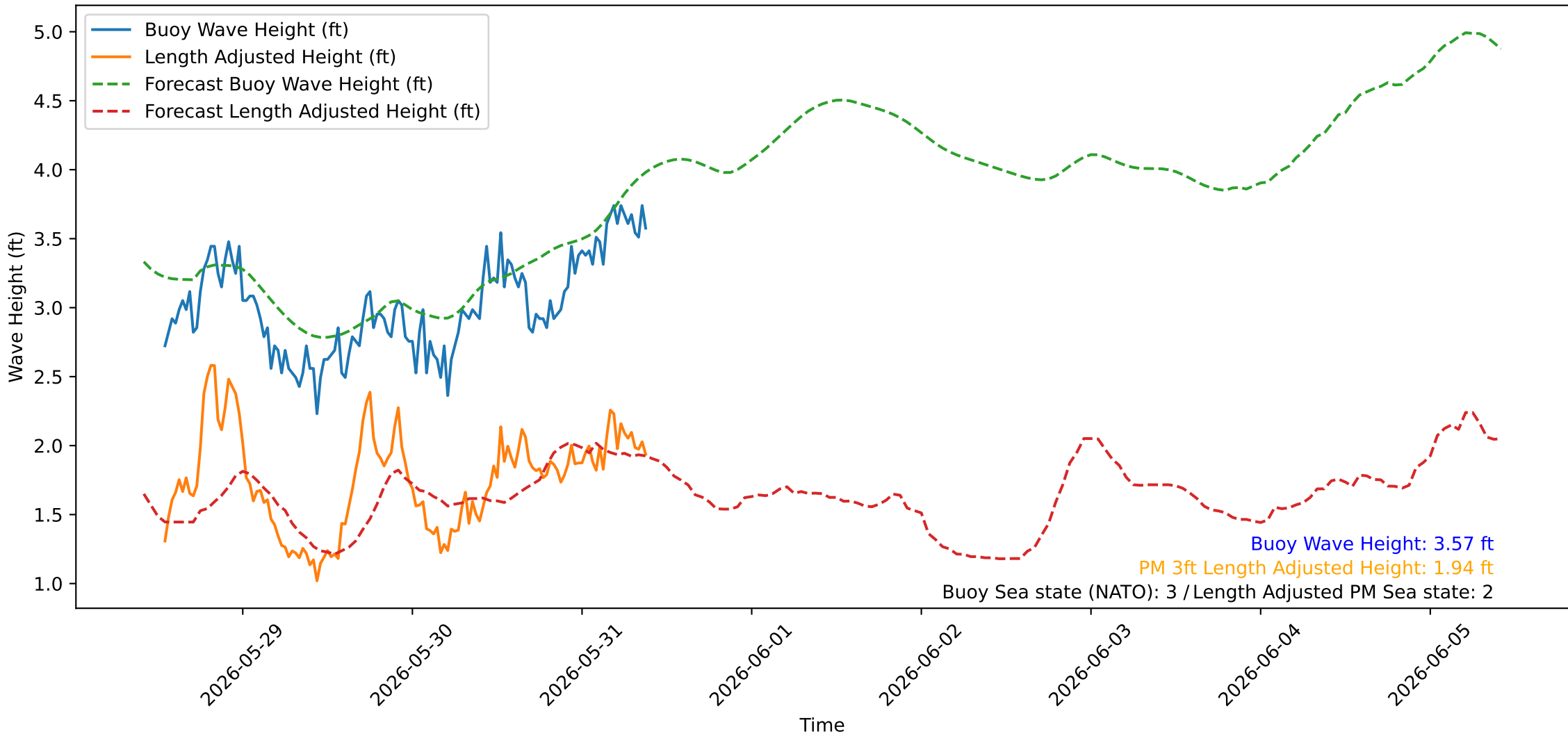
Wave Heights over Time for Oceanside Harbor at 2026-05-31 10:00:26
