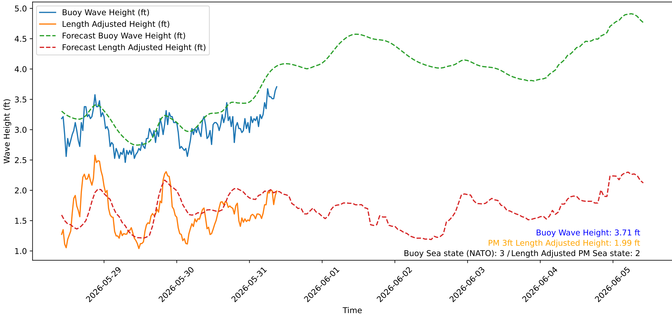
Wave Heights over Time for Green Beach at 2026-05-31 10:01:08
