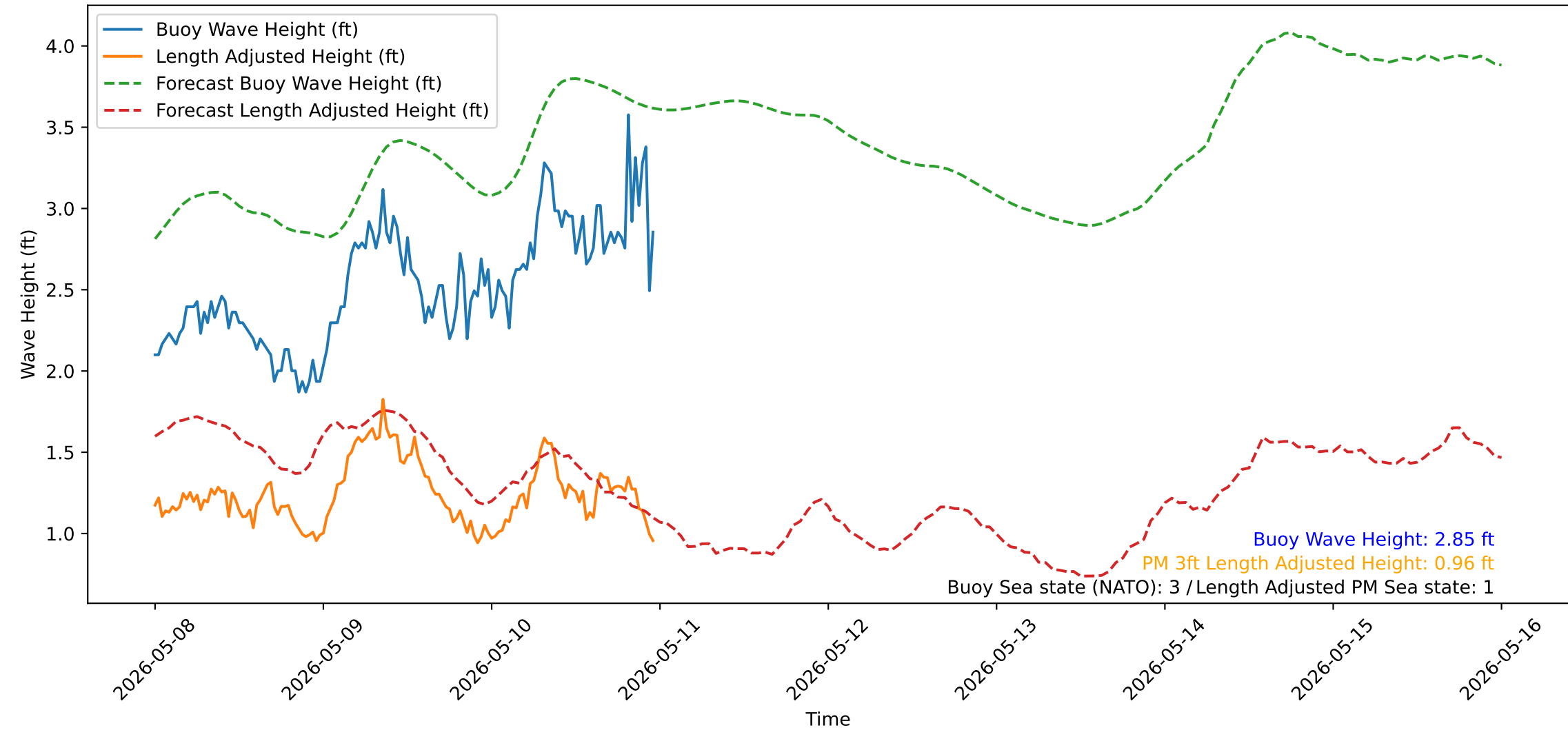
Wave Heights over Time for Oceanside Harbor at 2026-05-10 23:50:31
