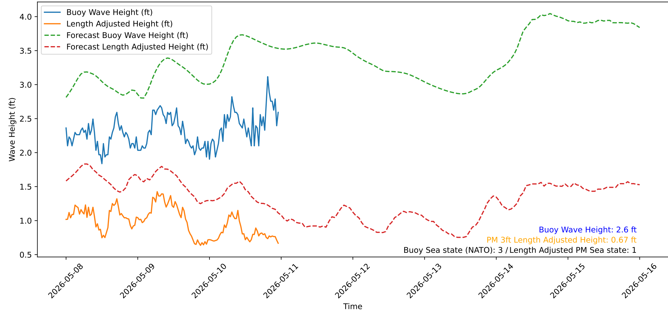
Wave Heights over Time for Green Beach at 2026-05-10 23:51:14
