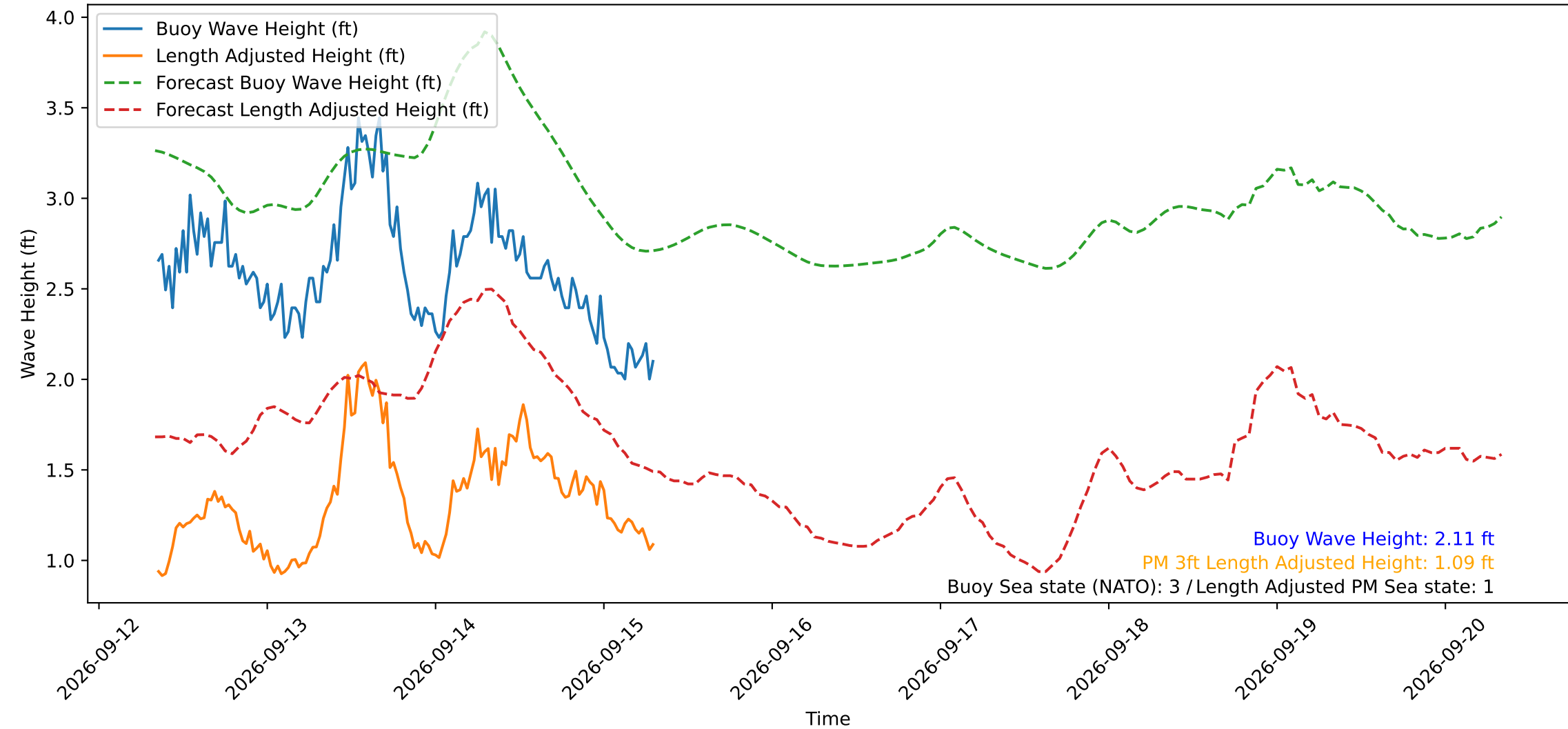
Wave Heights over Time for Red Beach at 2026-09-15 08:00:50
