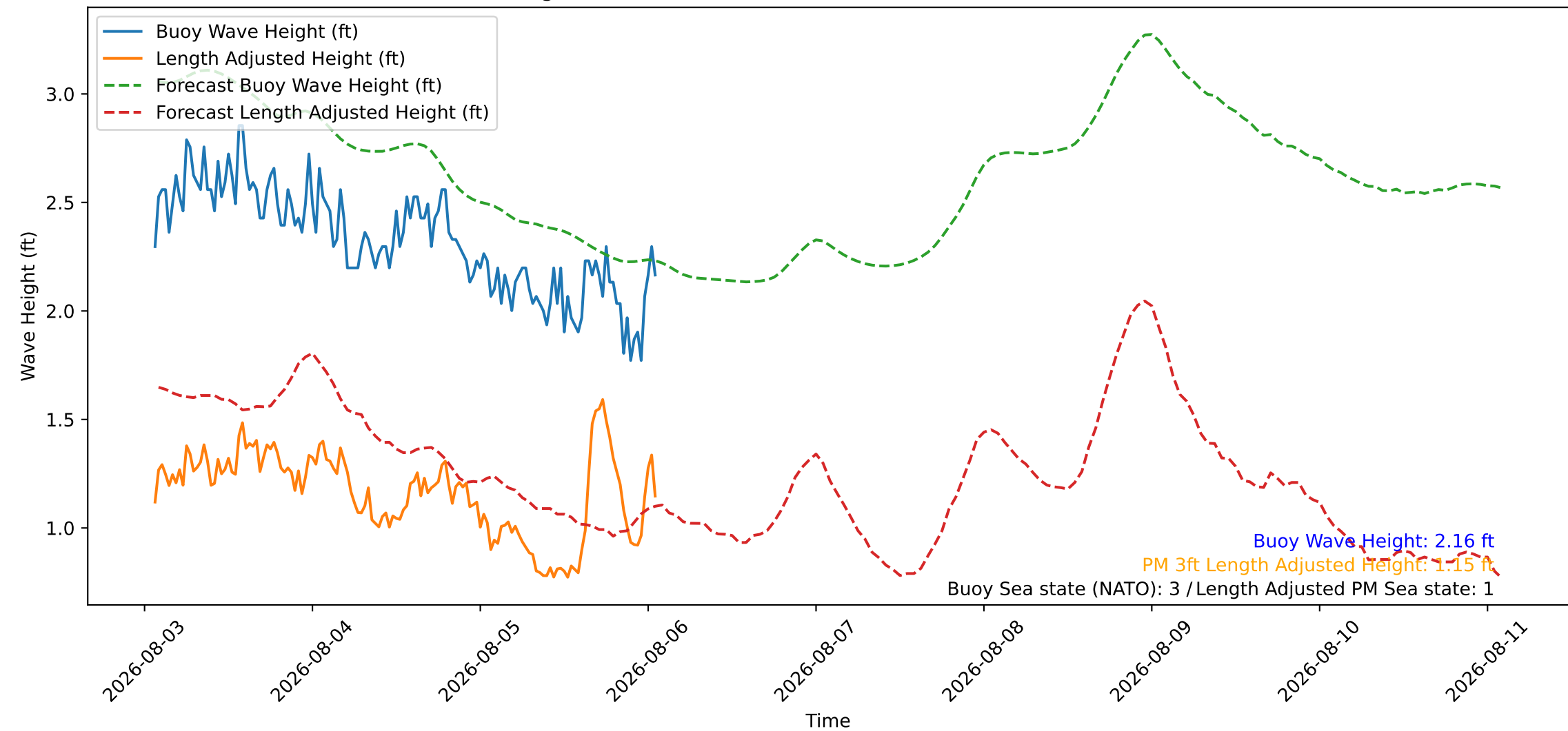
Wave Heights over Time for Oceanside Harbor at 2026-08-06 01:40:26
