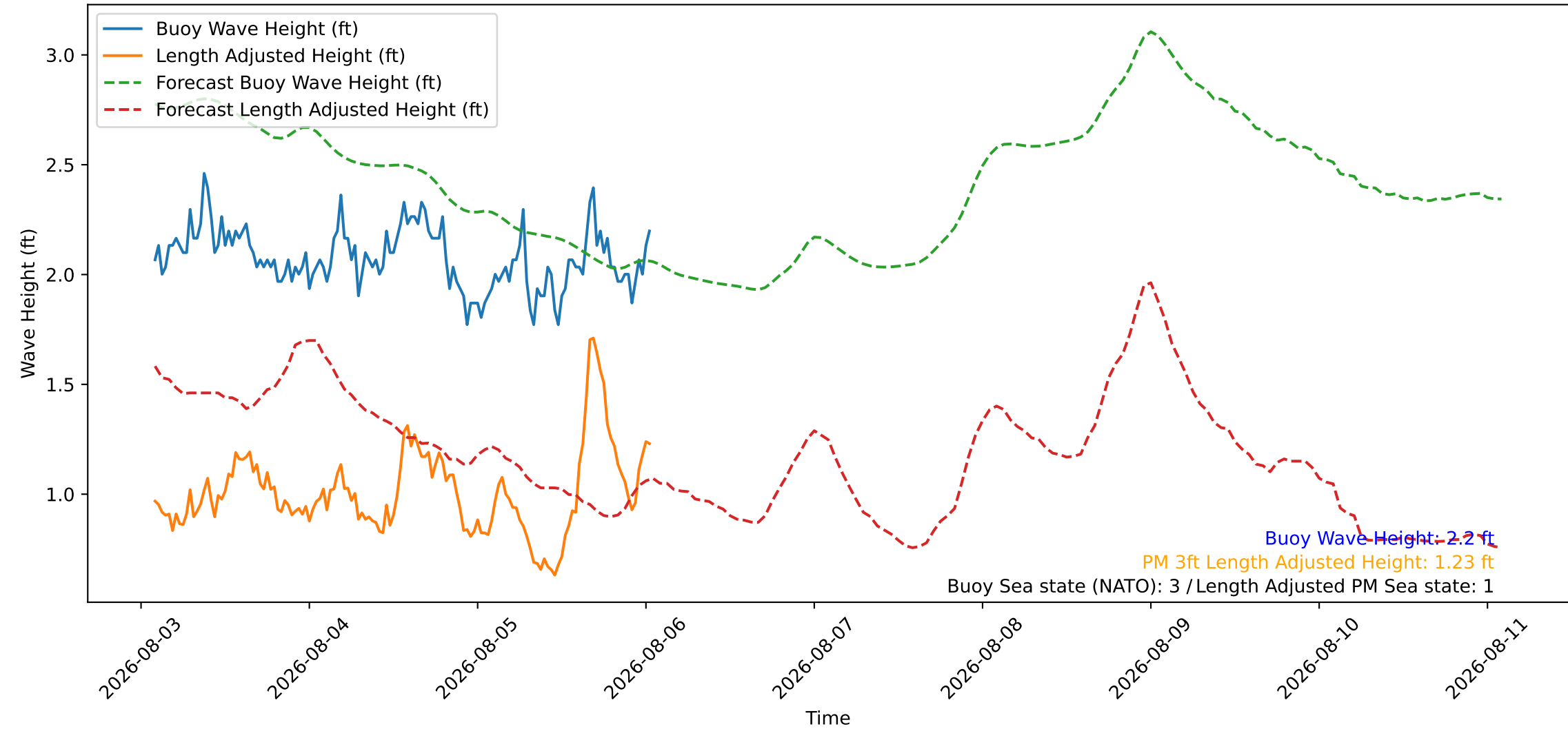
Wave Heights over Time for Red Beach at 2026-08-06 01:40:46
