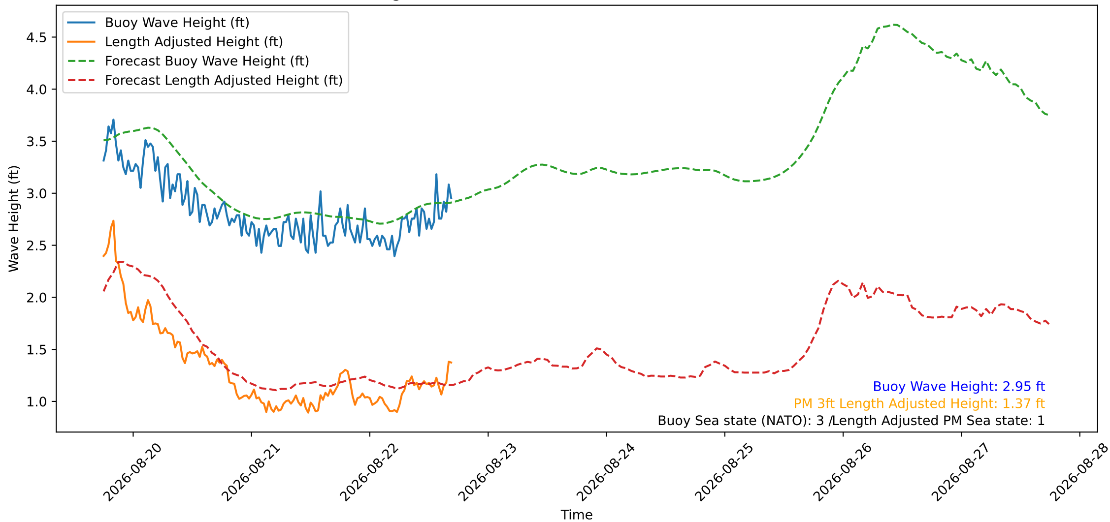
Wave Heights over Time for Green Beach at 2026-08-22 17:31:11
