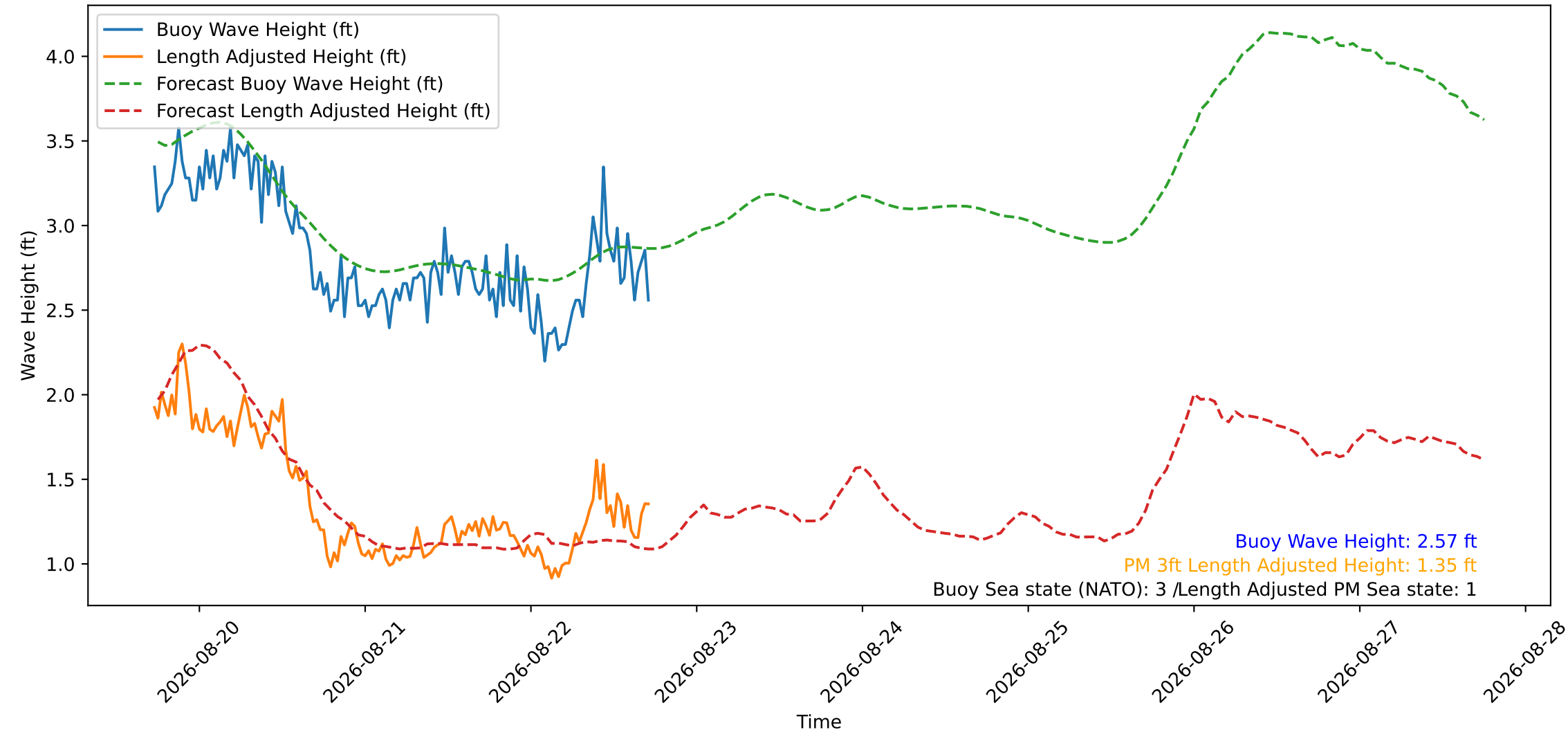
Wave Heights over Time for Oceanside Harbor at 2026-08-22 17:30:29
