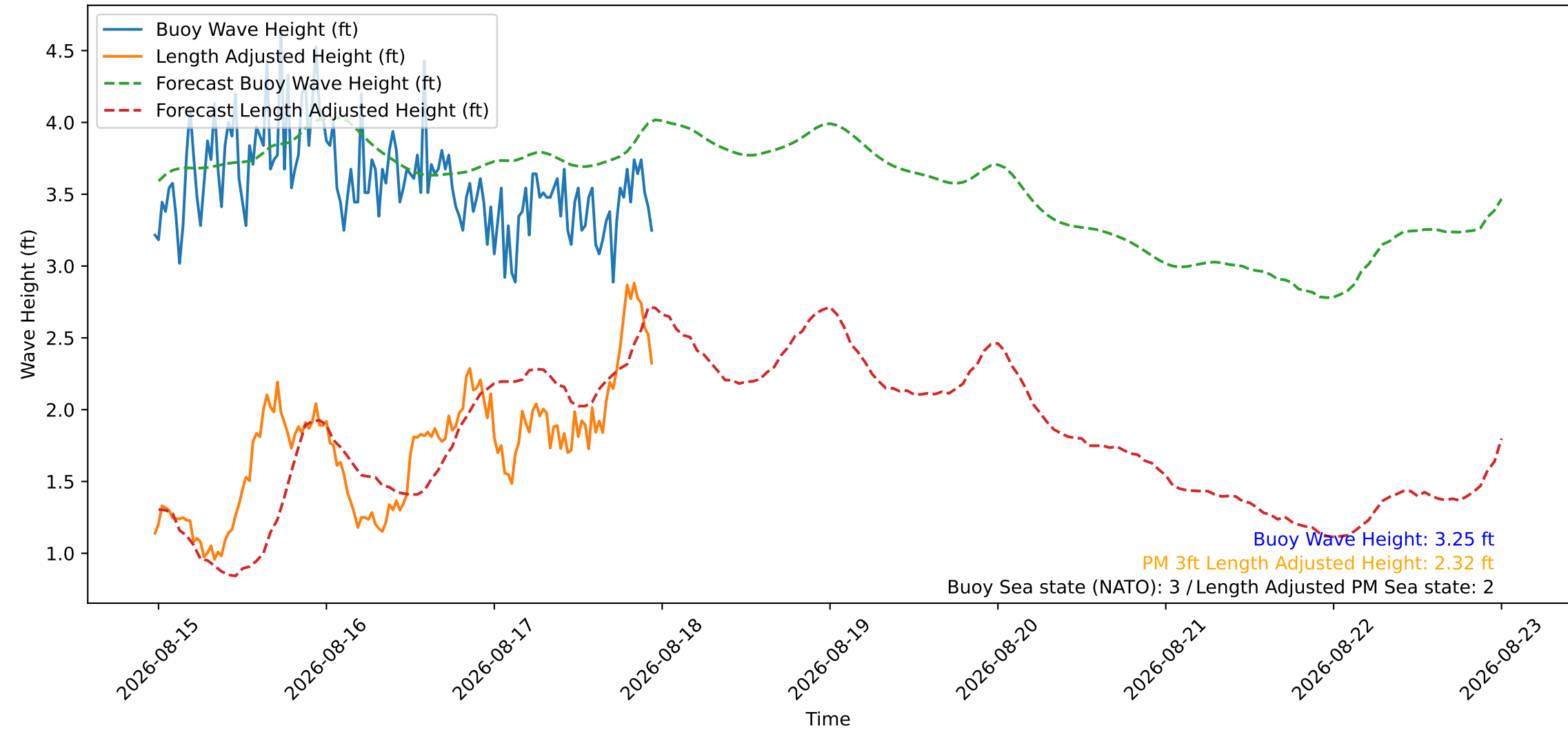
Wave Heights over Time for Oceanside Harbor at 2026-08-17 23:30:26
