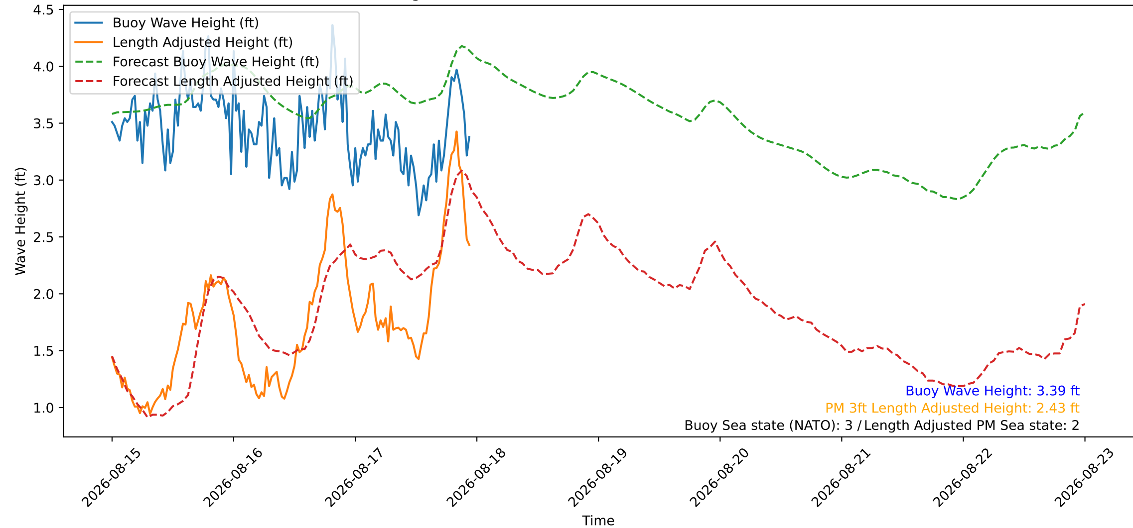
Wave Heights over Time for Green Beach at 2026-08-17 23:31:08
