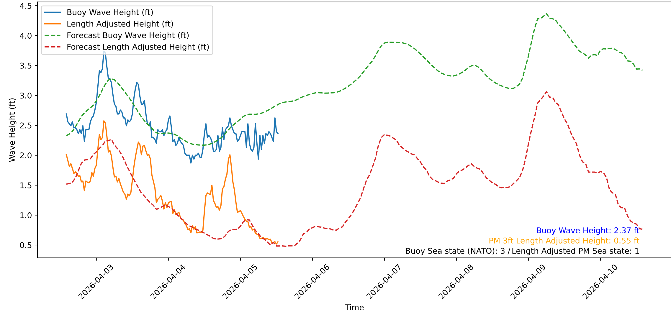
Wave Heights over Time for Red Beach at 2026-04-05 13:30:48
