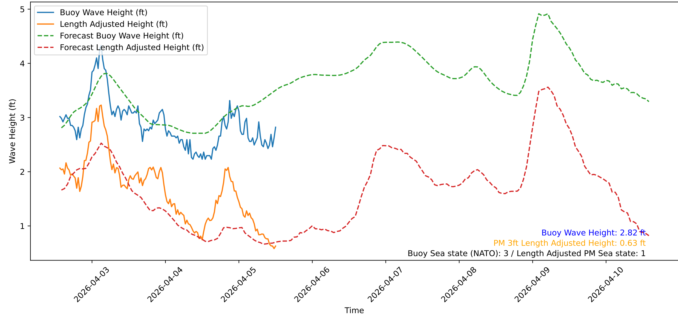
Wave Heights over Time for Green Beach at 2026-04-05 13:31:10
