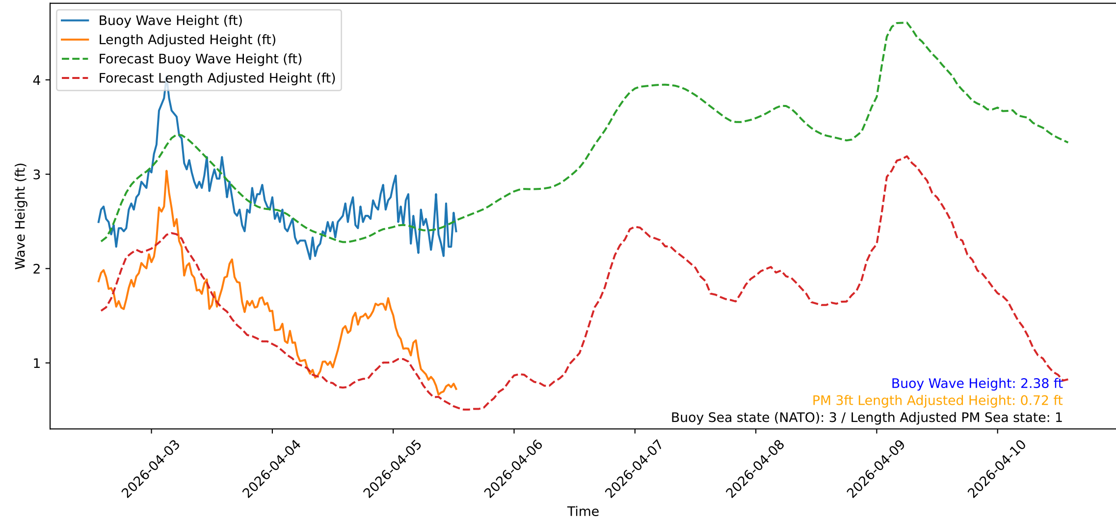
Wave Heights over Time for Oceanside Harbor at 2026-04-05 13:30:32
