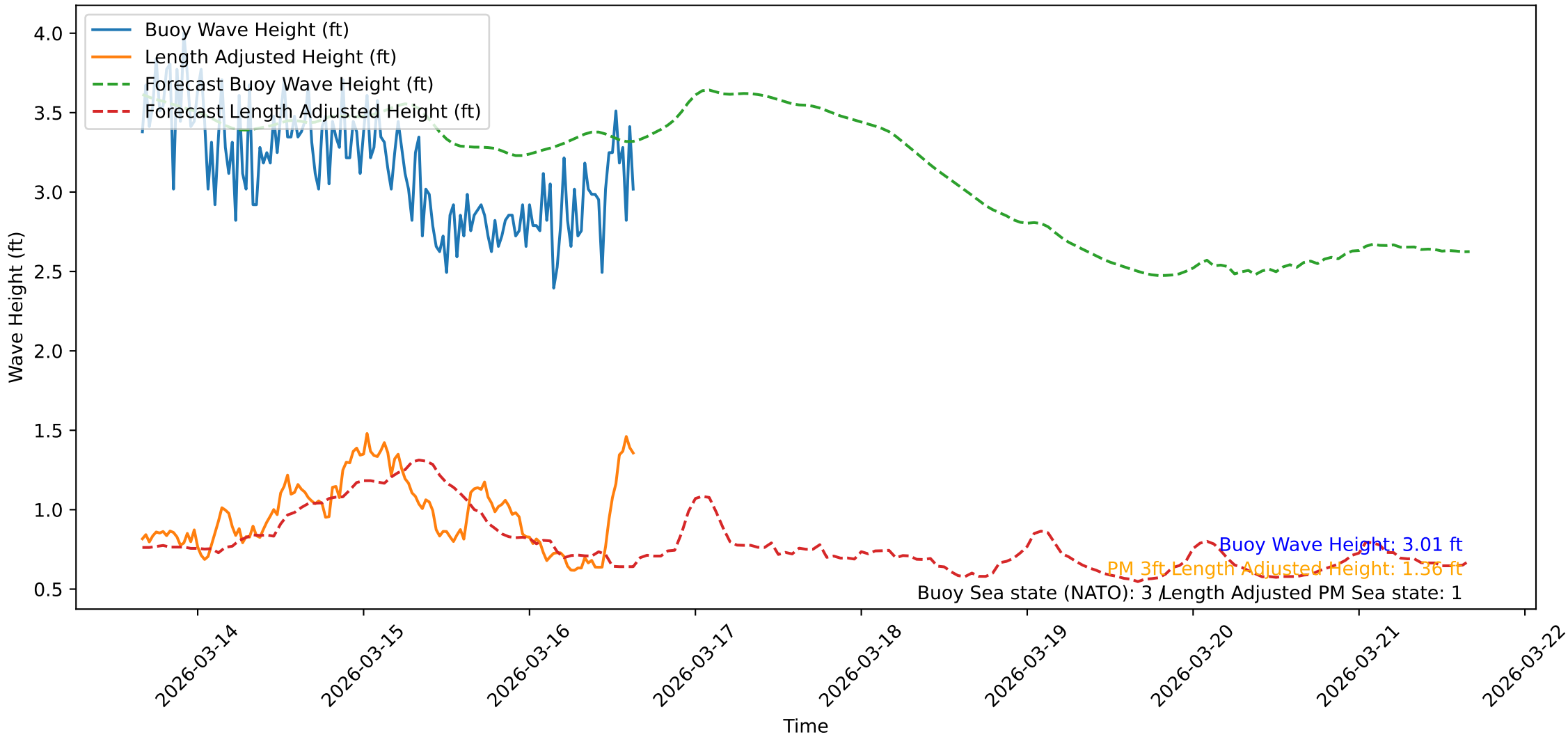
Wave Heights over Time for Oceanside Harbor at 2026-03-16 16:00:41
