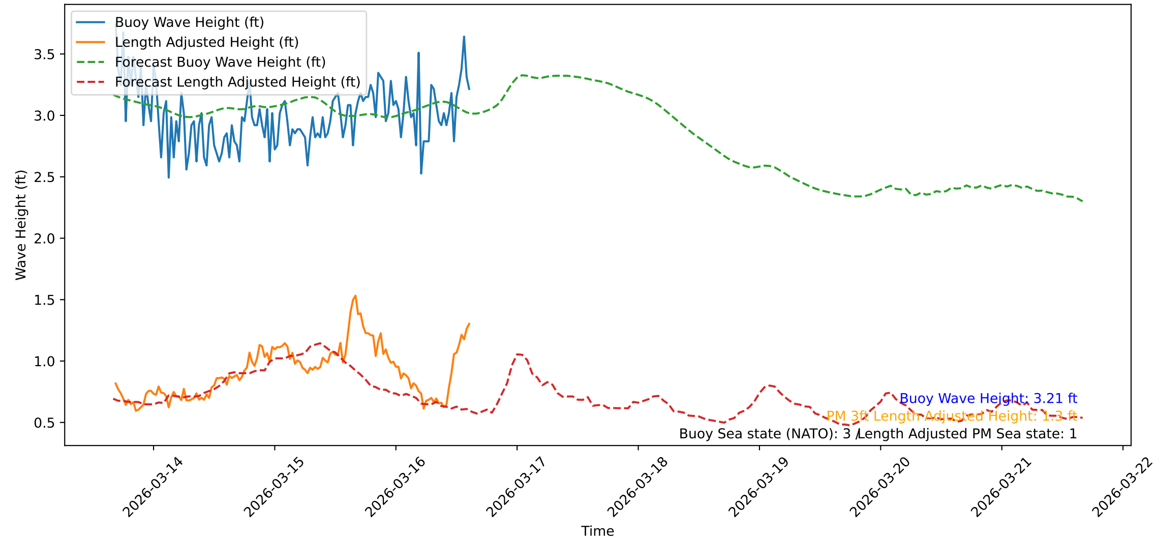
Wave Heights over Time for Red Beach at 2026-03-16 16:01:05
