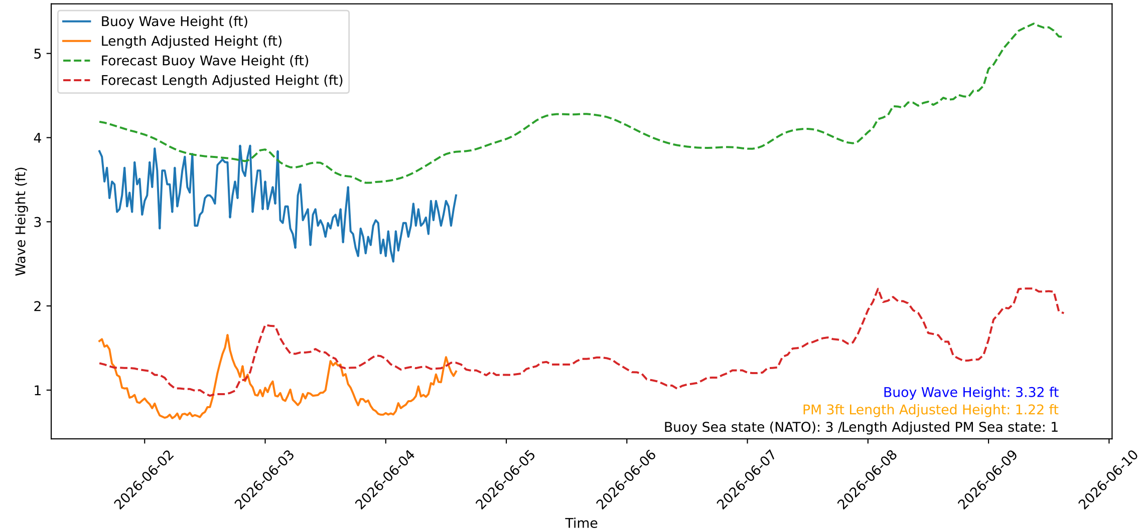
Wave Heights over Time for Red Beach at 2026-06-04 14:50:47
