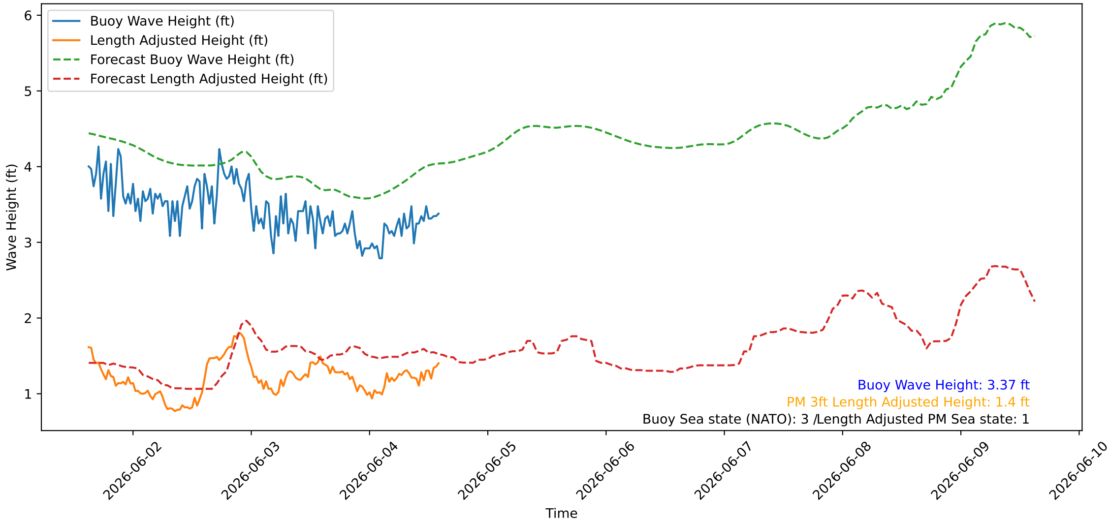
Wave Heights over Time for Green Beach at 2026-06-04 14:51:09
