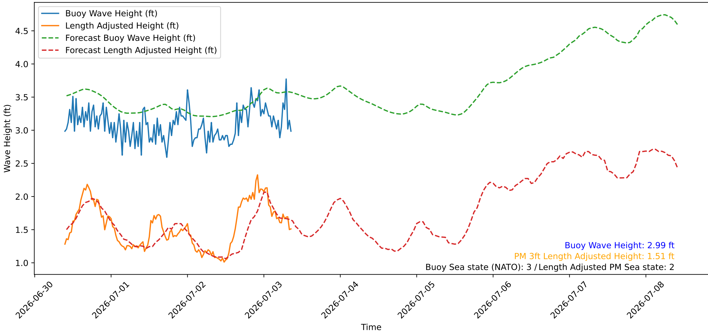
Wave Heights over Time for Oceanside Harbor at 2026-07-03 09:30:27
