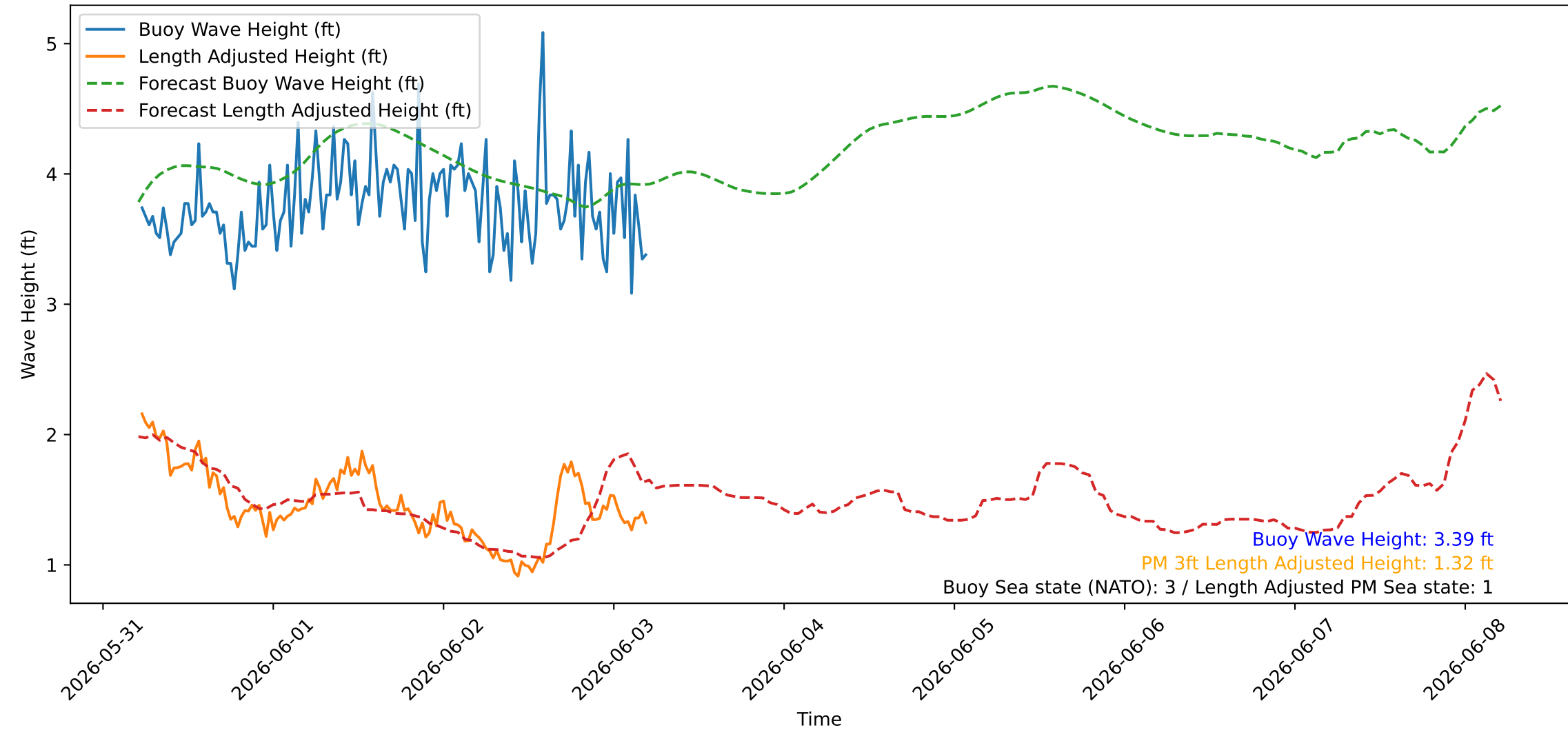
Wave Heights over Time for Oceanside Harbor at 2026-06-03 05:20:26
