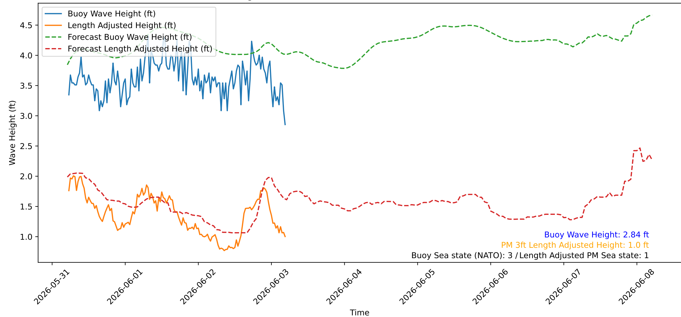
Wave Heights over Time for Green Beach at 2026-06-03 05:21:09
