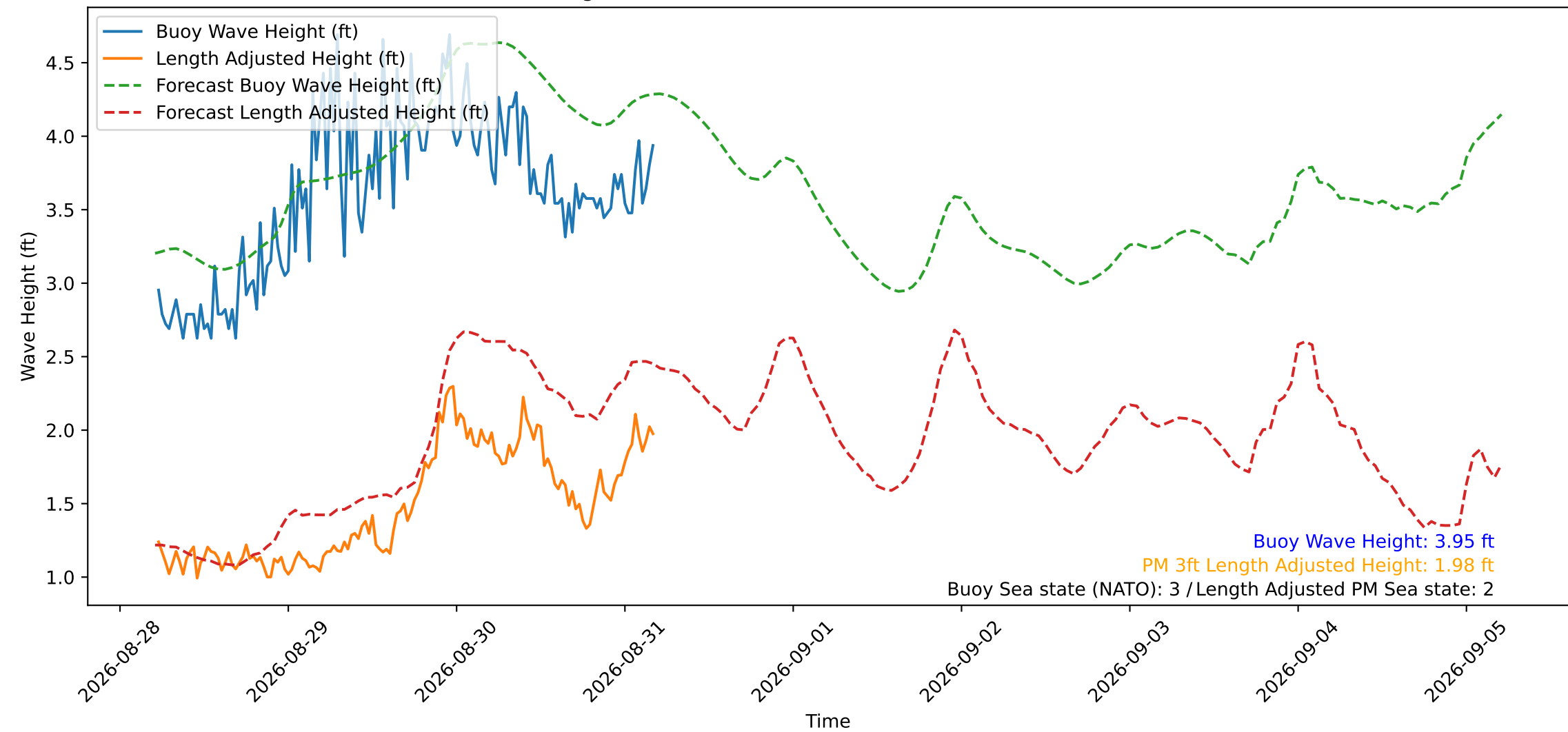
Wave Heights over Time for Red Beach at 2026-08-31 05:00:49
