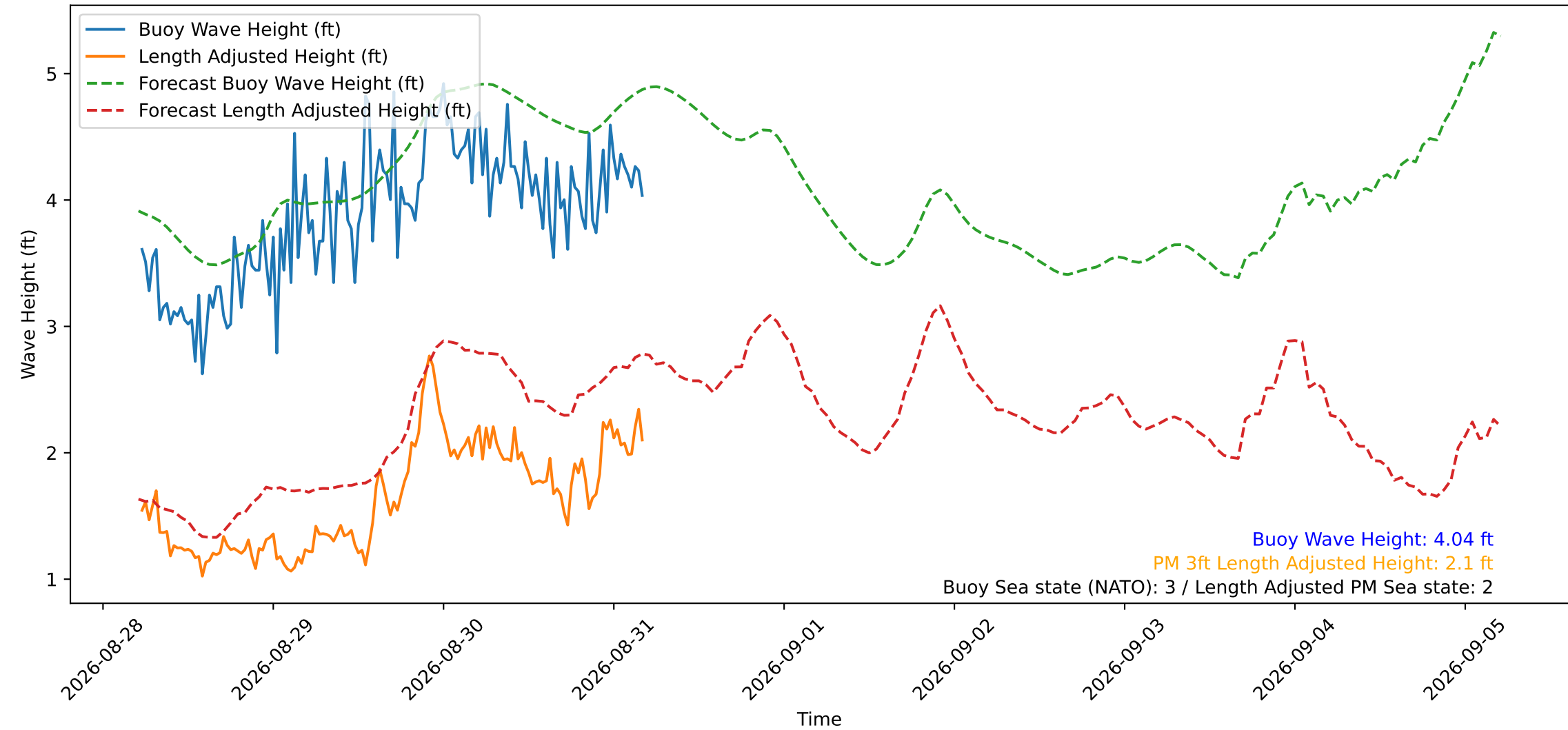
Wave Heights over Time for Green Beach at 2026-08-31 05:01:12
