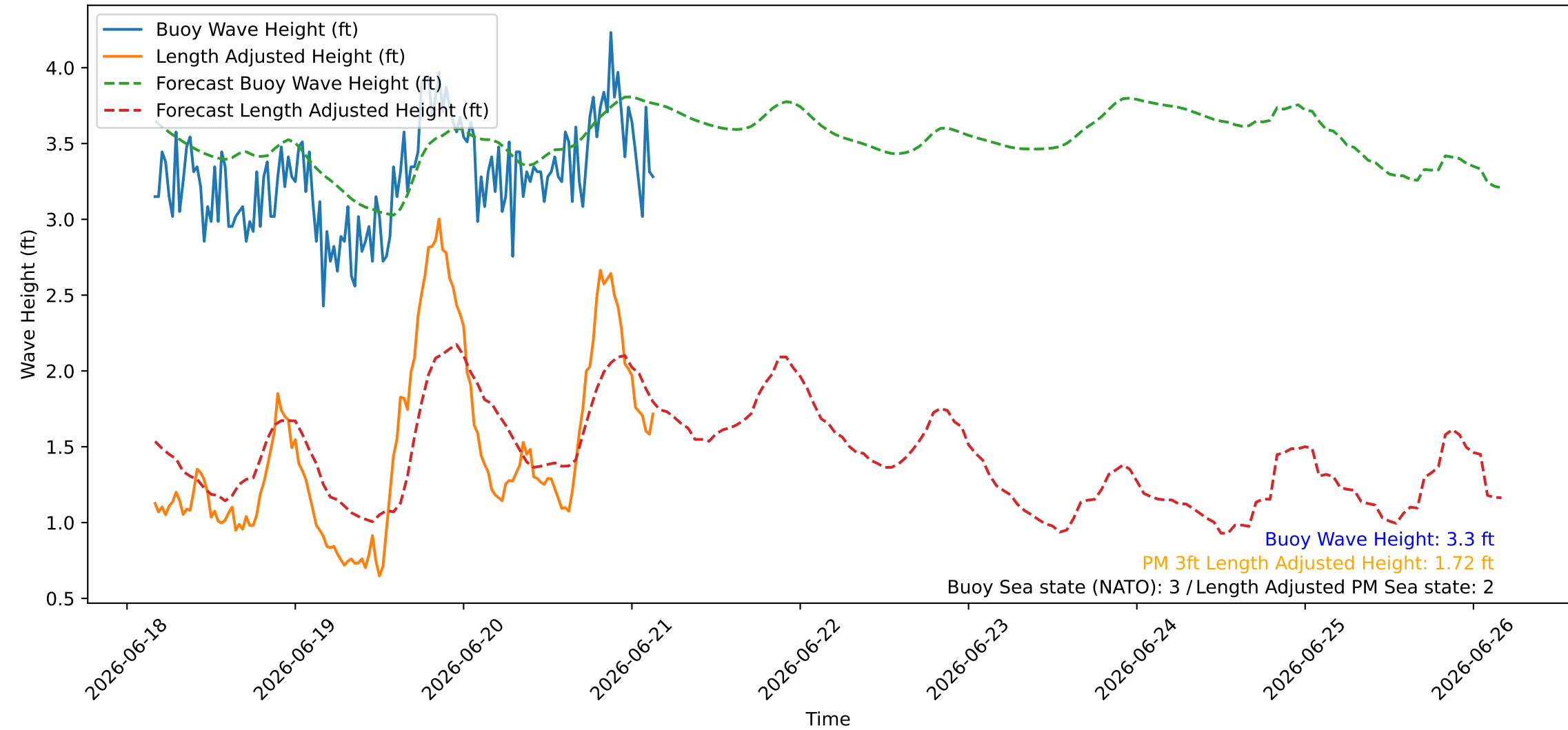
Wave Heights over Time for Green Beach at 2026-06-21 03:51:08
