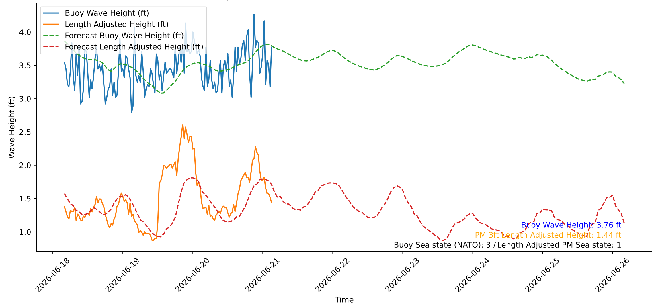
Wave Heights over Time for Oceanside Harbor at 2026-06-21 03:50:26
