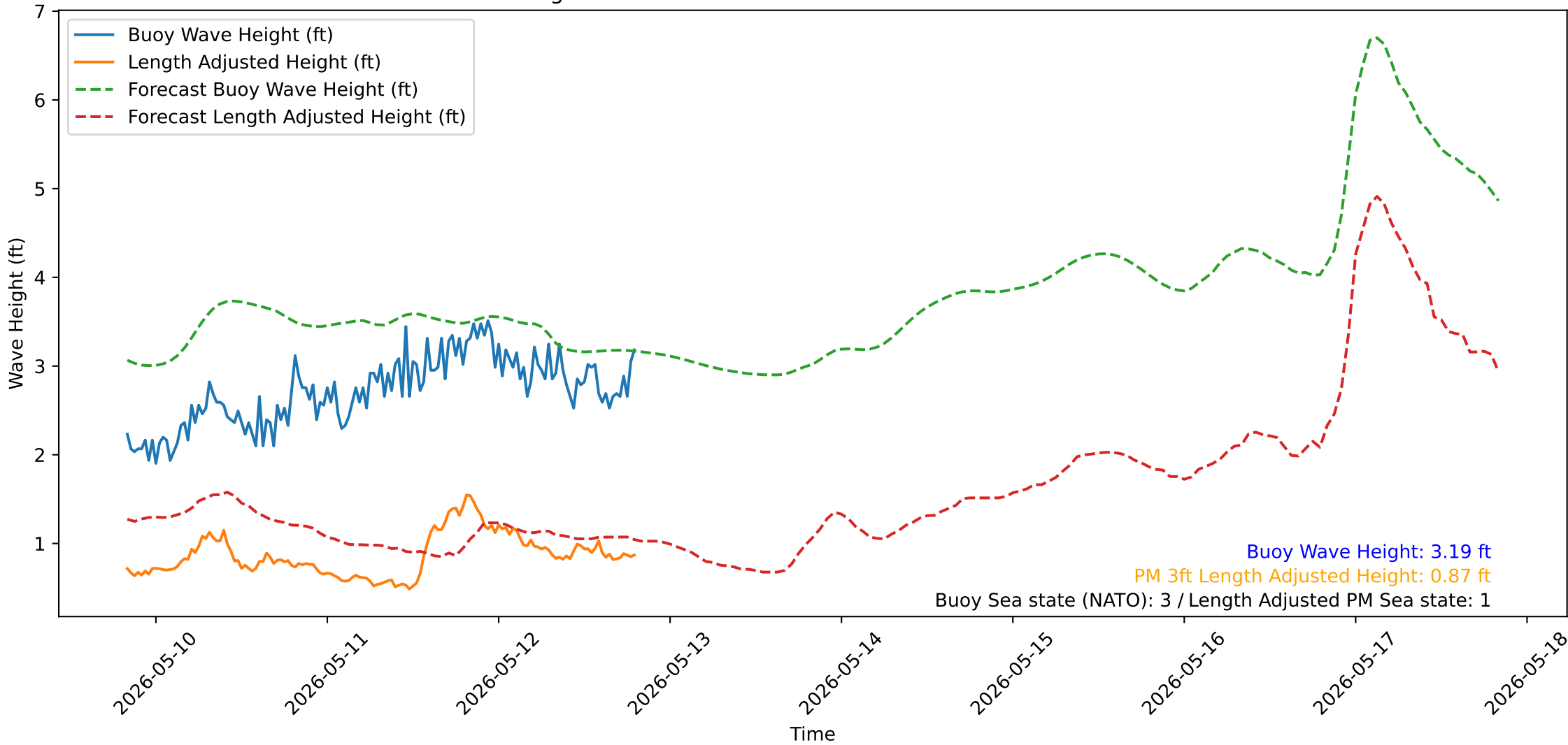
Wave Heights over Time for Green Beach at 2026-05-12 20:01:14
