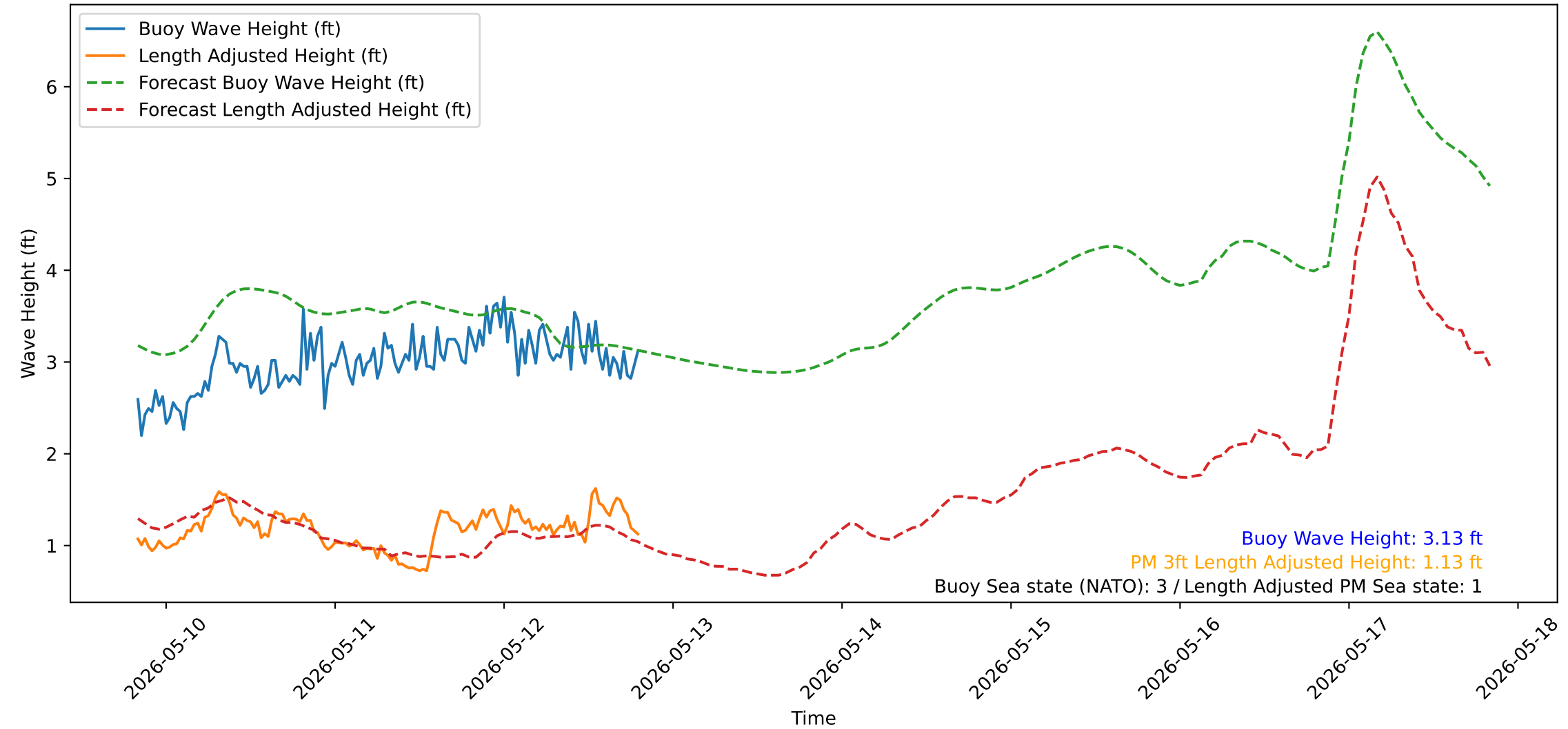
Wave Heights over Time for Oceanside Harbor at 2026-05-12 20:00:31
