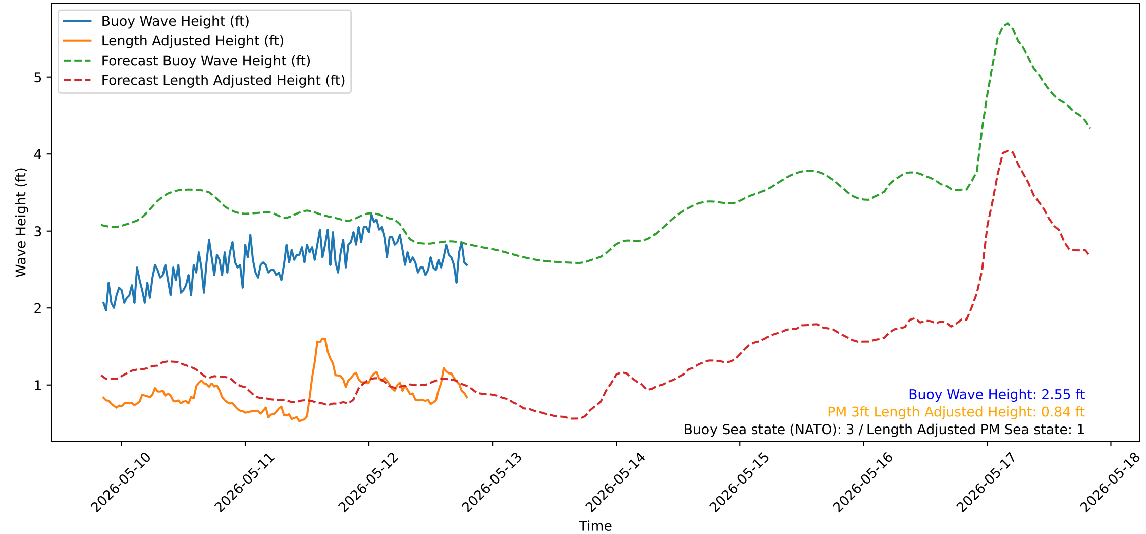
Wave Heights over Time for Red Beach at 2026-05-12 20:00:50
