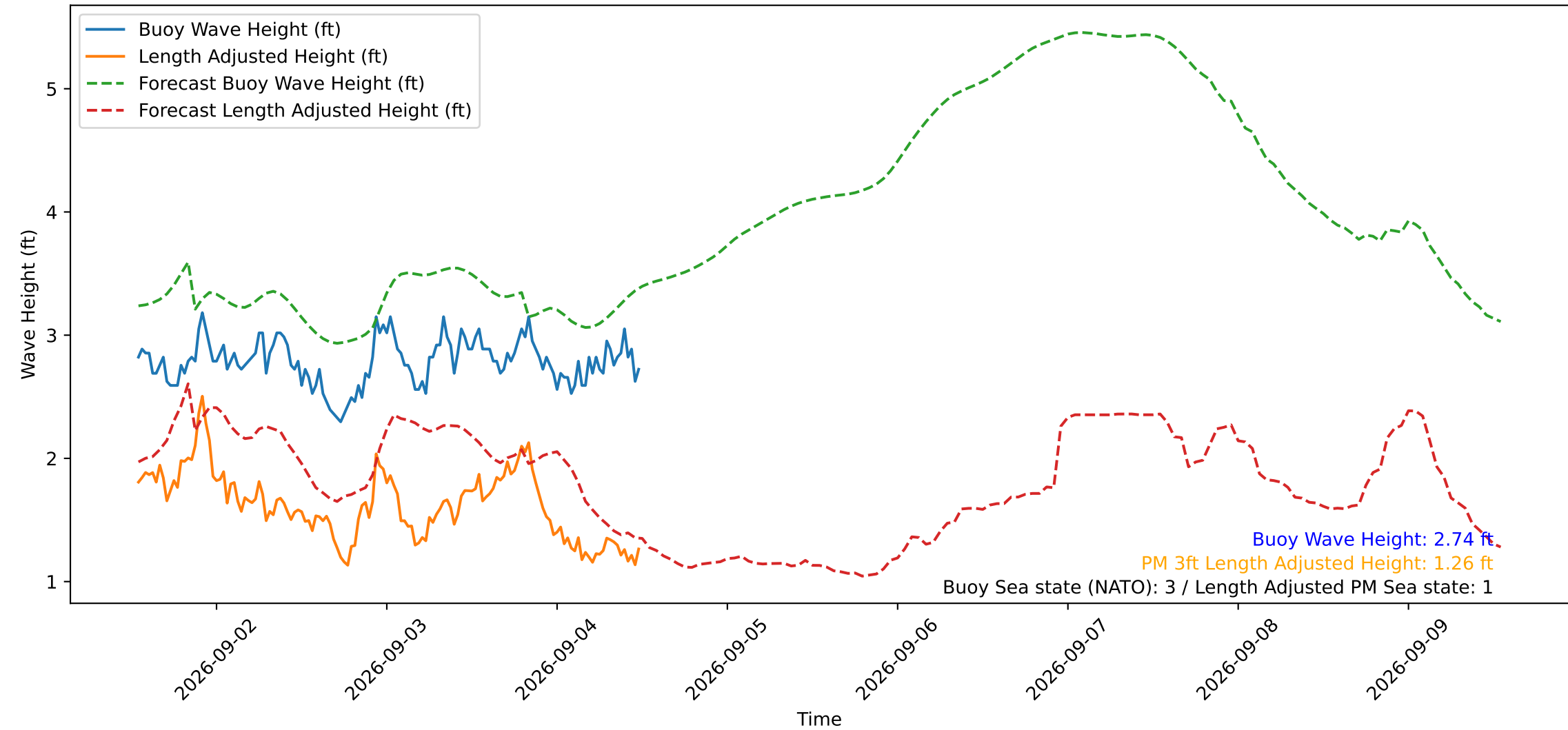
Wave Heights over Time for Red Beach at 2026-09-04 12:30:49
