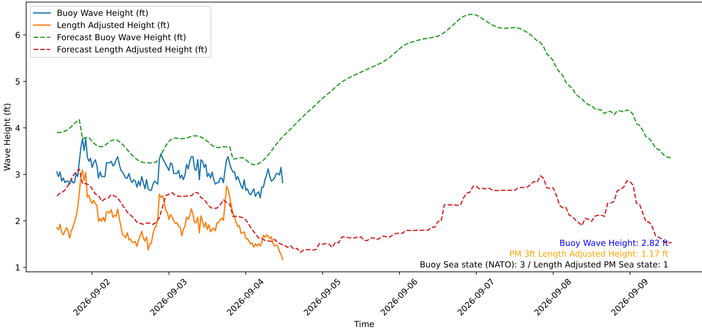
Wave Heights over Time for Green Beach at 2026-09-04 12:31:12
