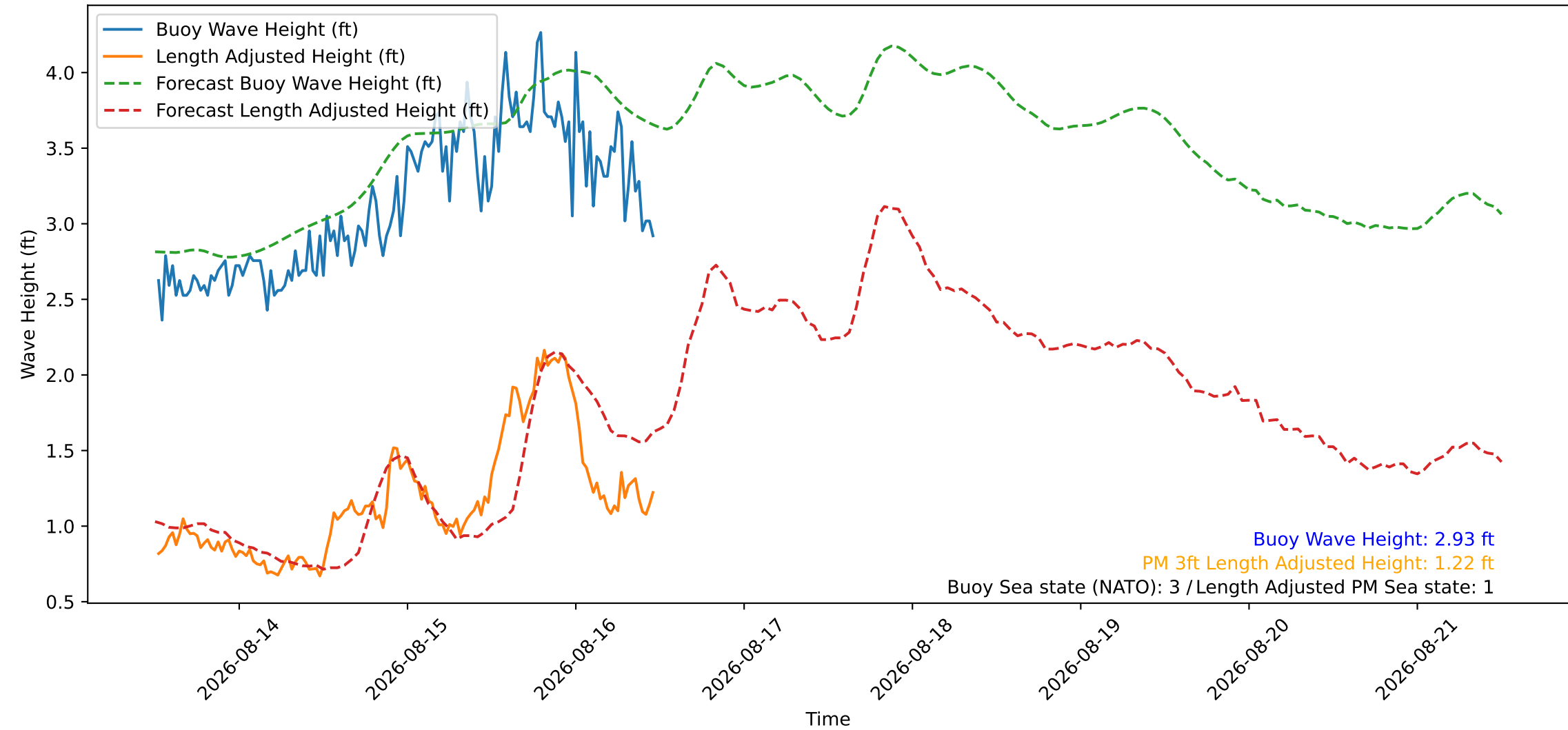
Wave Heights over Time for Green Beach at 2026-08-16 12:01:08
