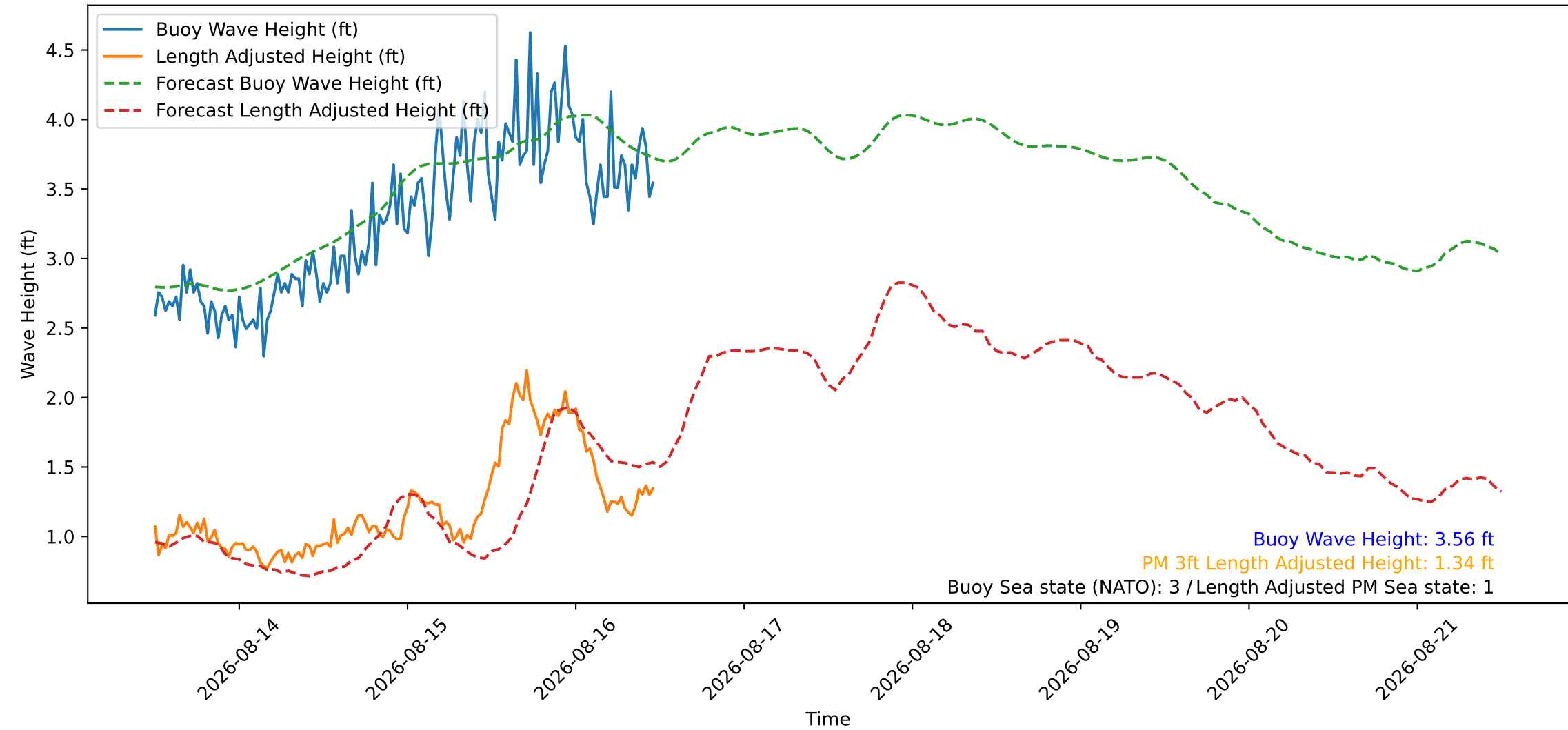
Wave Heights over Time for Oceanside Harbor at 2026-08-16 12:00:27
