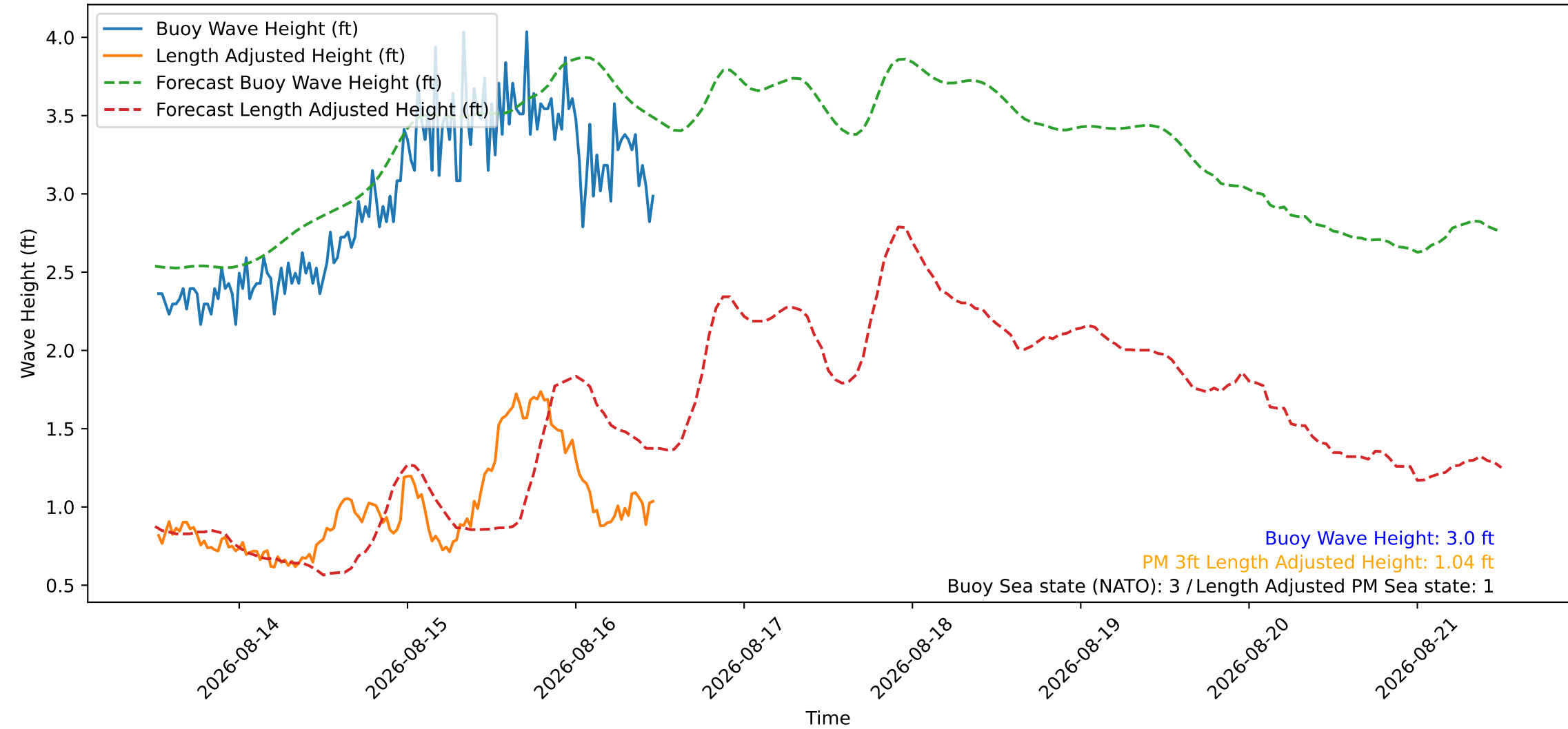
Wave Heights over Time for Red Beach at 2026-08-16 12:00:46
