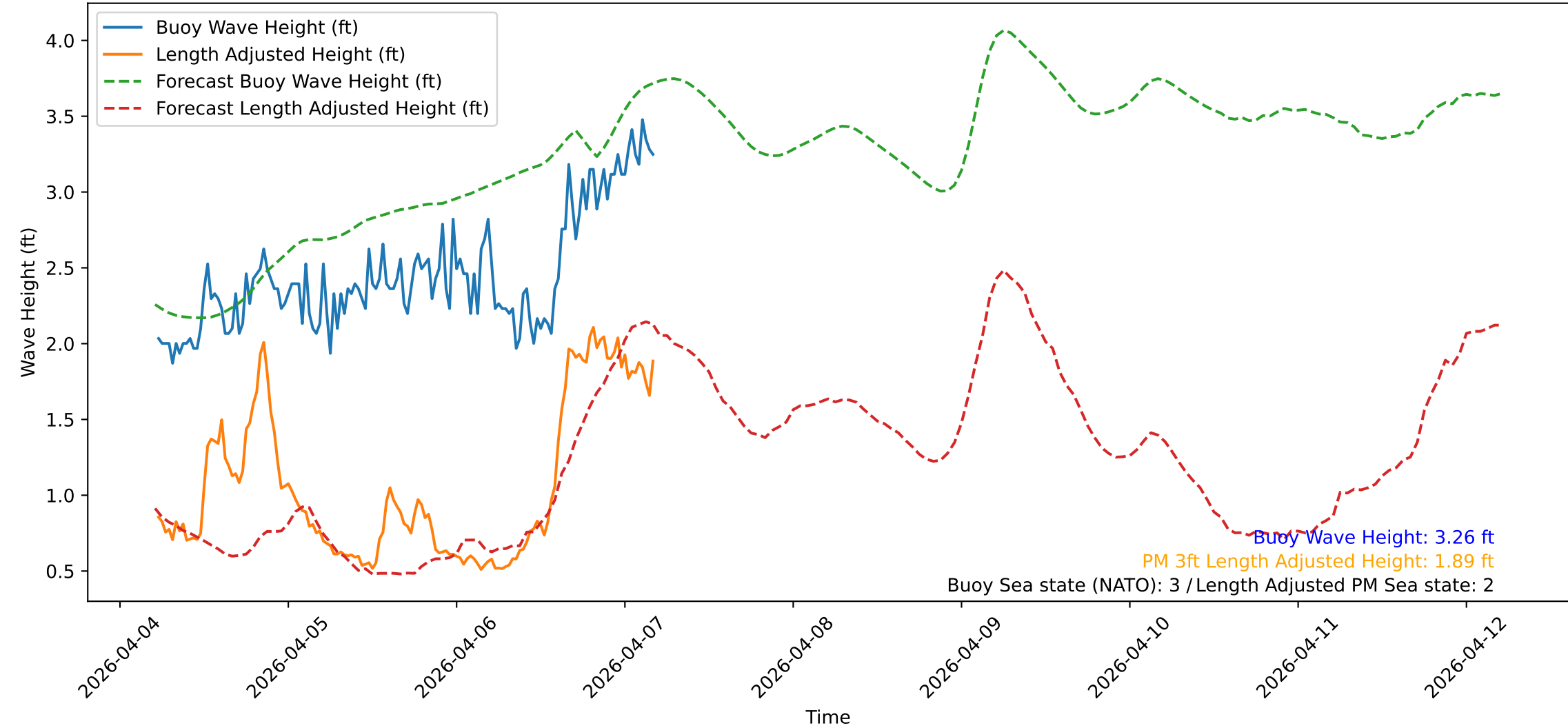
Wave Heights over Time for Red Beach at 2026-04-07 05:10:47
