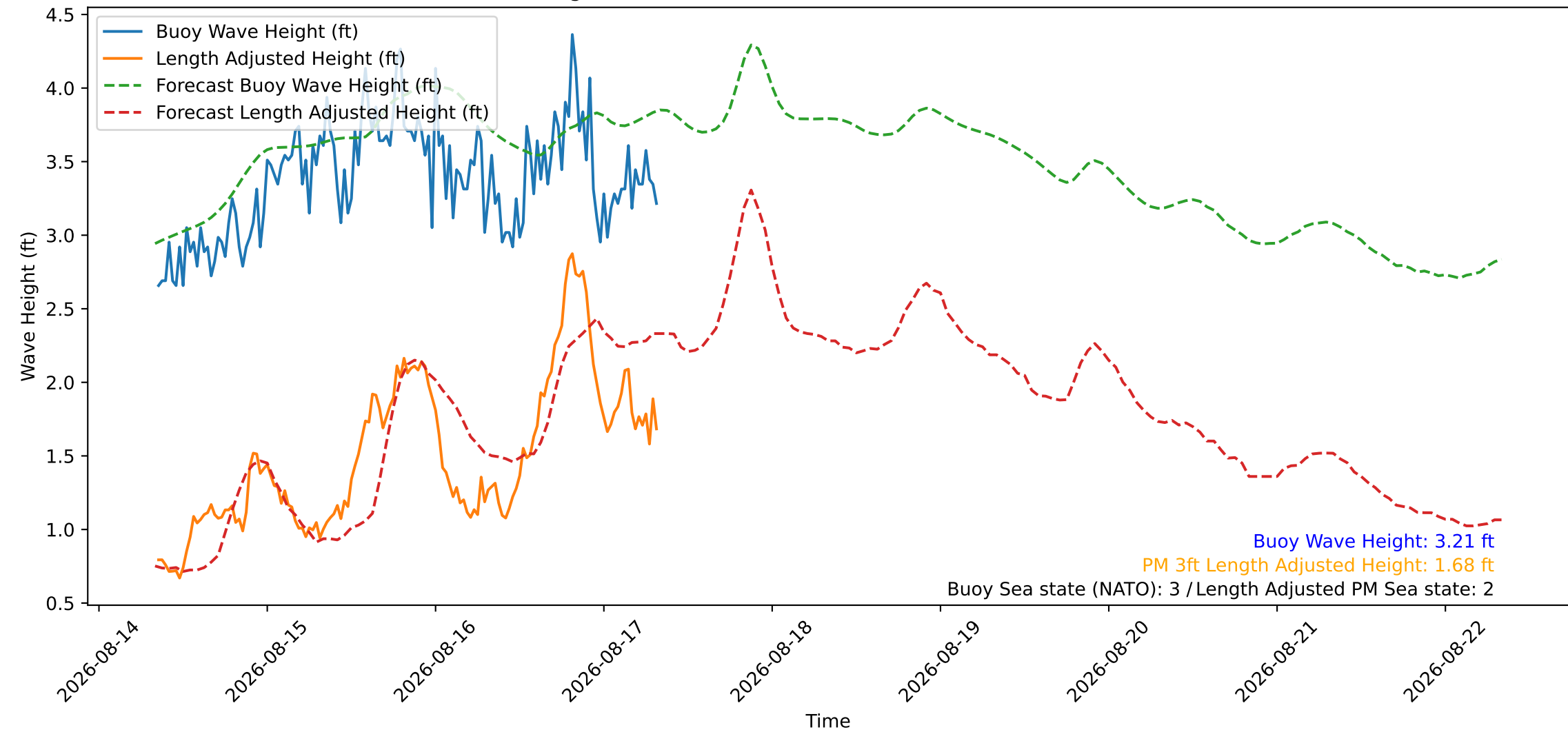
Wave Heights over Time for Green Beach at 2026-08-17 08:21:11
