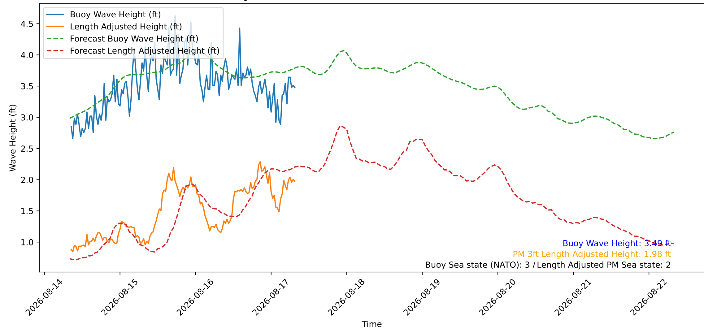
Wave Heights over Time for Oceanside Harbor at 2026-08-17 08:20:26
