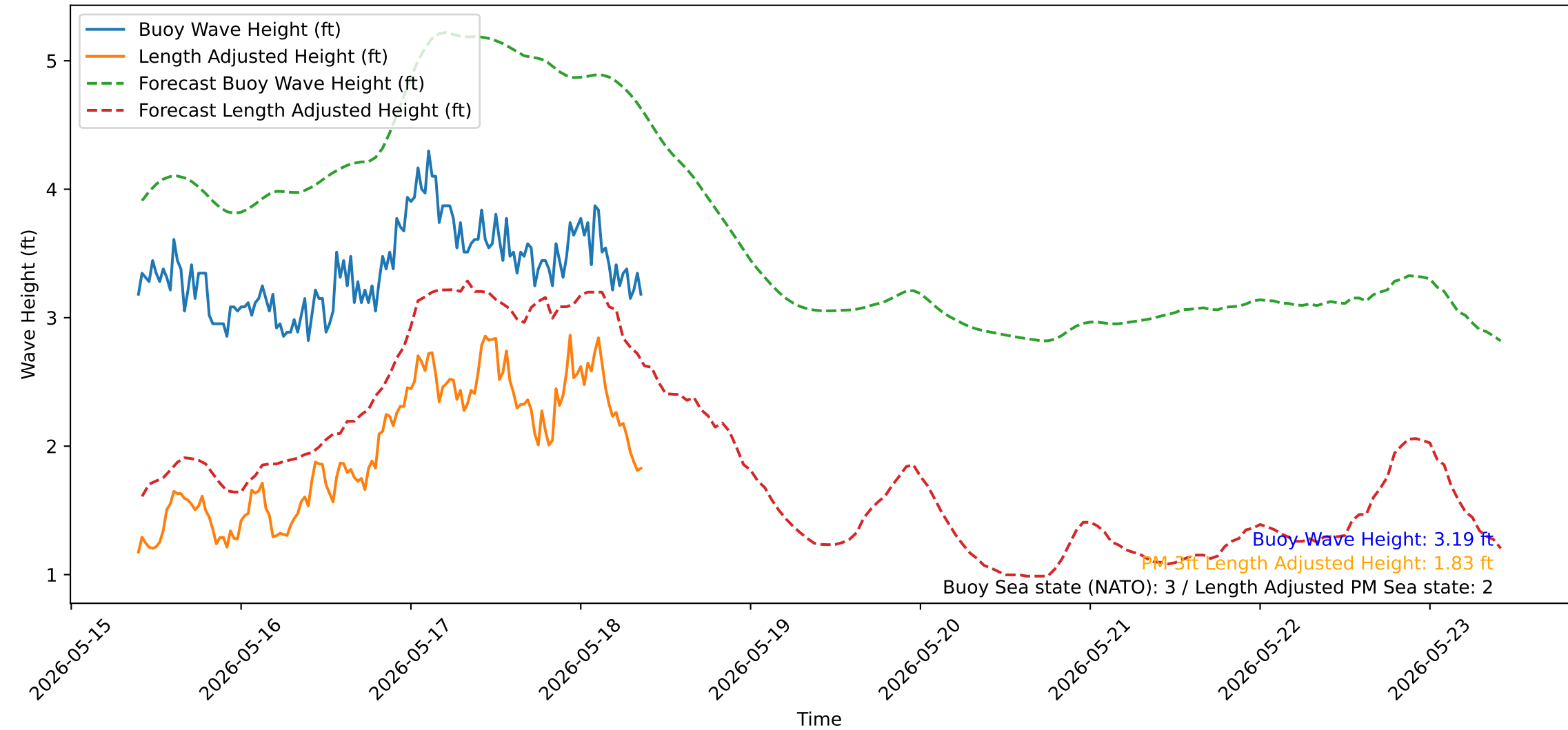
Wave Heights over Time for Oceanside Harbor at 2026-05-18 09:30:31
