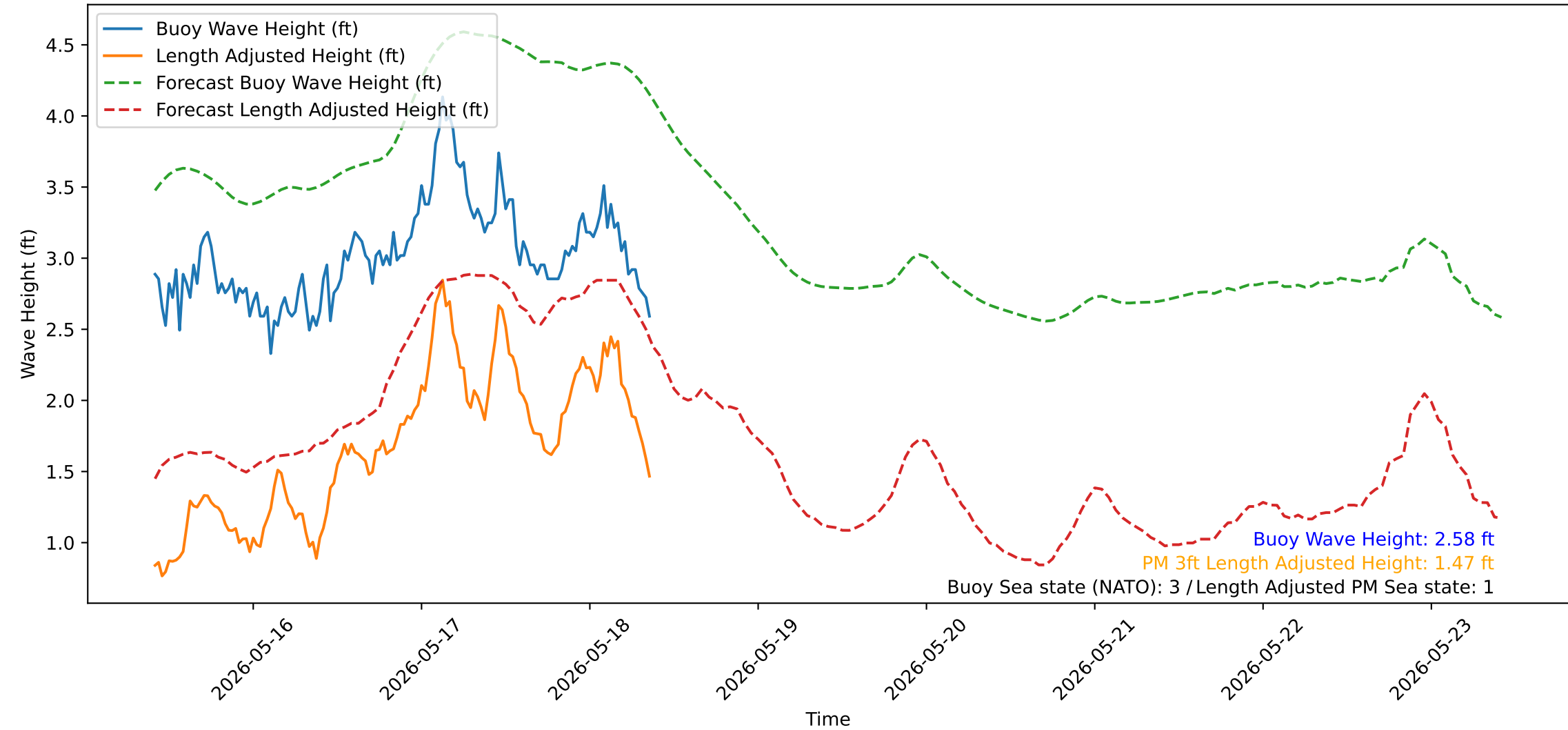
Wave Heights over Time for Red Beach at 2026-05-18 09:30:51
