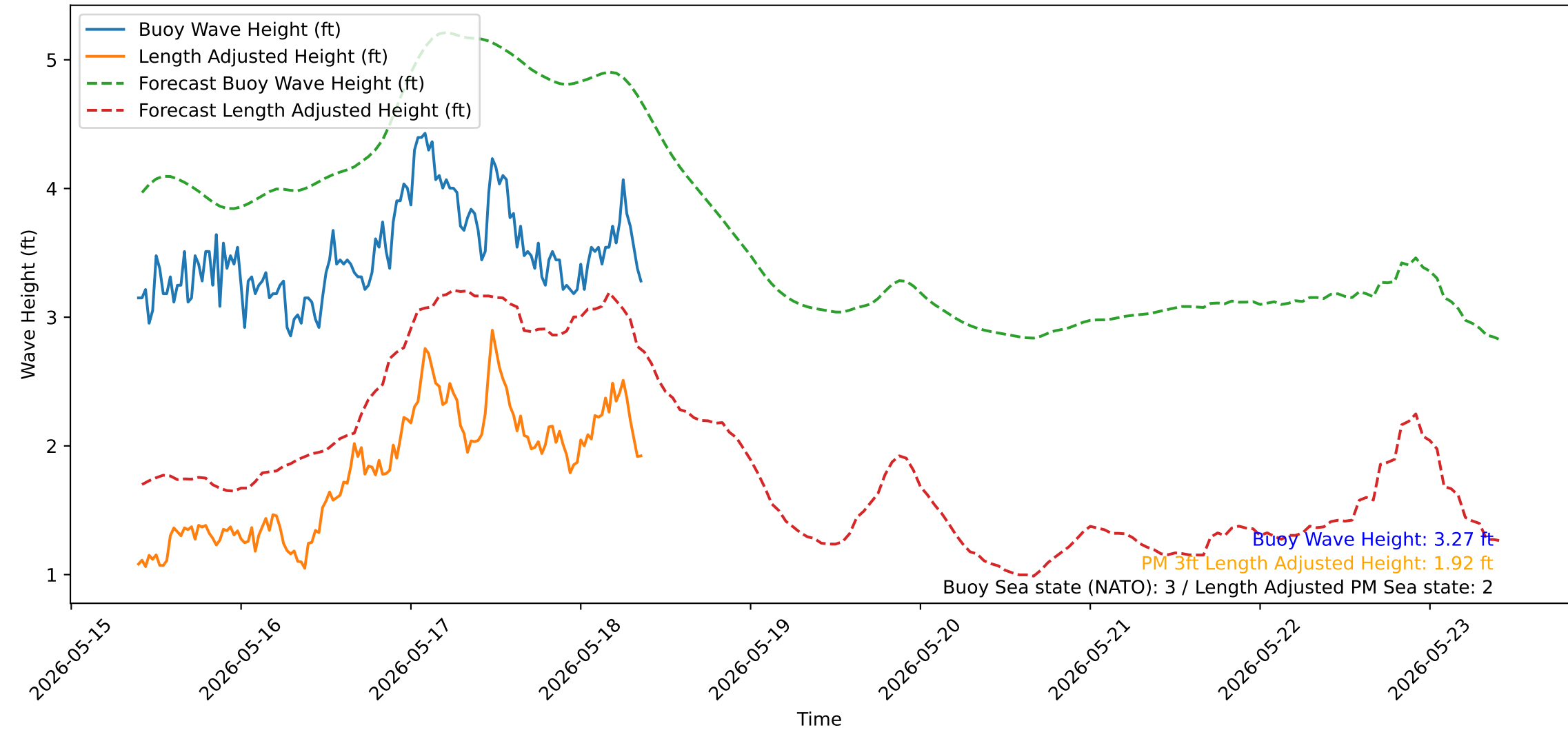
Wave Heights over Time for Green Beach at 2026-05-18 09:31:13
