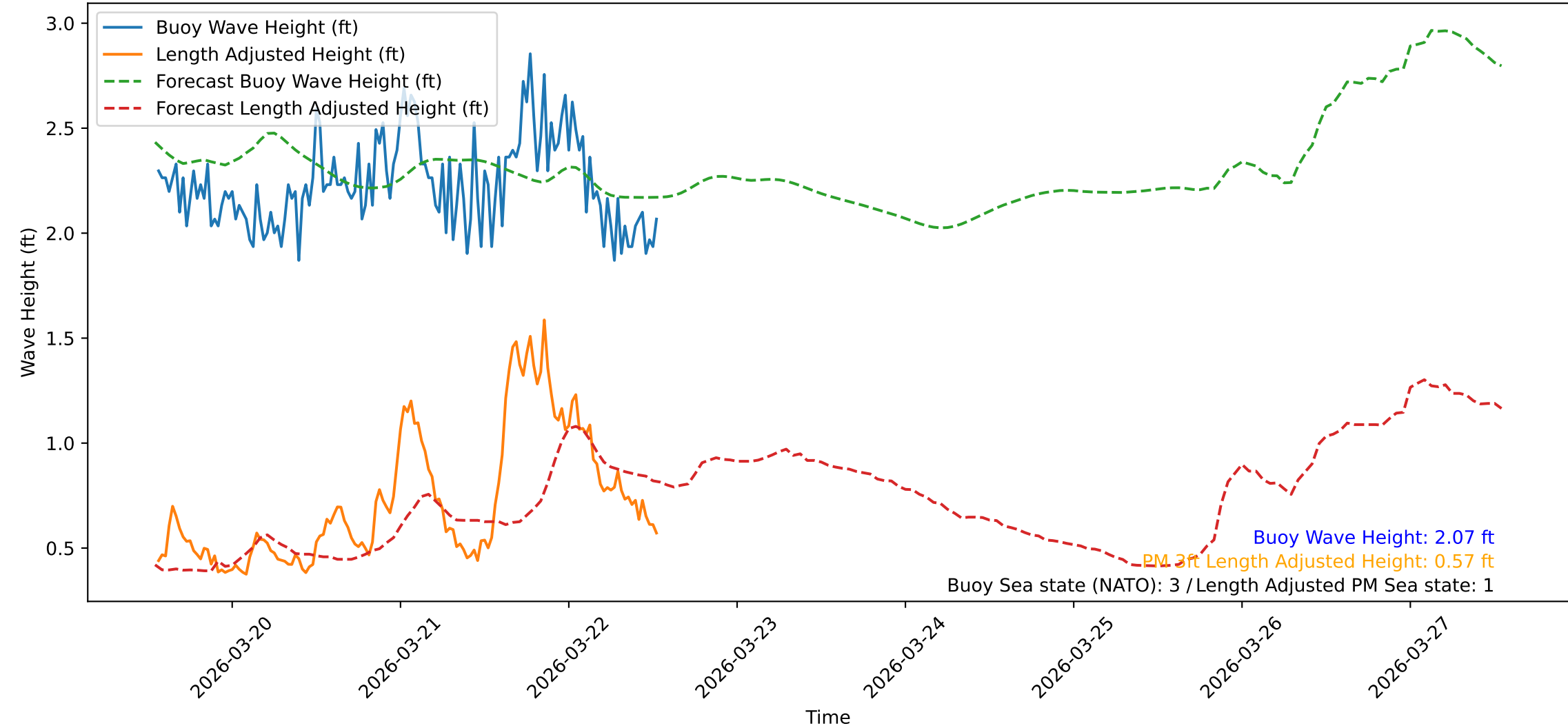
Wave Heights over Time for Red Beach at 2026-03-22 13:20:47
