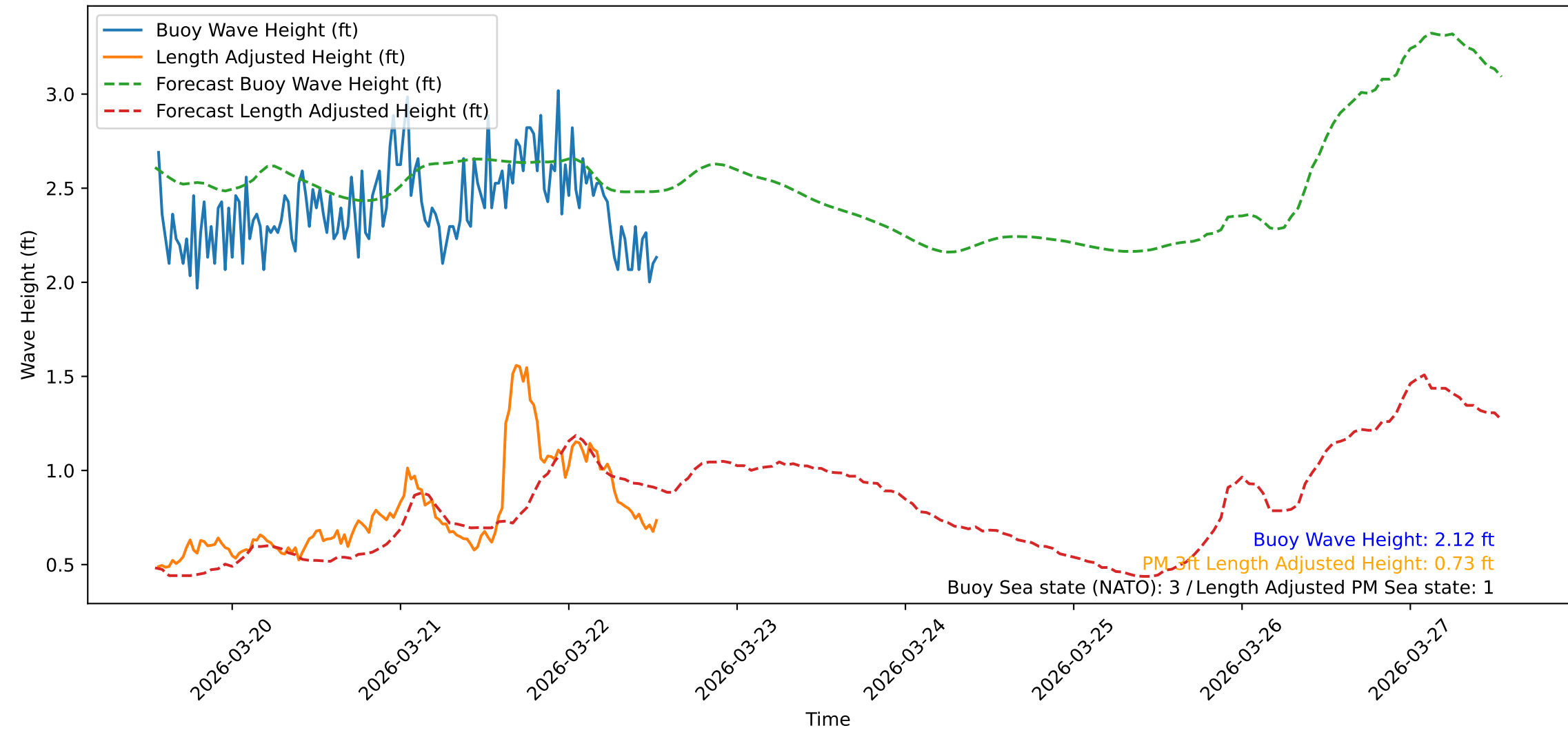
Wave Heights over Time for Oceanside Harbor at 2026-03-22 13:20:31
